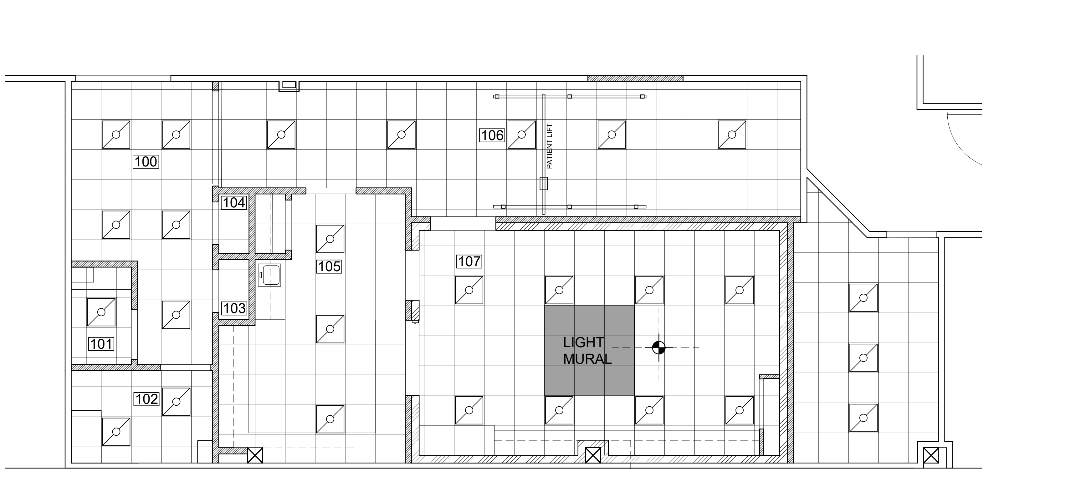
1 REFLECTED CEILING PLAN SCALE: 1/4" = 1'-0"
