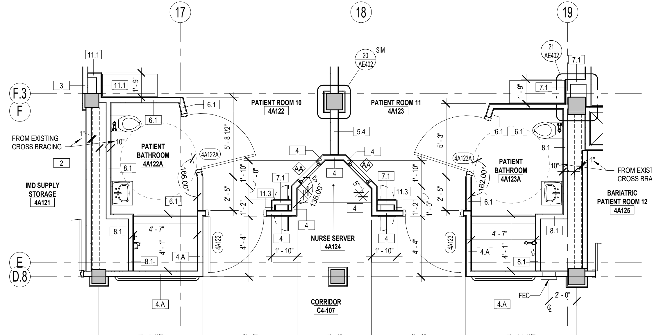
5 ENLARGED DIMENSION PLAN - 4A122A/4A123A AE108.2 1/4" = 1'-0"
