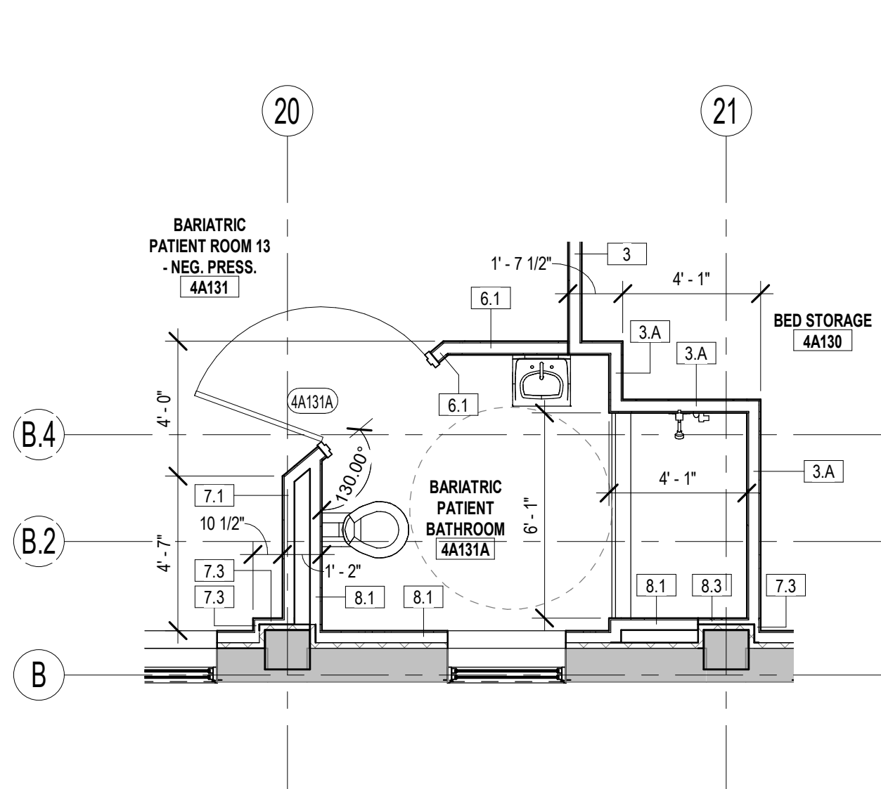
7 ENLARGED DIMENSION PLAN - 4A131A AE108.2 1/4" = 1'-0"
