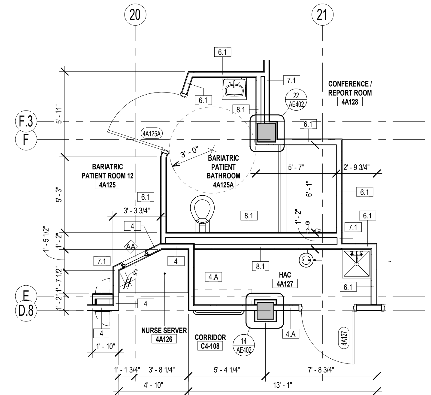
6 ENLARGED DIMENSION PLAN - 4A125A AE108.2 1/4" = 1'-0"
