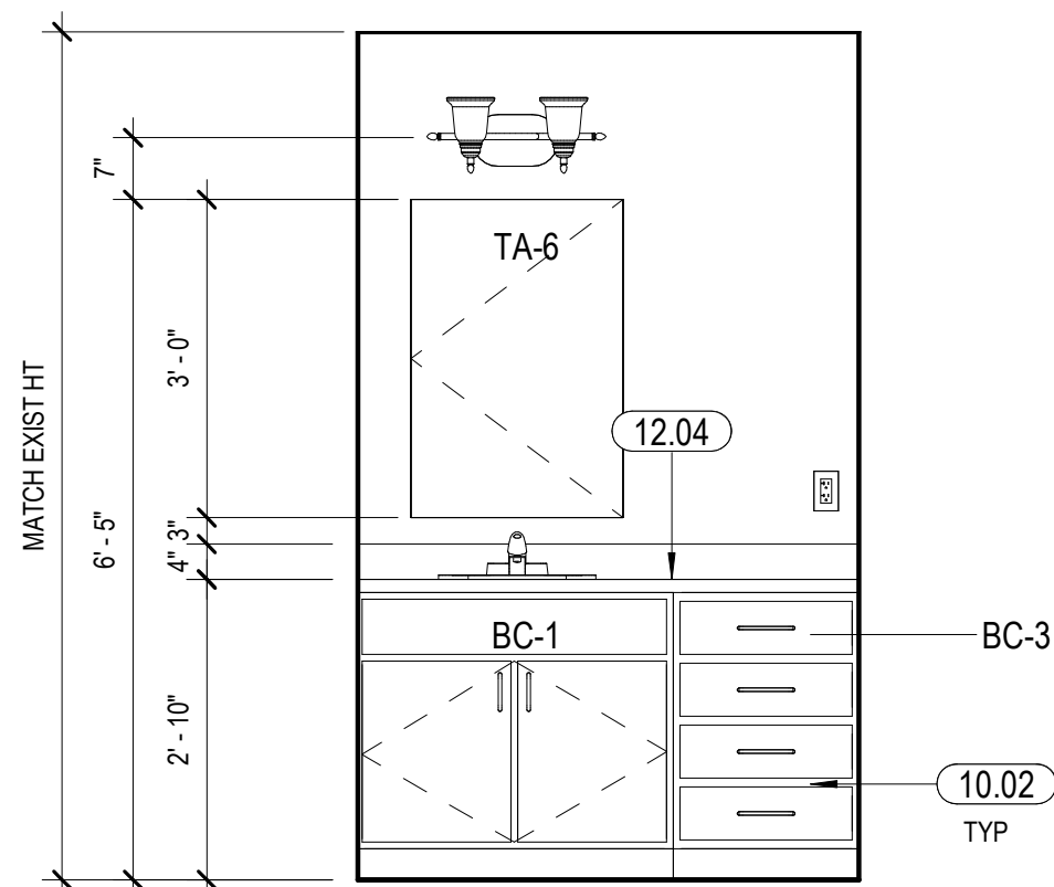
(E5) BEDROOM CASEWORK - INT EL 2 1/2" = 1'-0"
