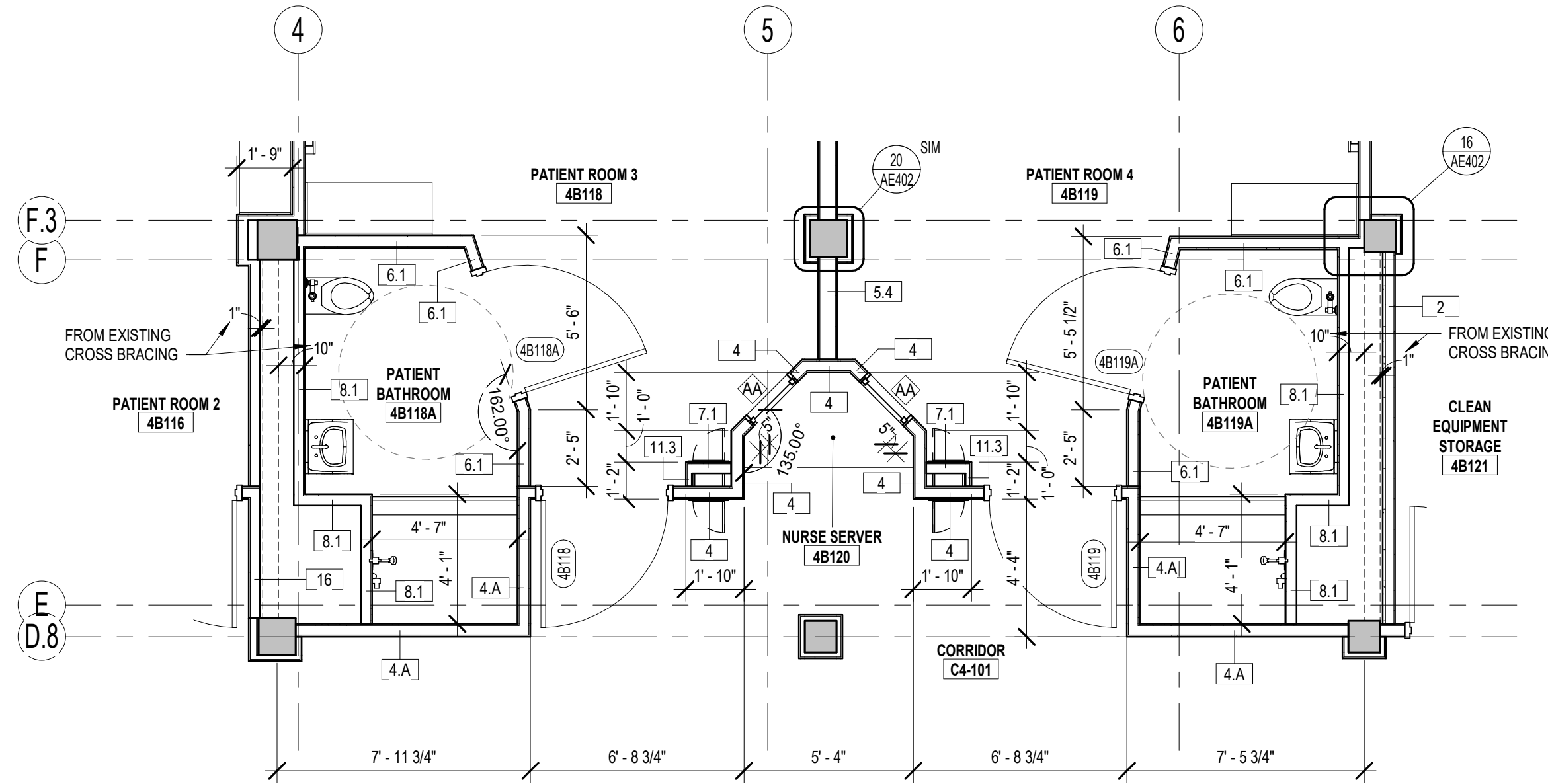
2 ENLARGED DIMENSION PLAN - 4B118A/4B119A AE108.2 1/4" = 1'-0"
