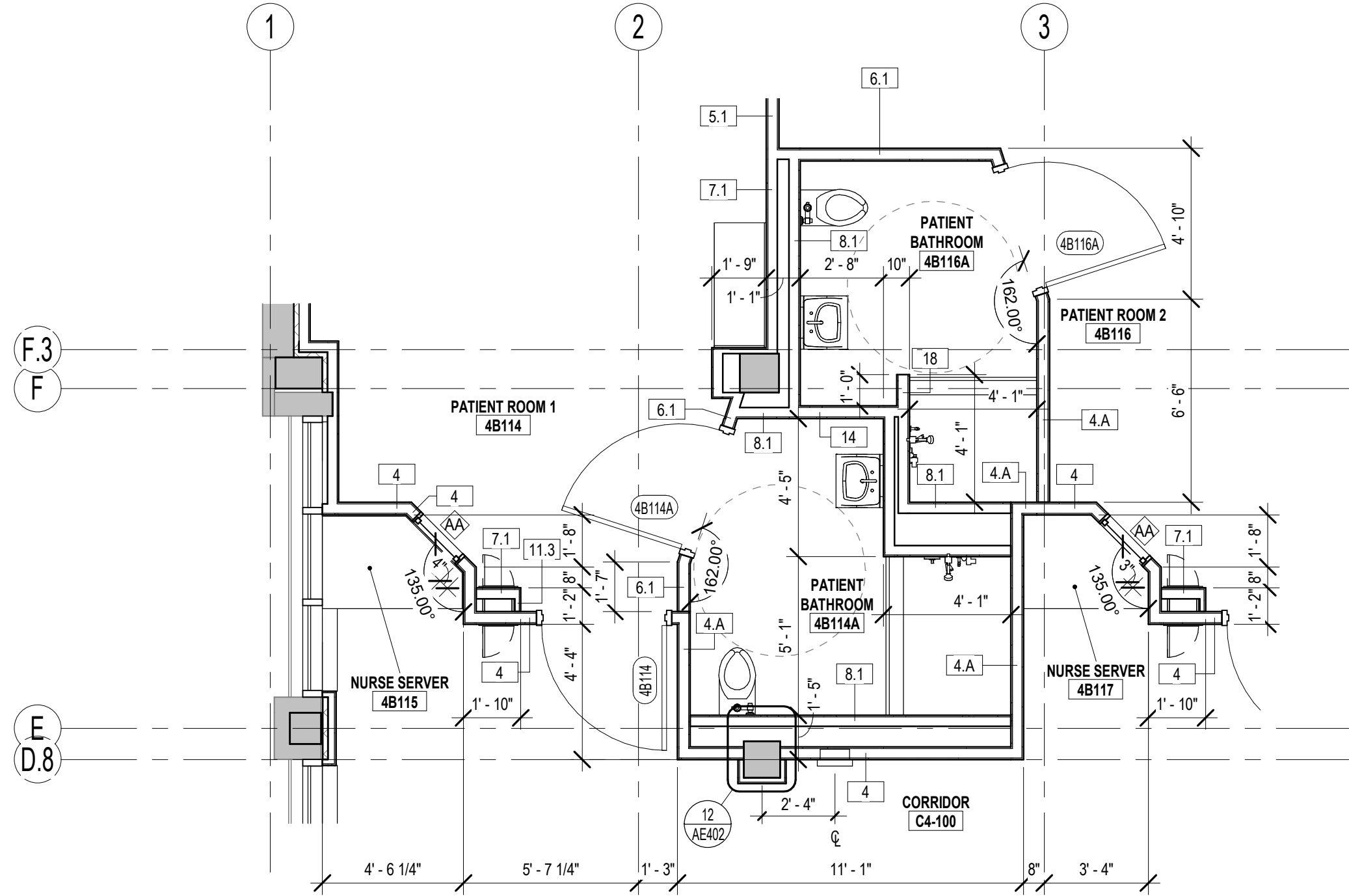
1 ENLARGED DIMENSION PLAN - 4B114A/4B116A AE108.2 1/4" = 1'-0"
