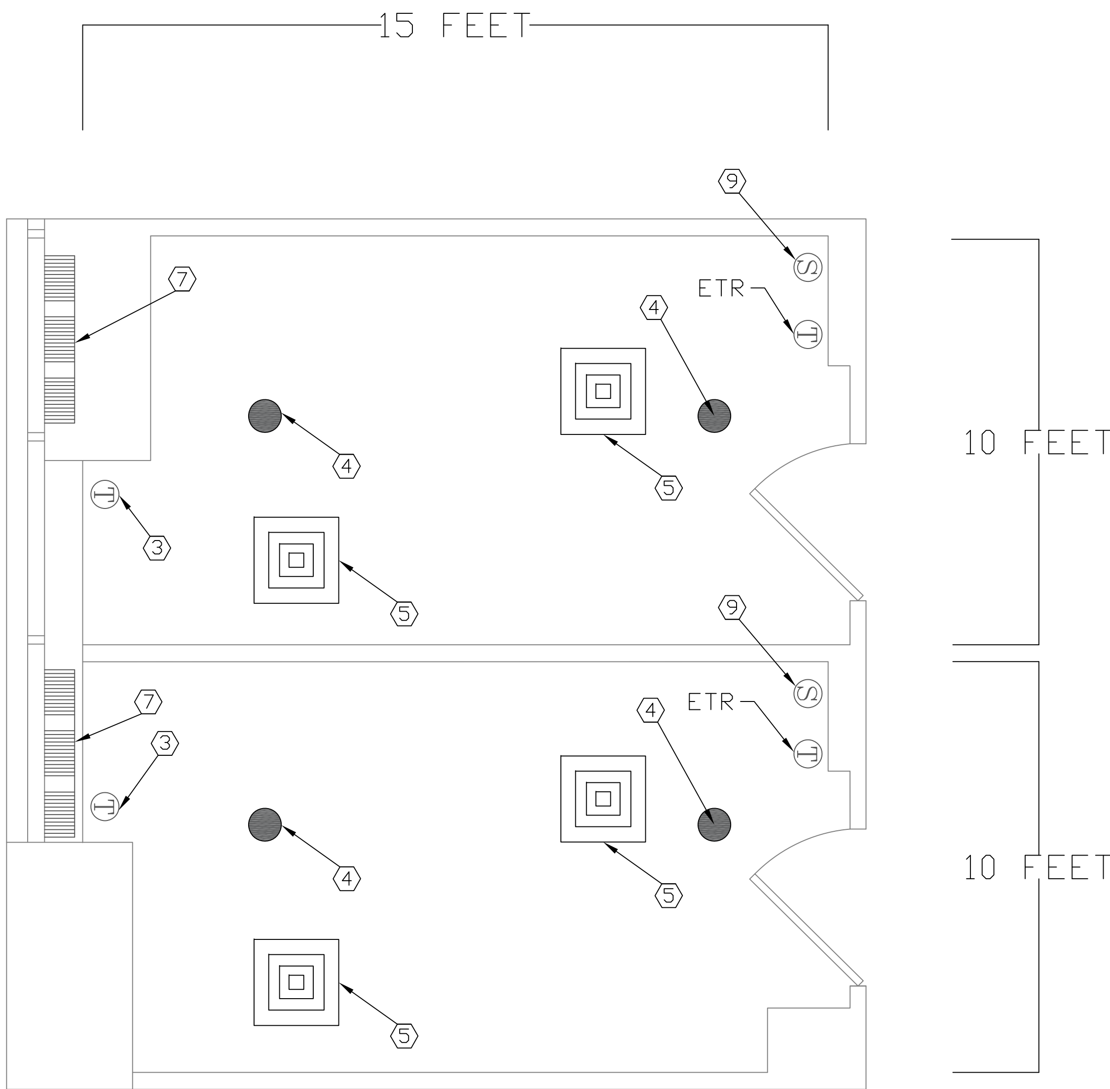
PROPOSED HVAC FOR ROOM 136-B, 137-B
