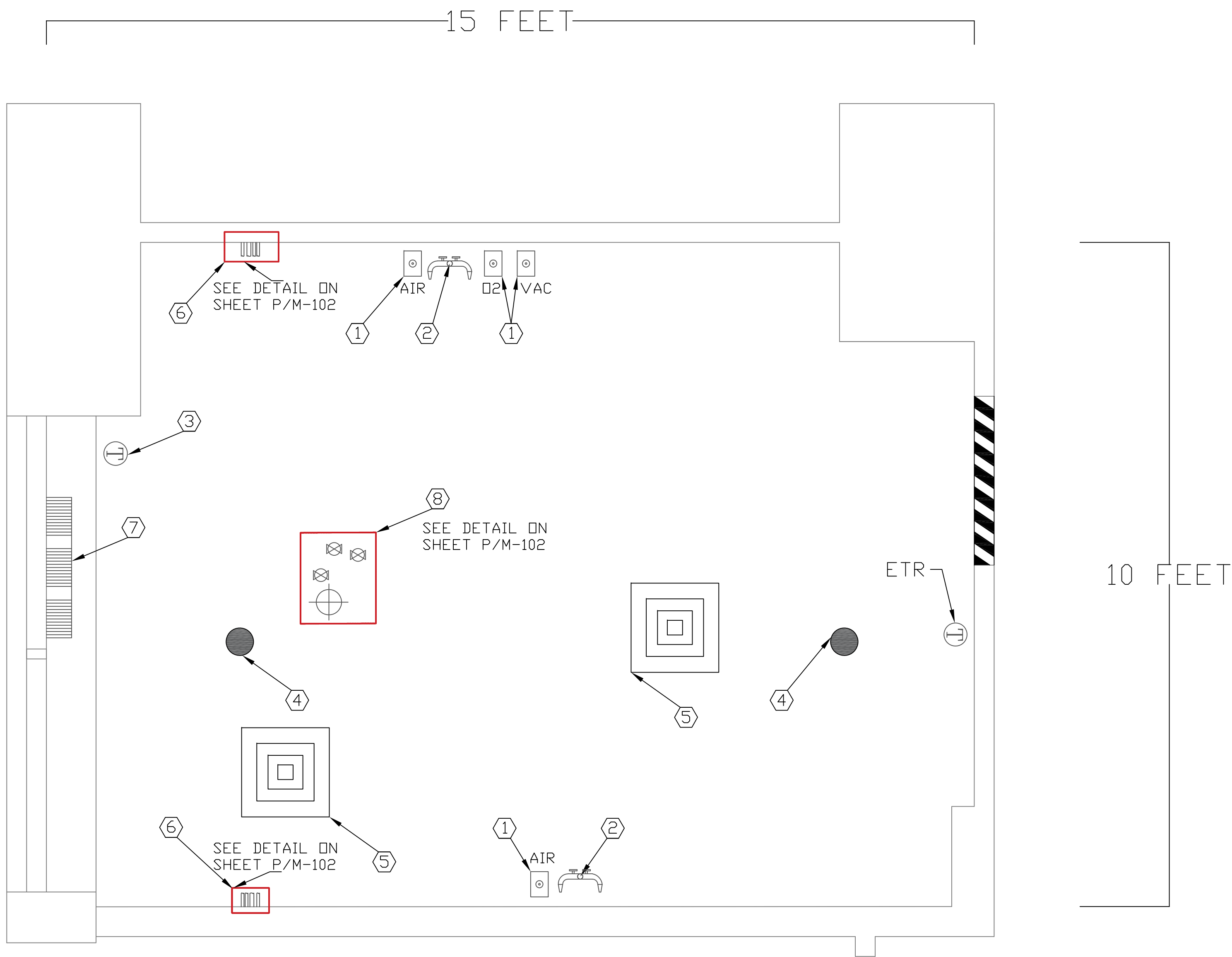
PROPOSED MECHANICAL/PLUMBING PLAN (N.T.S.)- 116-B-PHASE ONE
