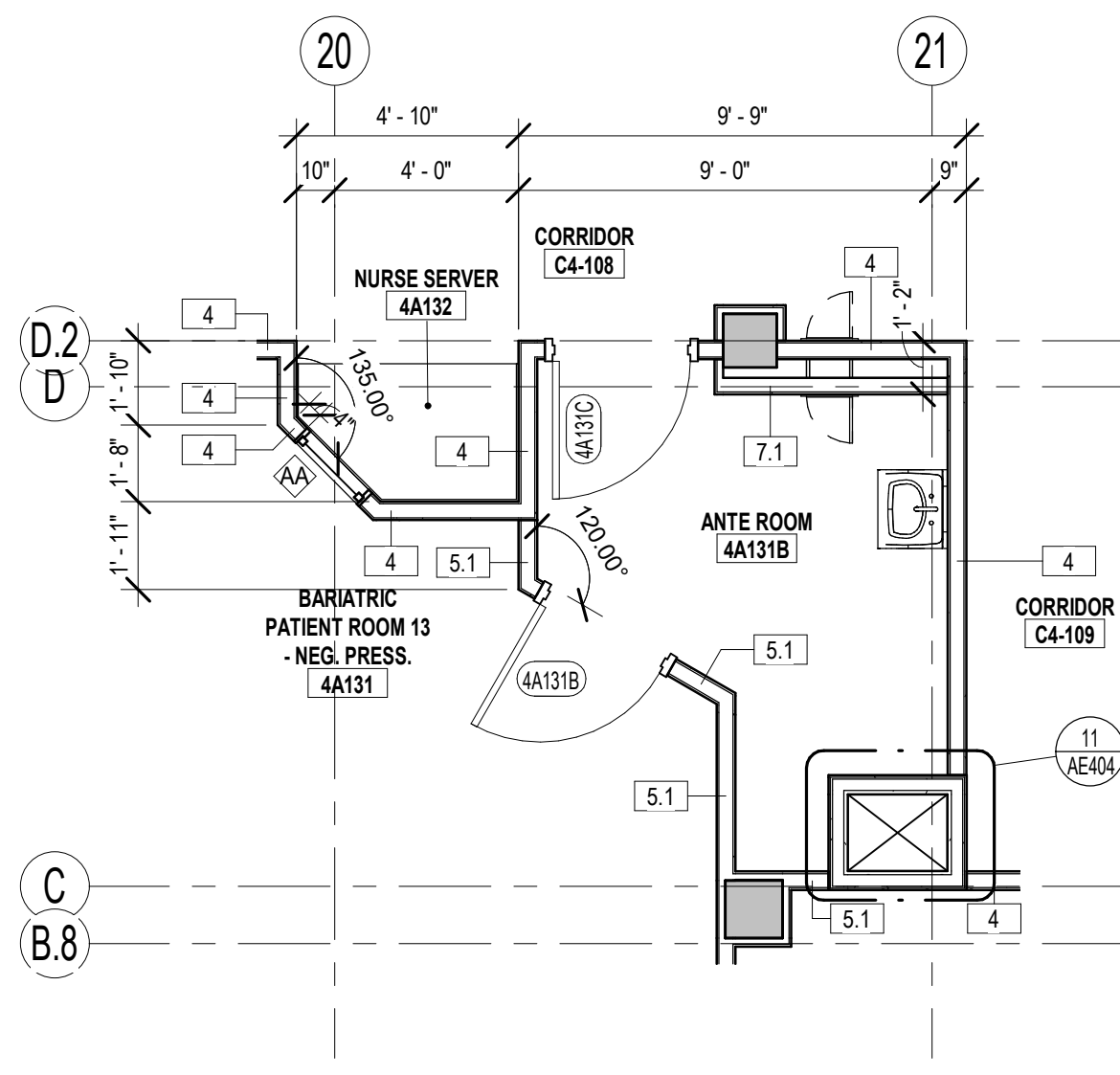
8 ENLARGED DIMENSION PLAN - 4A131B AE108.2 1/4" = 1'-0"
