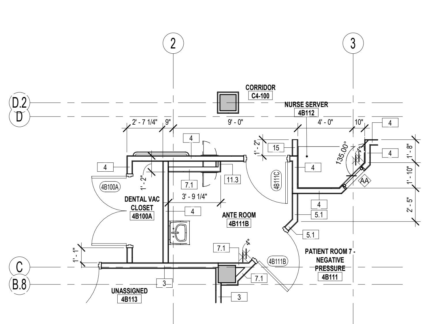
10 ENLARGED DIMENSION PLAN - 4B111B AE108.2 1/4" = 1'-0"
