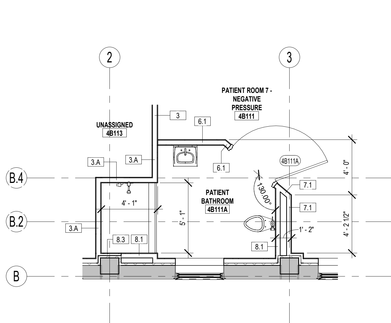
9 ENLARGED DIMENSION PLAN - 4B111A AE108.2 1/4" = 1'-0"
