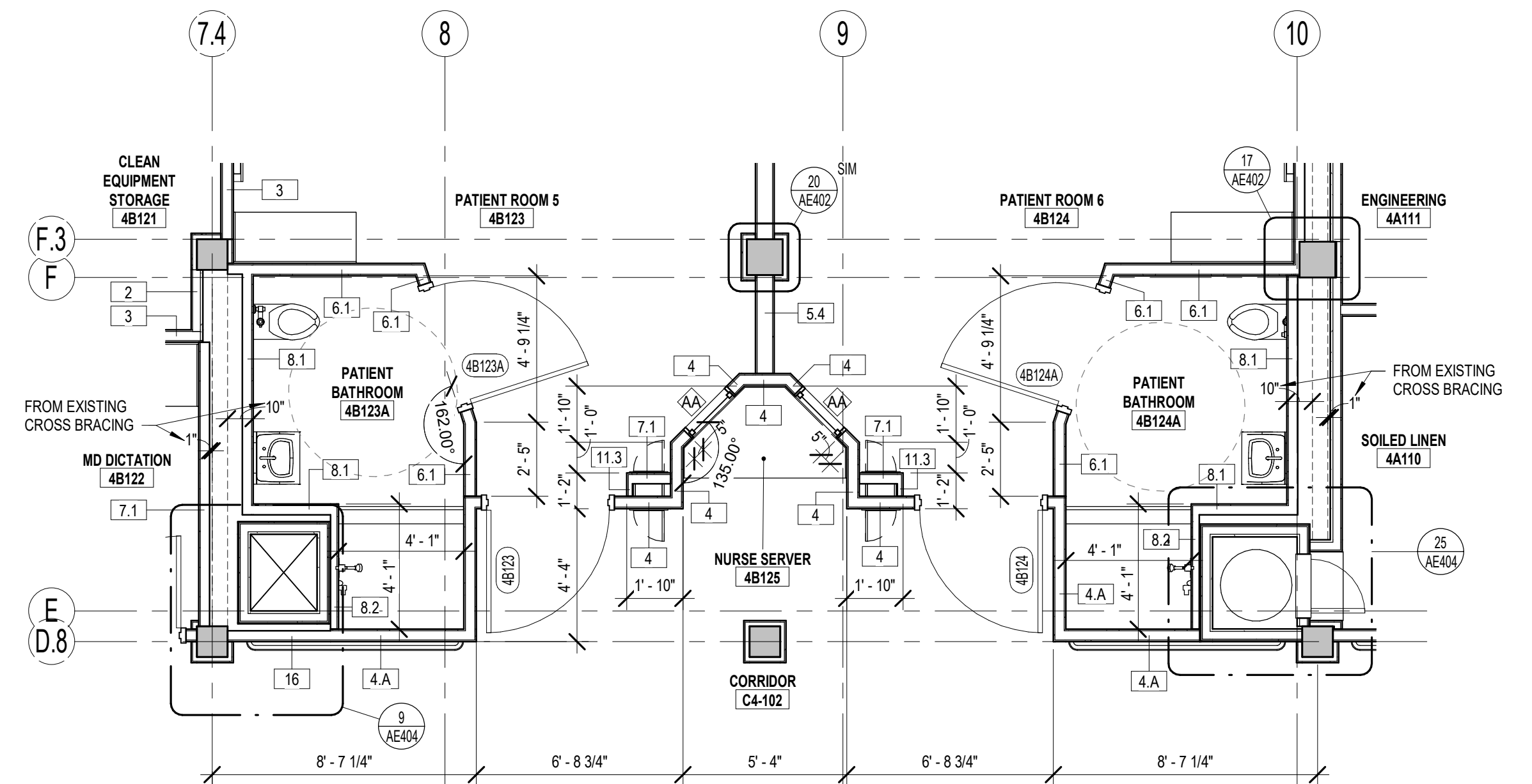
3 ENLARGED DIMENSION PLAN - 4B123A/4B124A AE108.2 1/4" = 1'-0"
