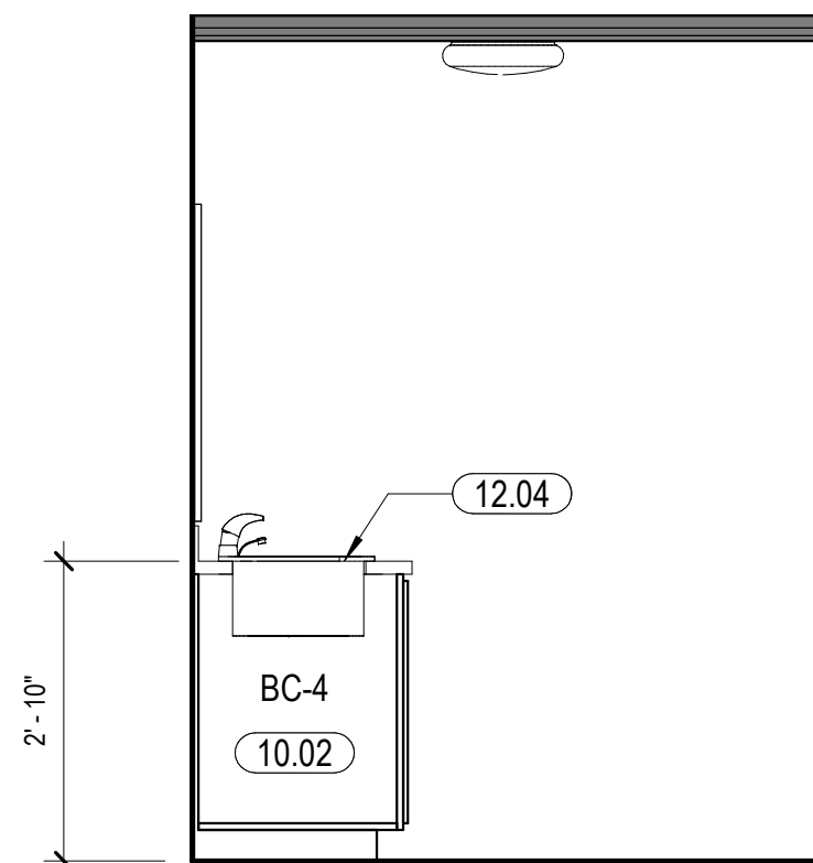
BATHROOM - RM 103 - INT EL 4 1/2" = 1'-0"
