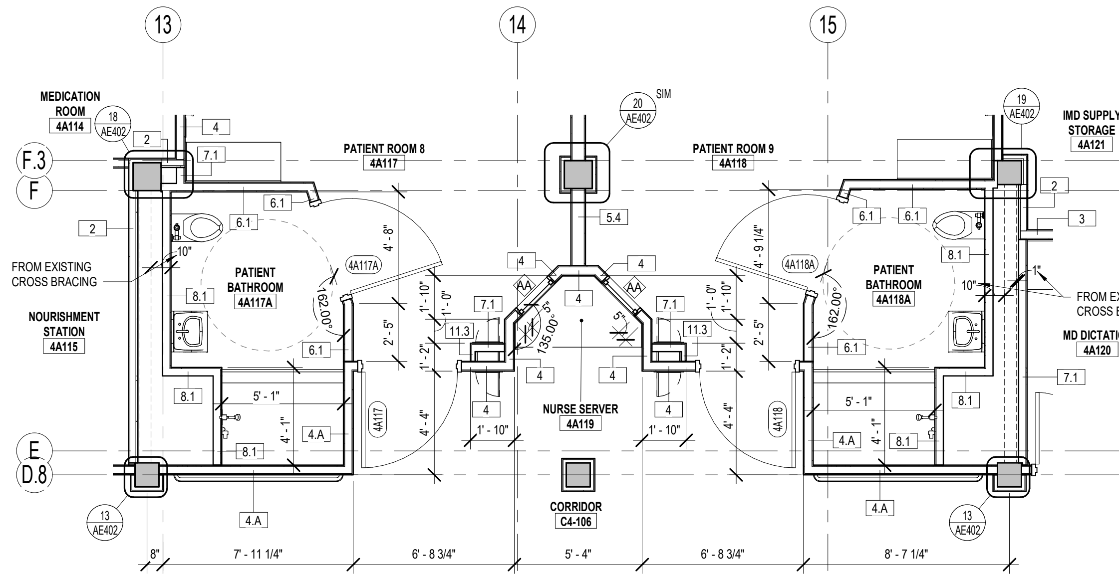
4 ENLARGED DIMENSION PLAN - 4A117A/4A118A AE108.2 1/4" = 1'-0"
