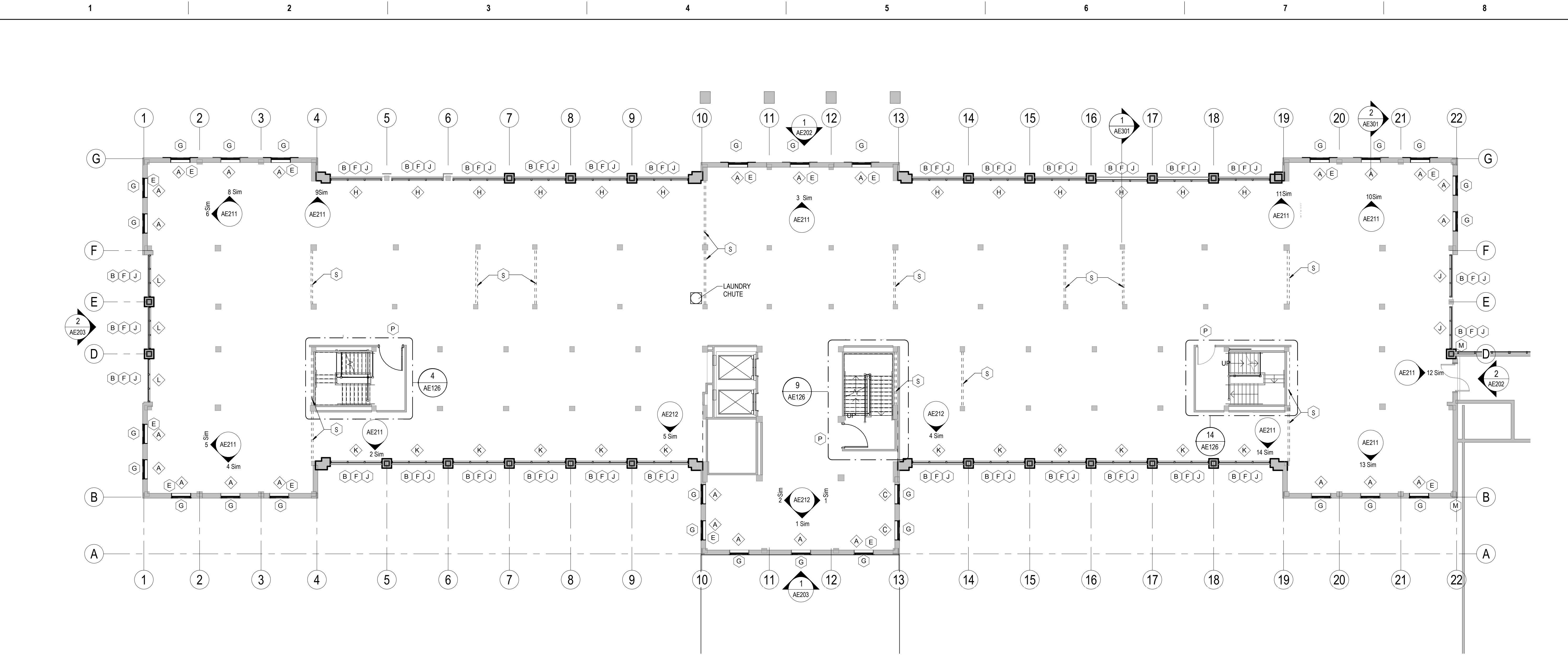
2 FOURTH FLOOR PLAN 3/32" = 1'-0"
