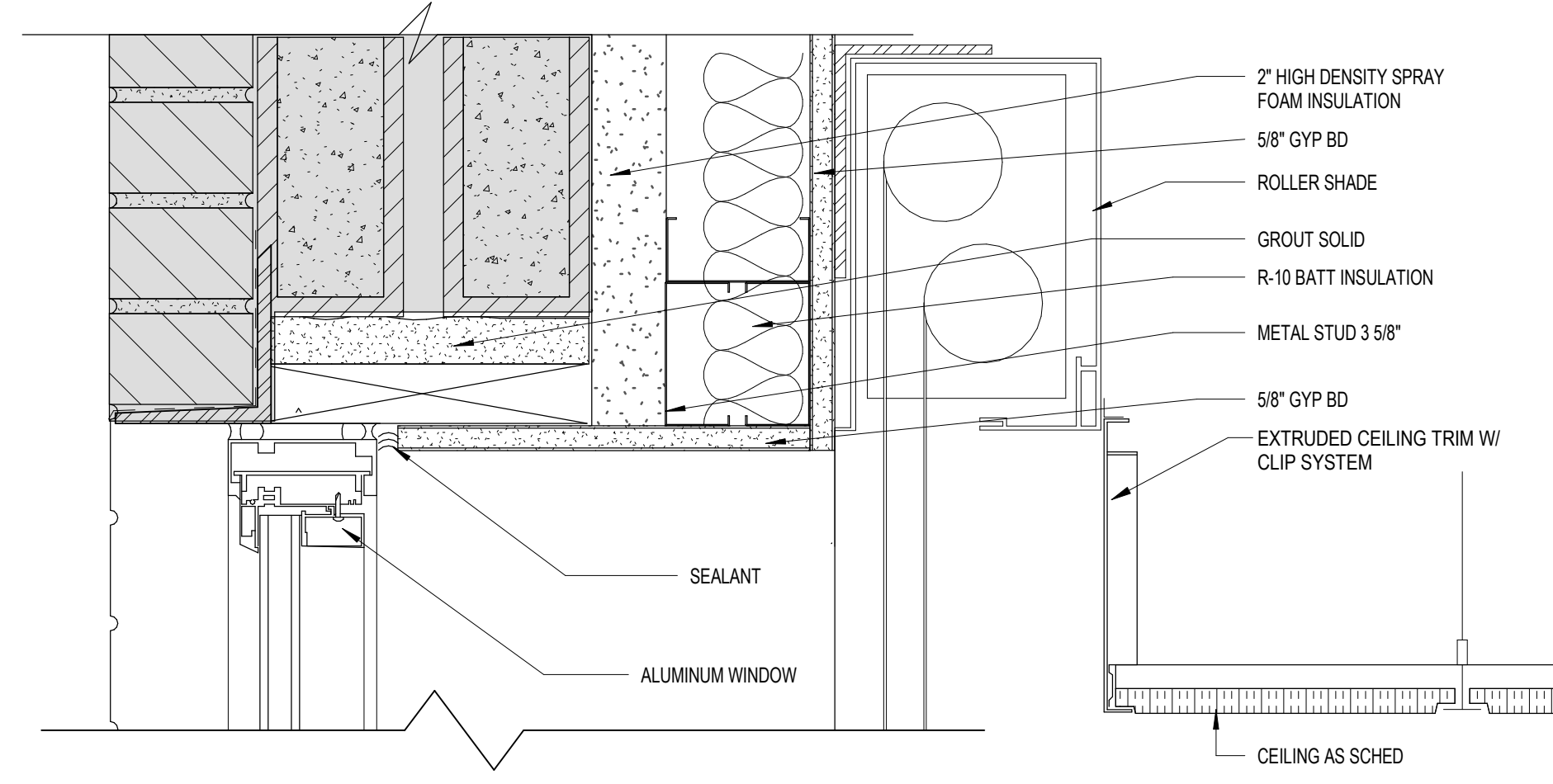
9 WINDOW HEAD AE514 3" = 1'-0"
