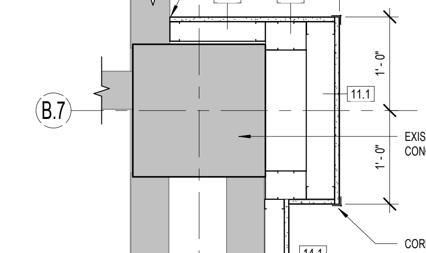
27 COLUMN PLAN DETAIL 1" = 1'-0"
