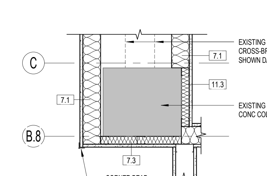
6 COLUMN PLAN DETAIL 1" = 1'-0"
