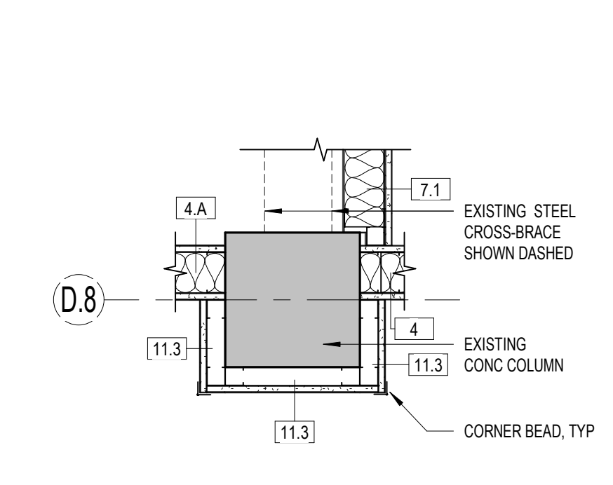
6 COLUMN PLAN DETAIL 1" = 1'-0"
