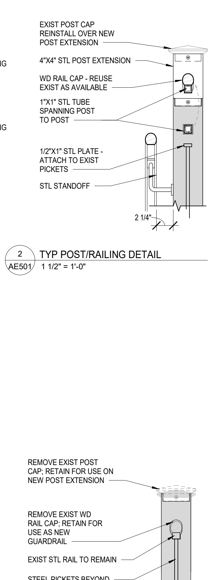
2 TYP POST/RAILING DETAIL AE501/ 1 1/2" = 1'-0"
