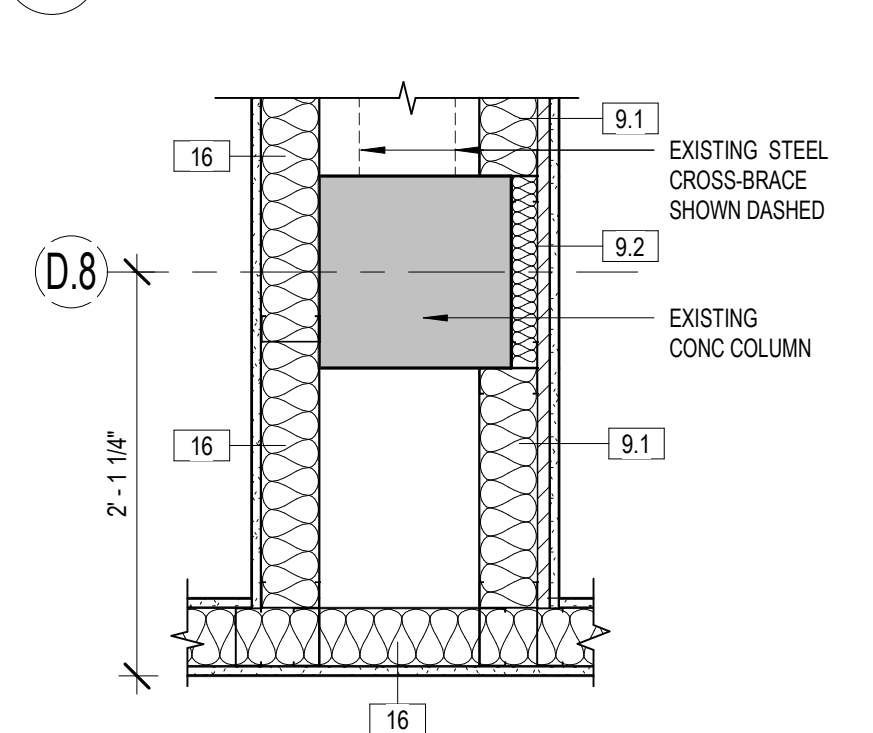
31 COLUMN PLAN DETAIL 1" = 1'-0"
