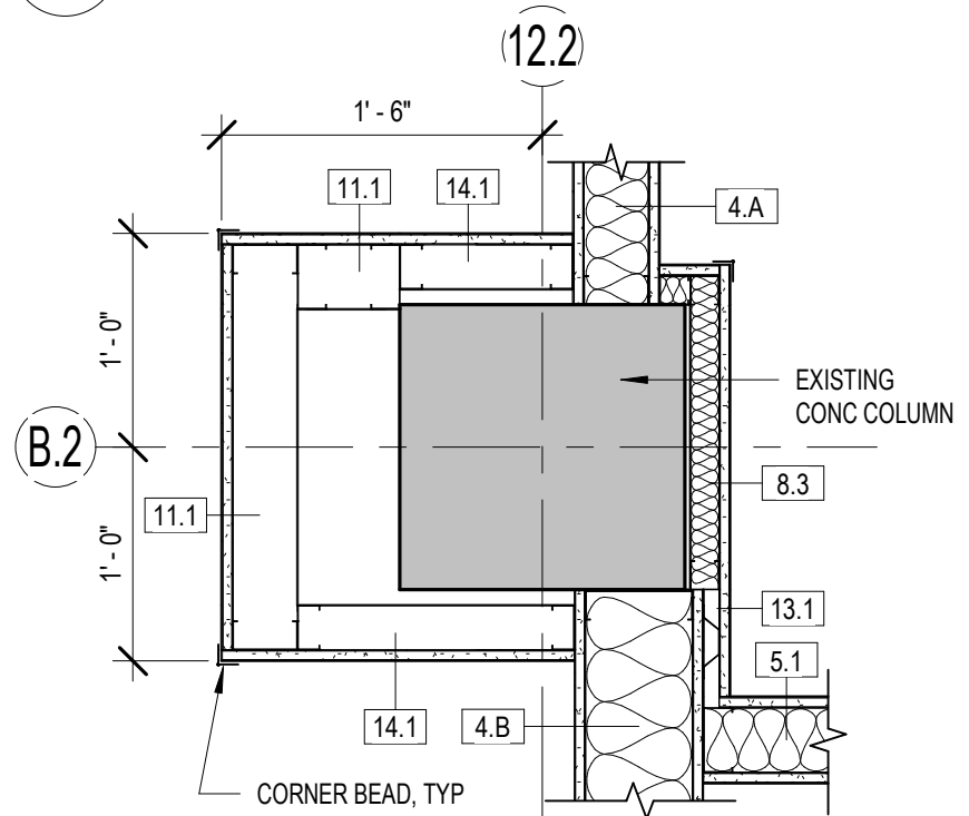
29 COLUMN PLAN DETAIL 1" = 1'-0"
