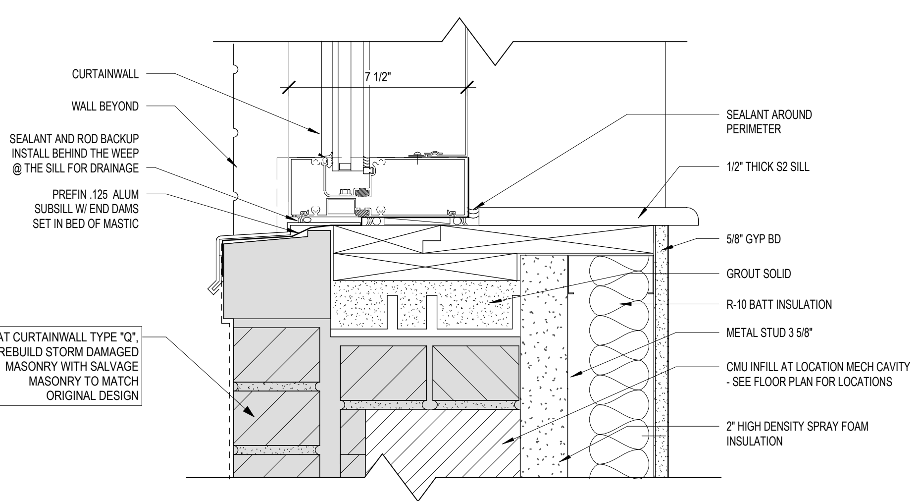
7 CURTAINWALL SILL DETAIL AE514 3" = 1'-0"
