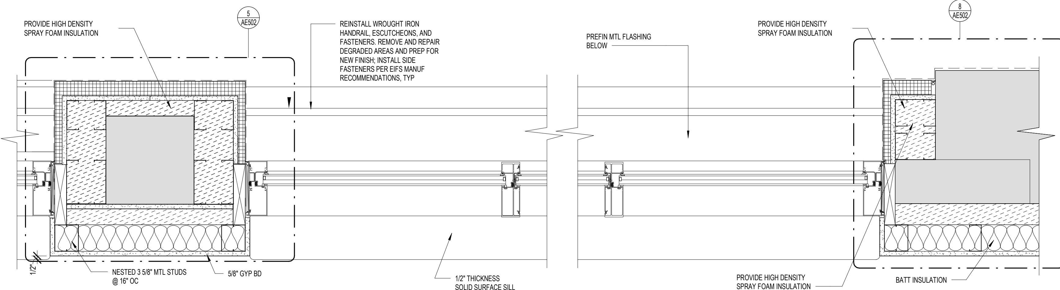
1 TYPICAL CURTAINWALL DETAIL - 3RD & 4TH FLOOR AE502 1 1/2" = 1'-0"
