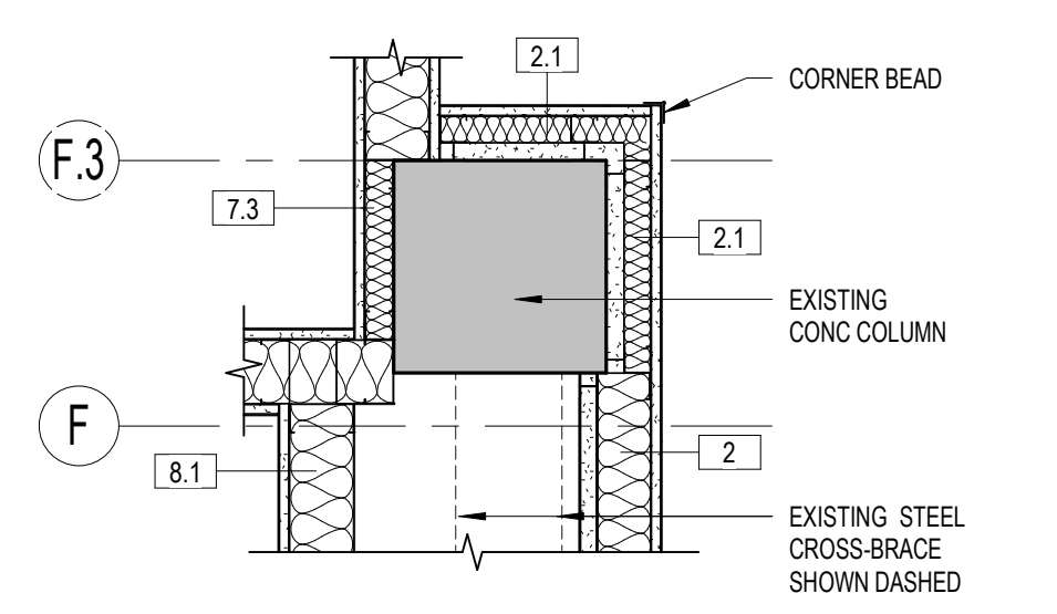
19 COLUMN PLAN DETAIL 1" = 1'-0"
