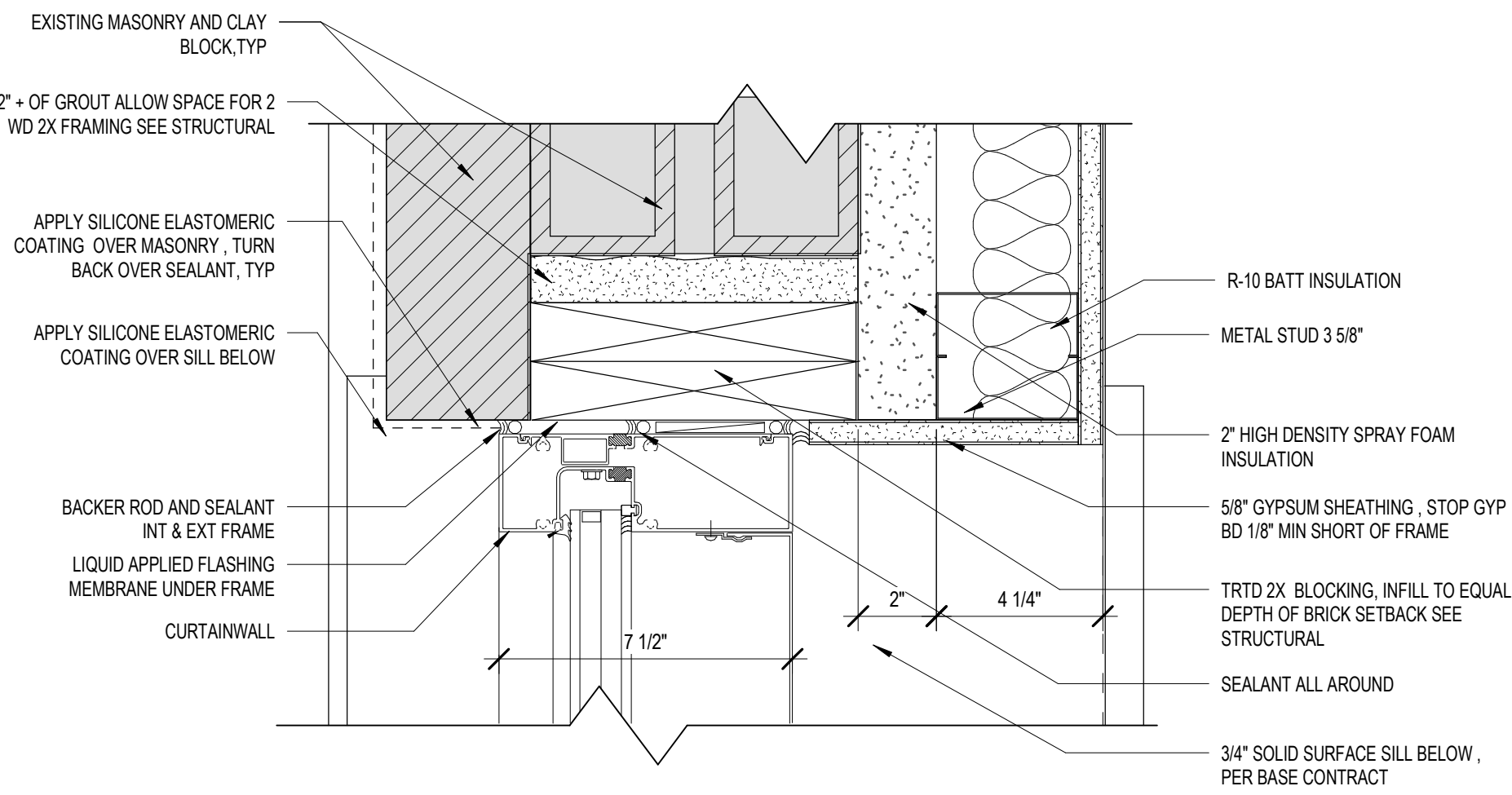
6 CURTAINWALL JAMB DETAIL AE514 3" = 1'-0"
