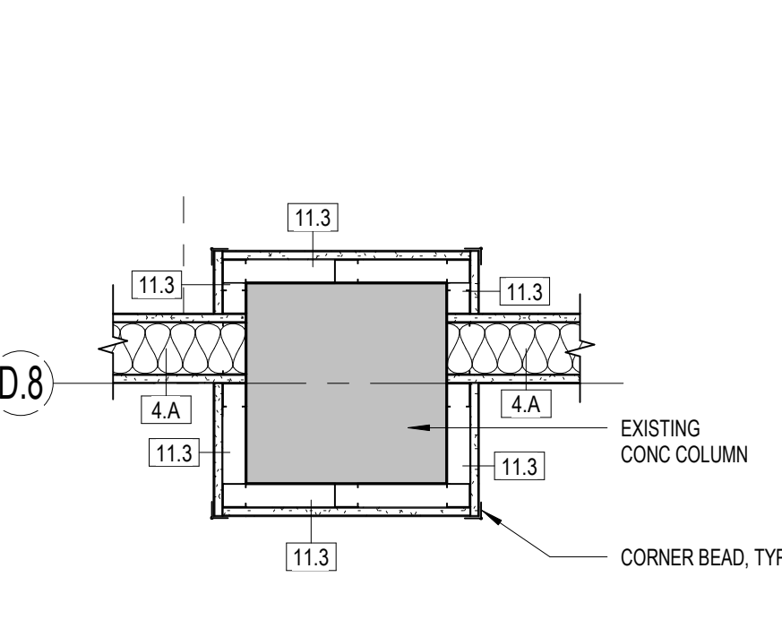
7 COLUMN PLAN DETAIL 1" = 1'-0"
