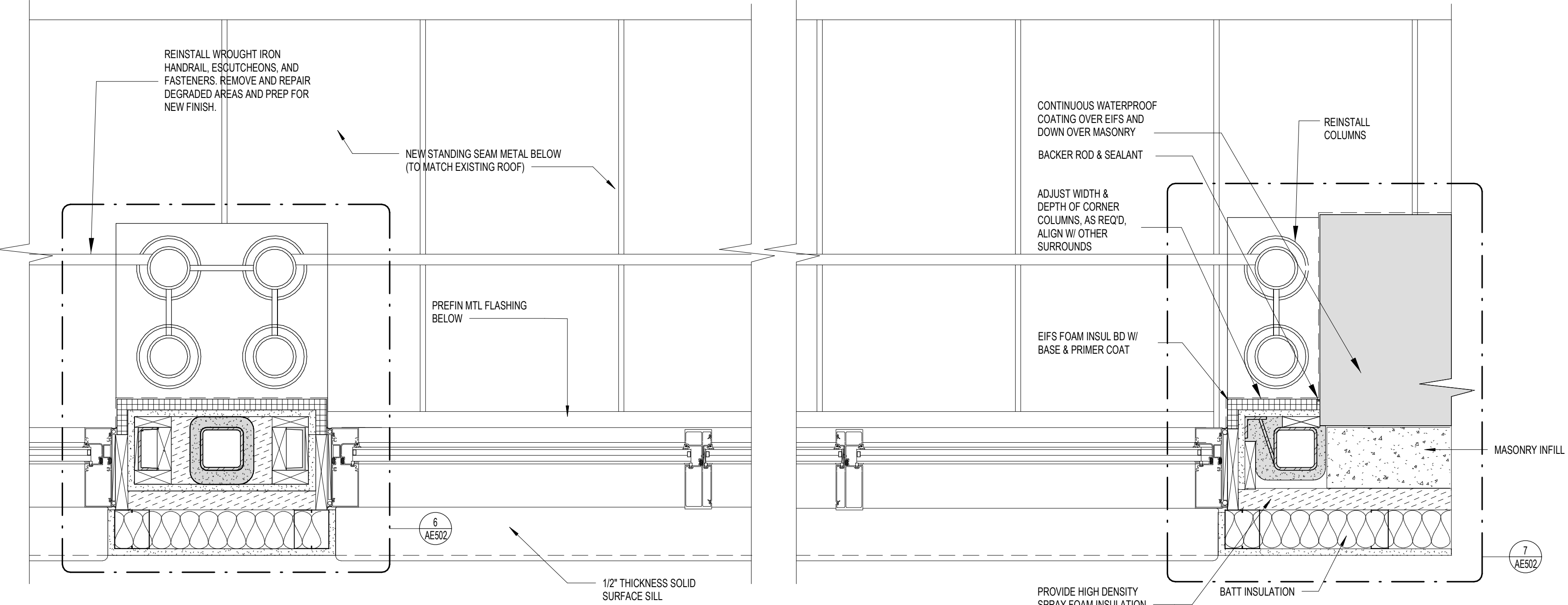
2 TYPICAL CURTAINWALL DETAIL - 5TH FLOOR AE502 1 1/2" = 1'-0"
