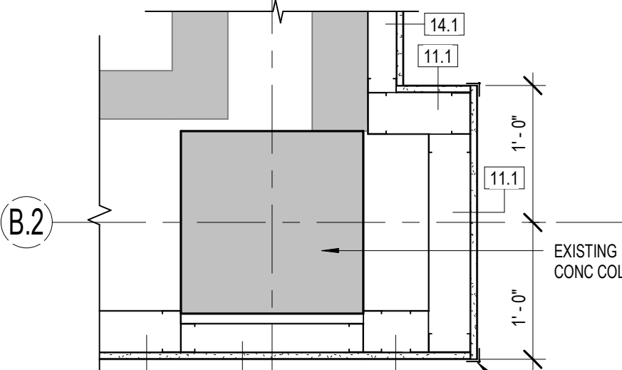
28 COLUMN PLAN DETAIL 1" = 1'-0"
