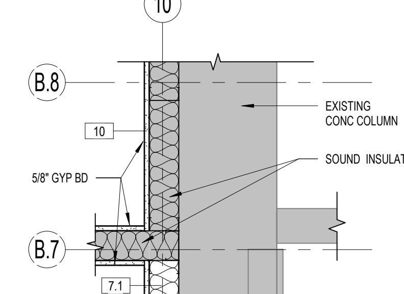
4 COLUMN PLAN DETAIL 1" = 1'-0"
