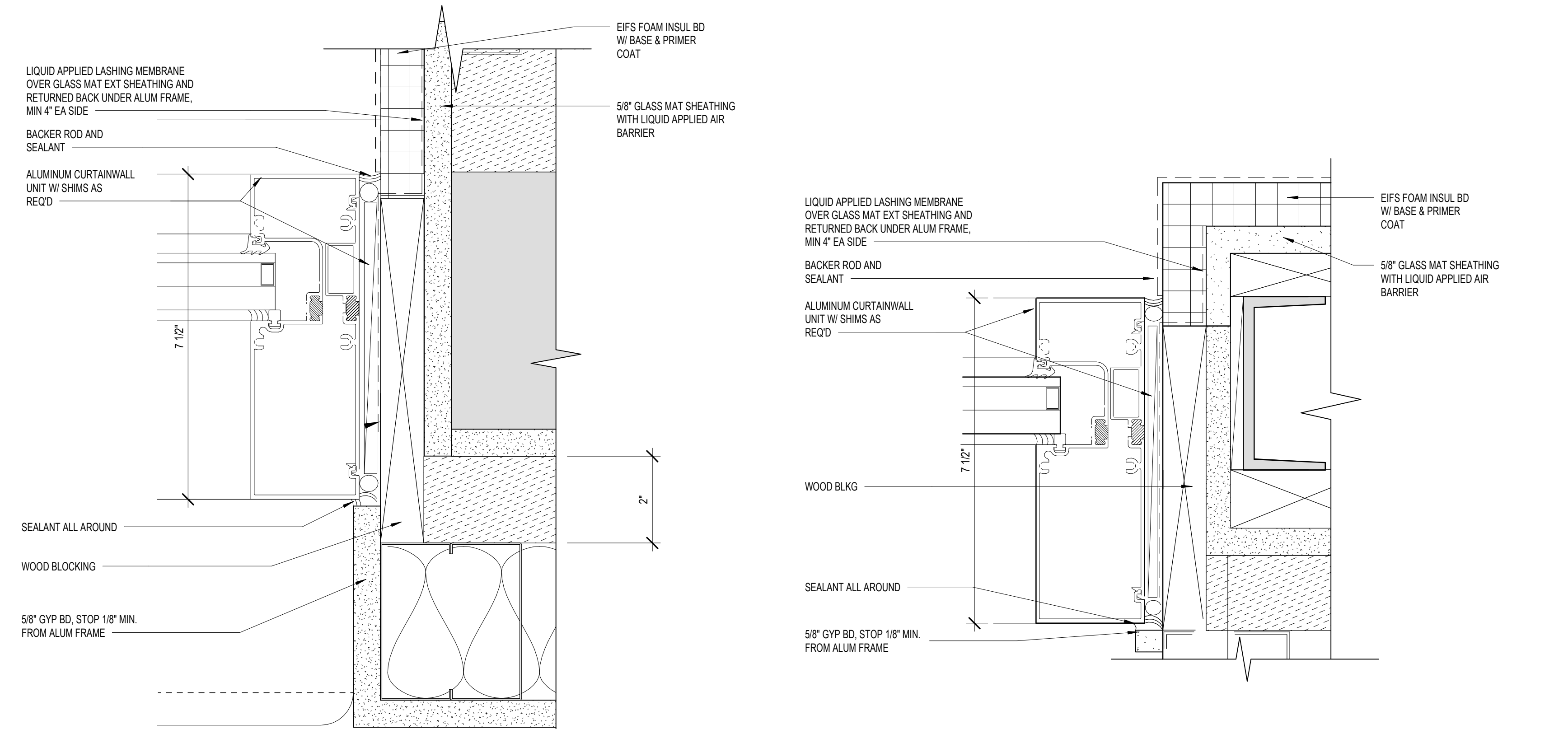
3 WINDOW JAMB & CONC COLUMN AE502 6" = 1'-0"
