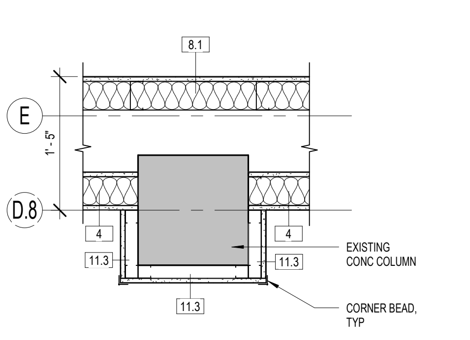
5 COLUMN PLAN DETAIL 1" = 1'-0"
