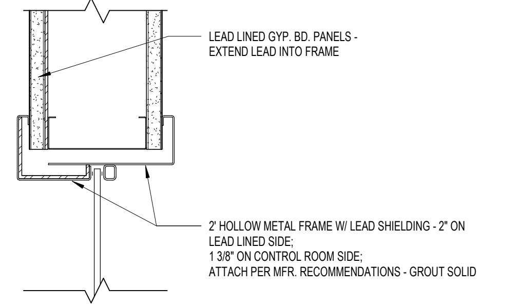
6 WINDOW HEAD - LEAD GLAZING AE612 3" = 1'-0"
