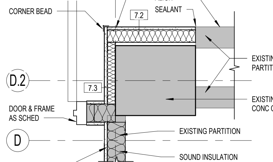
24 COLUMN PLAN DETAIL 1" = 1'-0"
