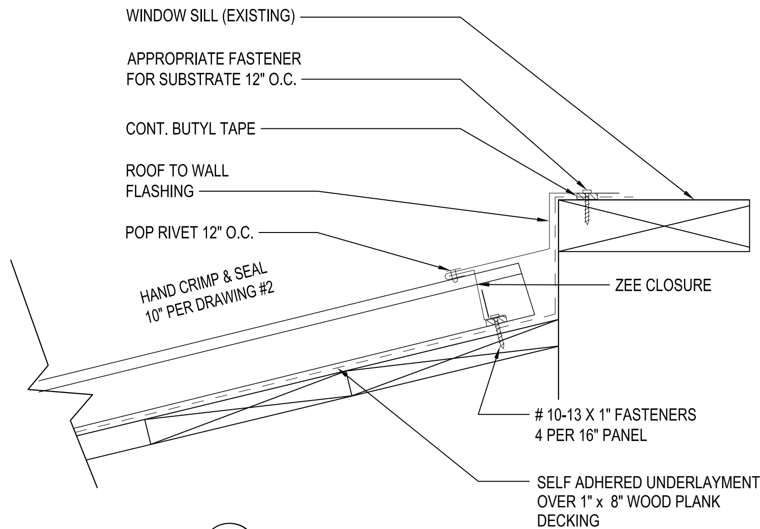
6 TRANSITION DETAIL AE503 SCALE: 1-1/2"=1'-0"
