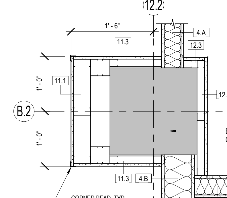
4 COLUMN PLAN DETAIL 1" = 1'-0"
