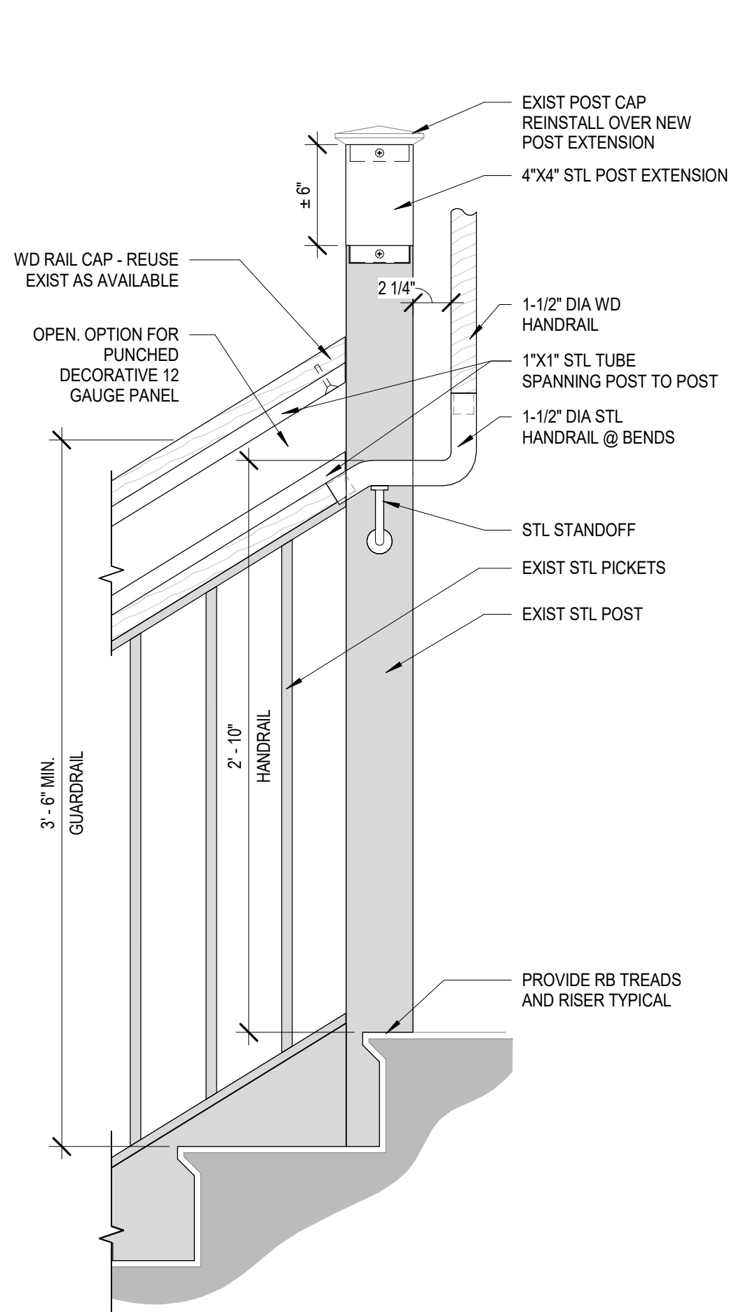
4 TYP STAIR RAIL DETAIL AE501/ 1 1/2" = 1'-0"
