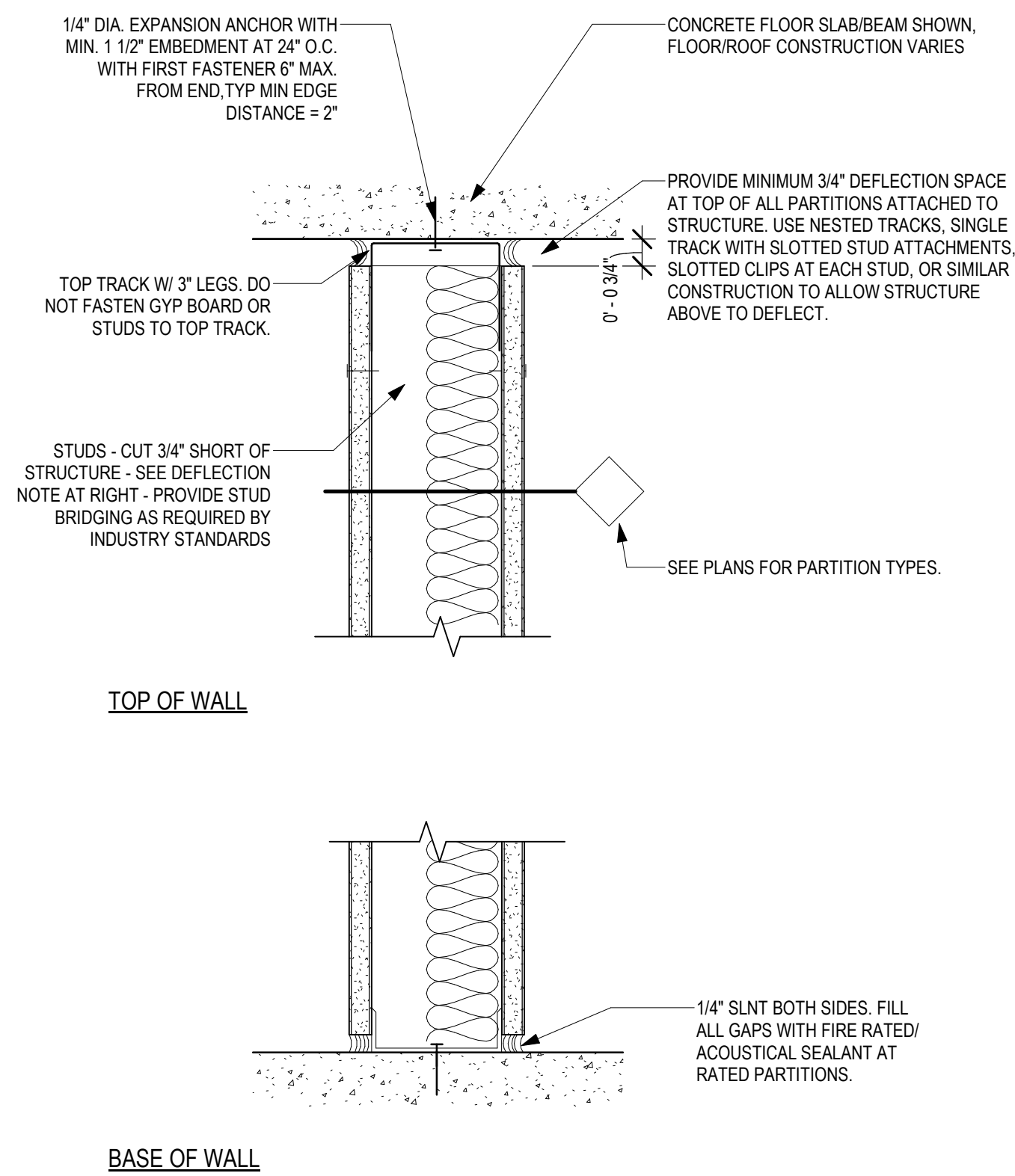
4 PARTITION DEFLECTION JOINT & FLOOR CLOSURE AE600/ 3" = 1'-0"
