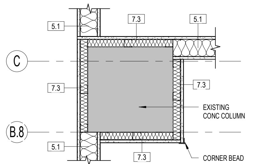
15 COLUMN PLAN DETAIL 1" = 1'-0"
