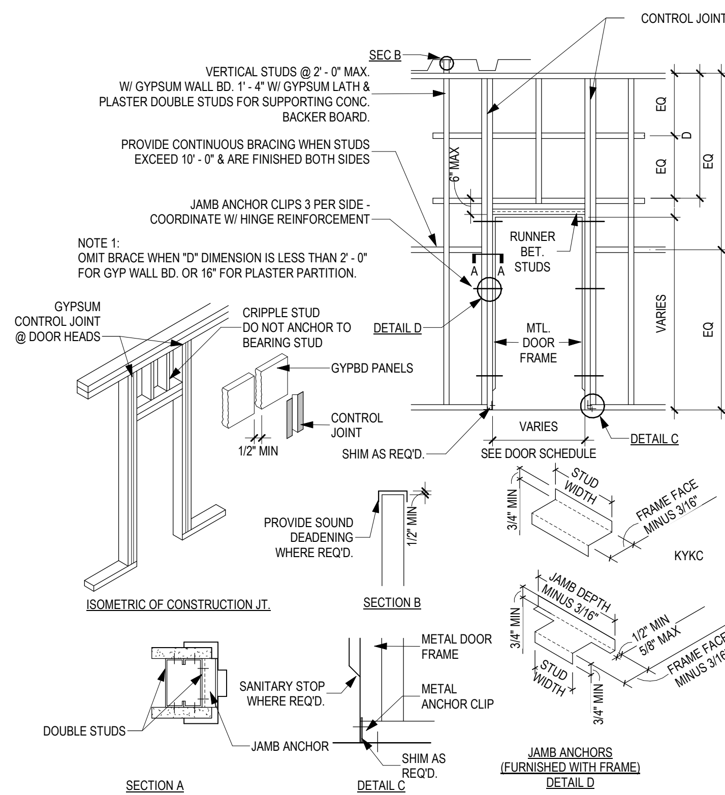
5 TYPICAL PARTITION CONTROL JOINT FRAMING AT DOORS AE600/ 1 1/2" = 1'-0"
