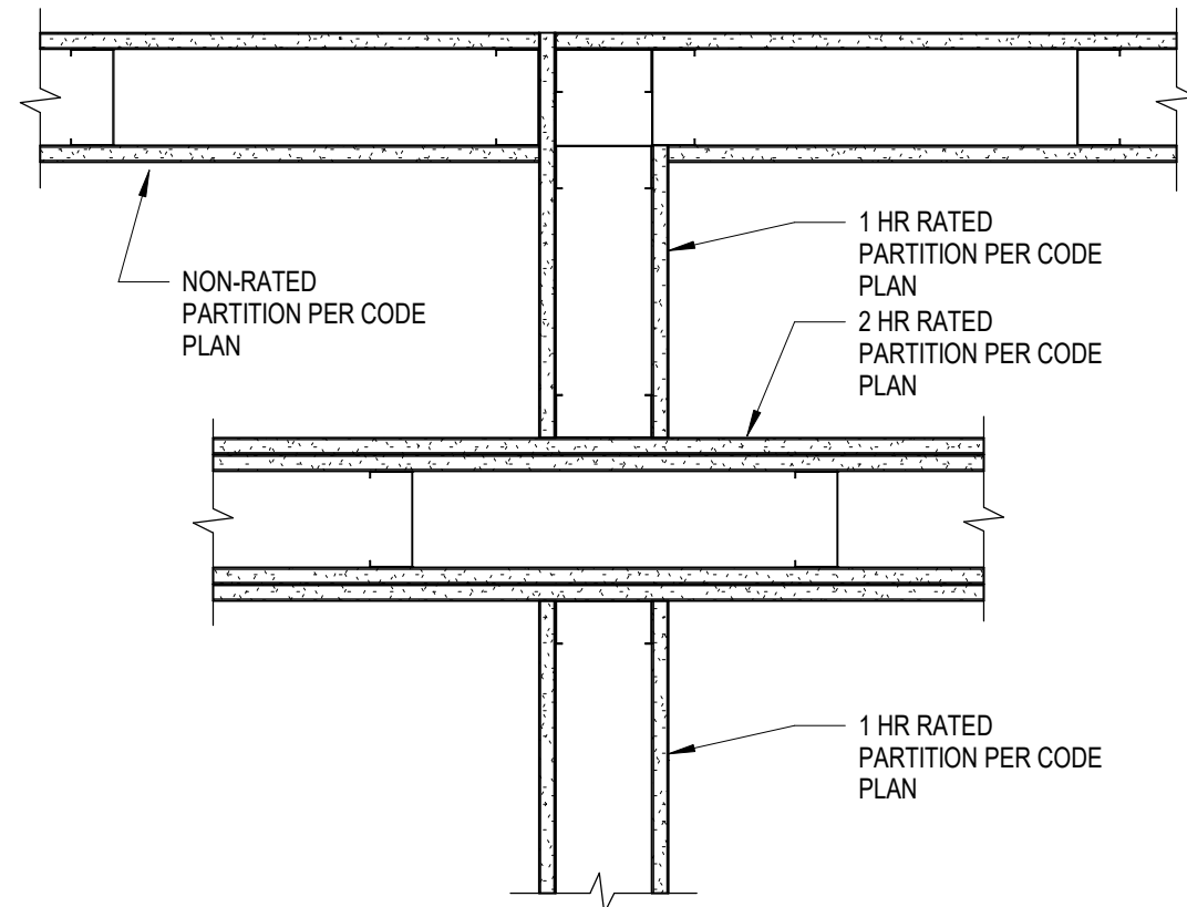
1 GUIDELINE - RATED WALL INTERSECTION AE600/ 1 1/2" = 1'-0"
