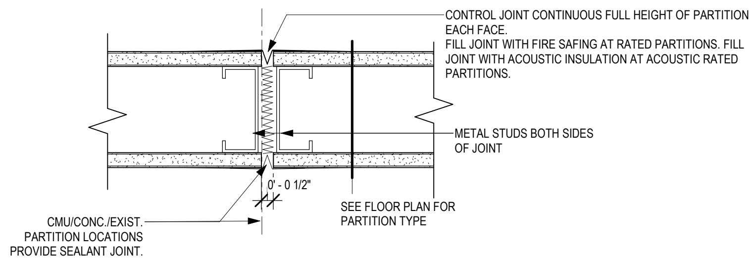
2 GYPSUM BOARD CONTROL JOINT AE600/ 3" = 1'-0"
