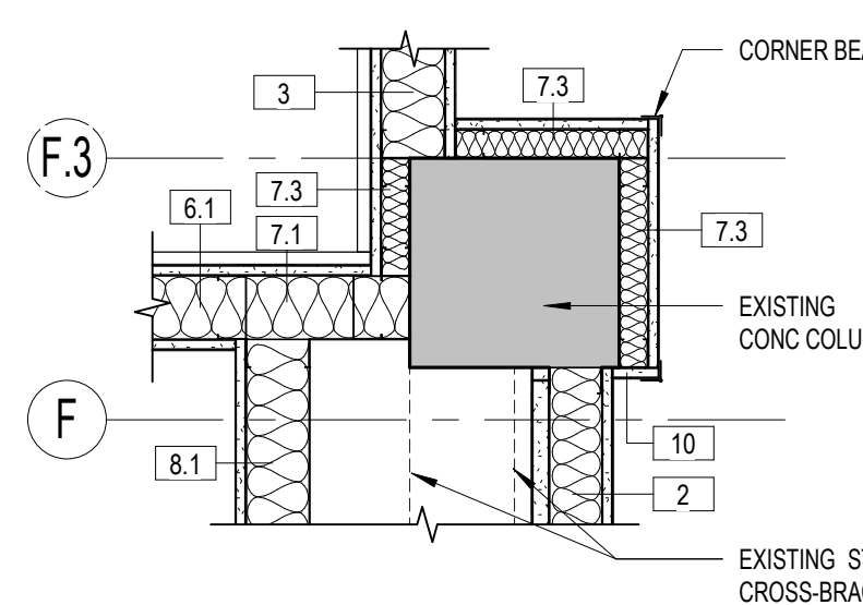
16 COLUMN PLAN DETAIL 1" = 1'-0"
