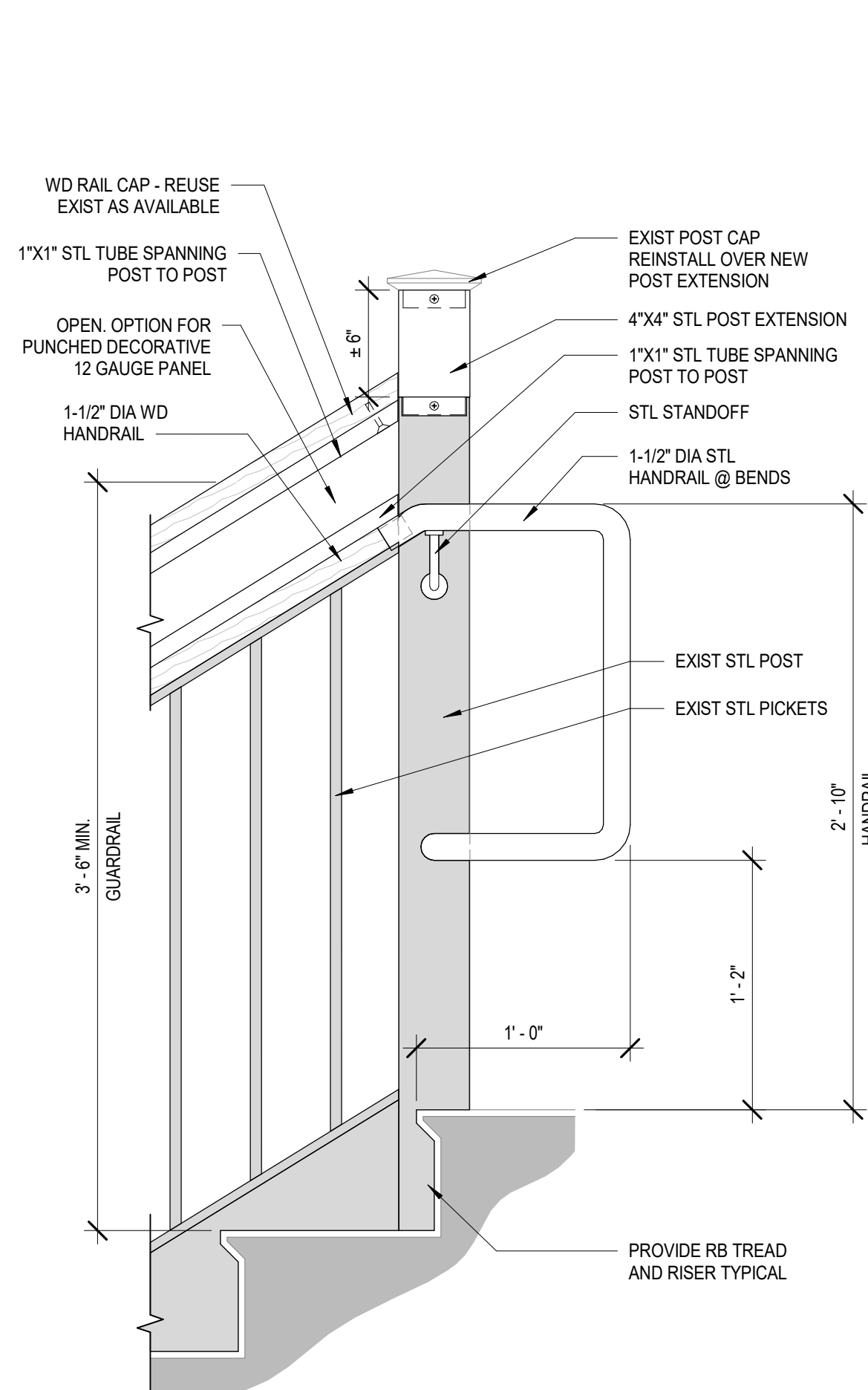
5 TYP STAIR RAIL DETAIL AE501/ 1 1/2" = 1'-0"
