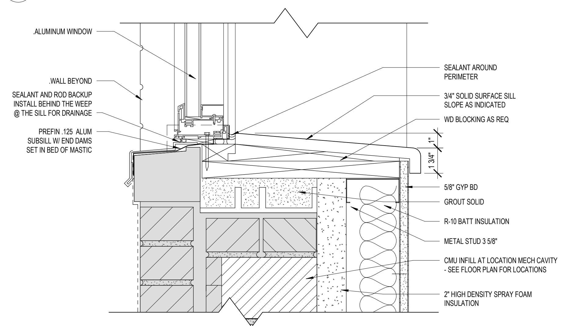
4 ALUMINUM WINDOW SILL DETAIL AE514 3" = 1'-0"
