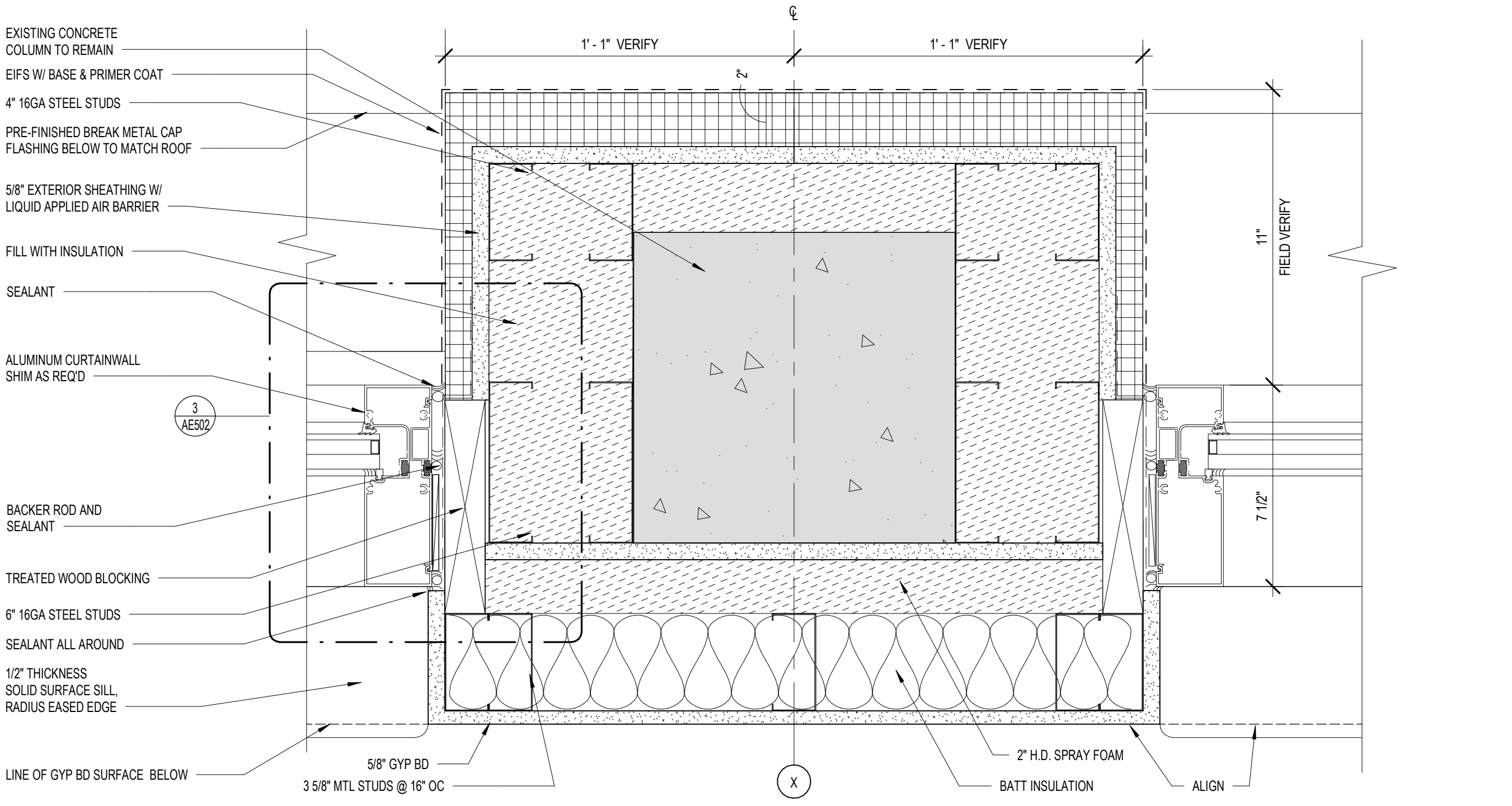
5 TYP (CONCRETE) COLUMN DETAIL - 3RD & 4TH FLOORS AE502 3" = 1'-0"
