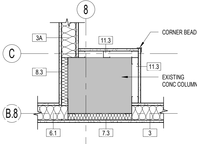
2 COLUMN PLAN DETAIL 1" = 1'-0"
