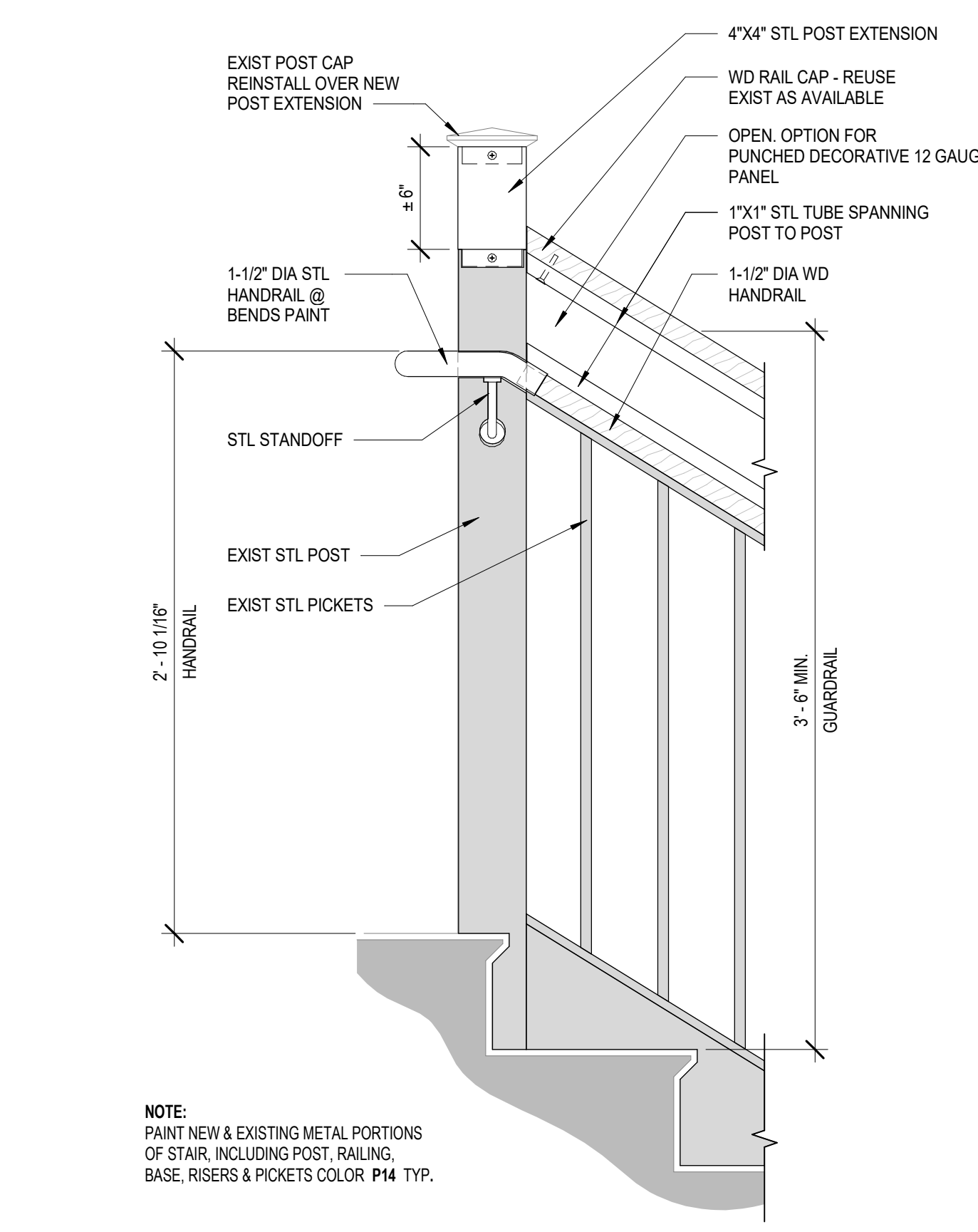
8 TYP STAIR RAIL DETAIL AE501/ 1 1/2" = 1'-0"
