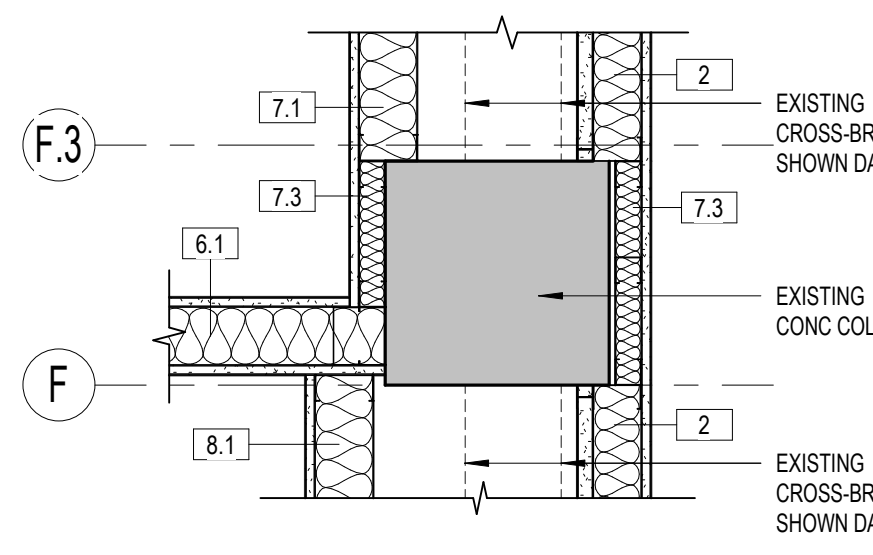
17 COLUMN PLAN DETAIL 1" = 1'-0"
