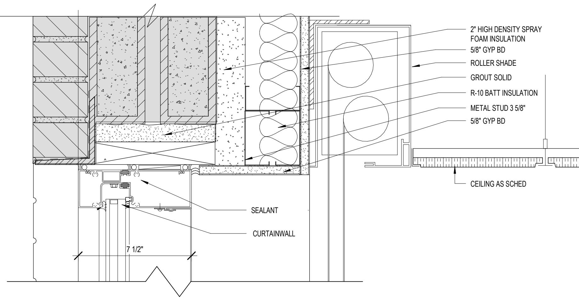
5 CURTAINWALL HEAD DETAIL AE514 3" = 1'-0"
