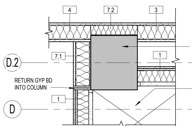
23 COLUMN PLAN DETAIL 1" = 1'-0"
