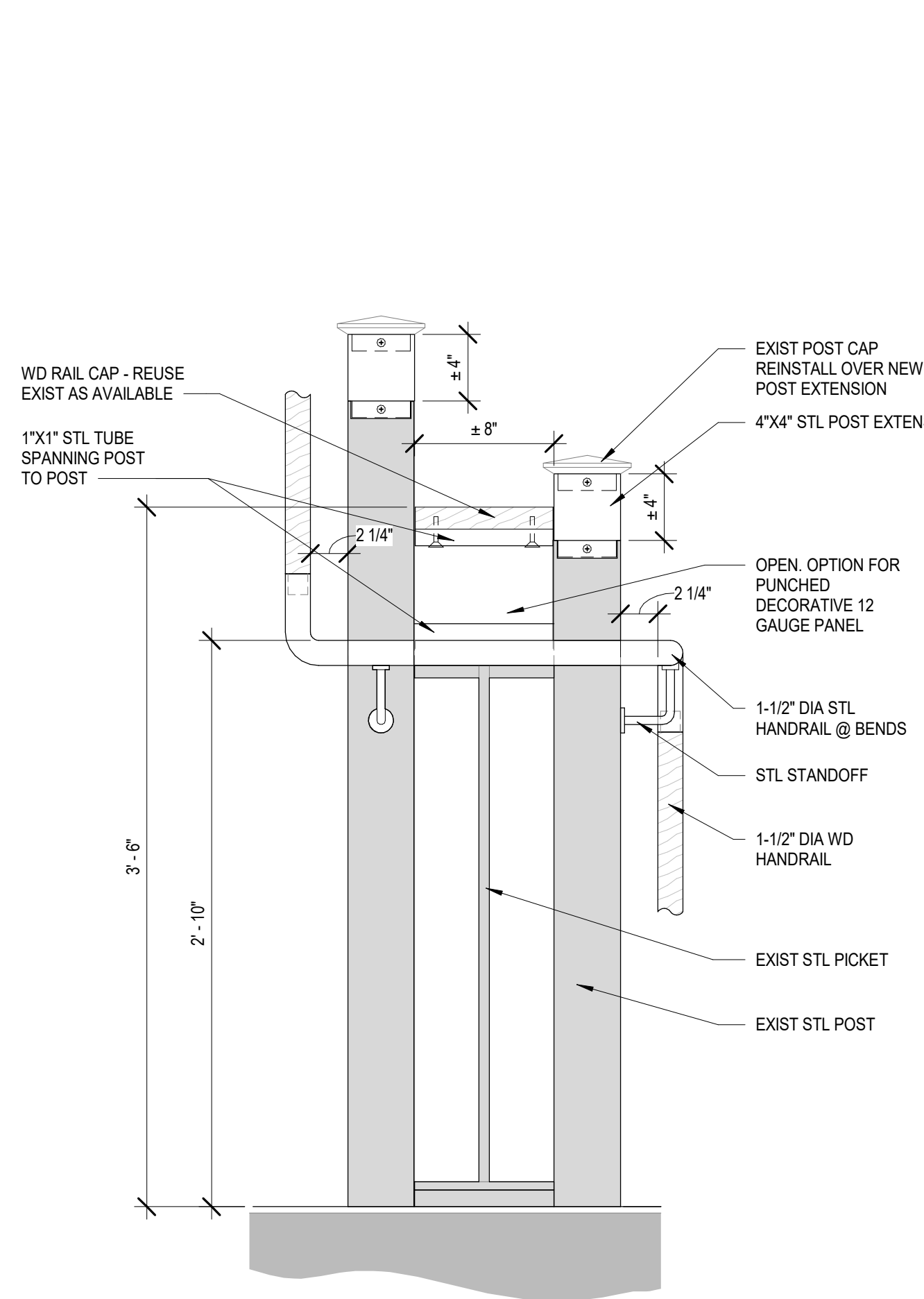
6 TYP STAIR RAIL DETAIL AE501/ 1 1/2" = 1'-0"
