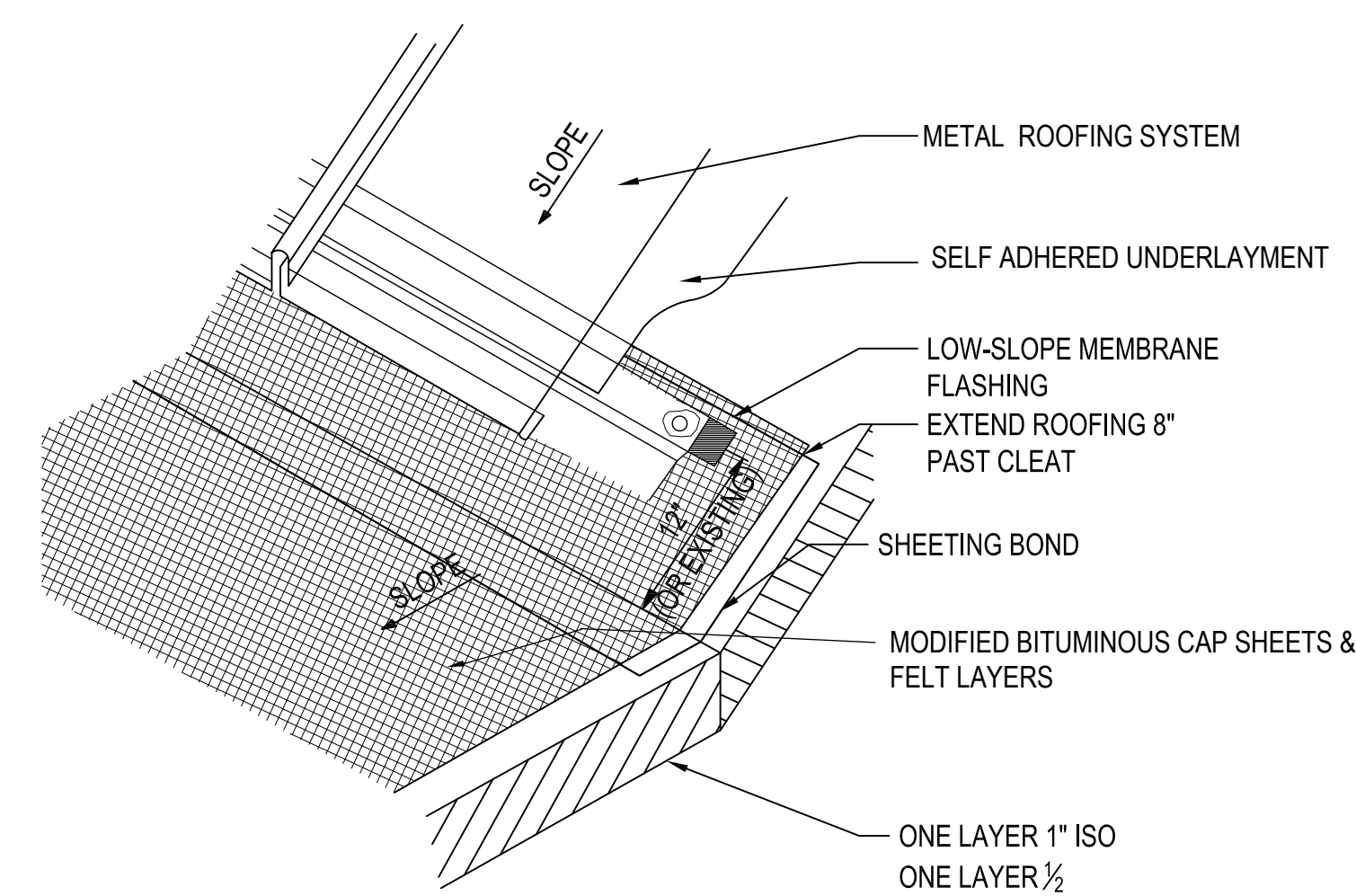
8 TRANSITION ROOF DETAIL AE503 SCALE: 1-1/2"=1'-0"
