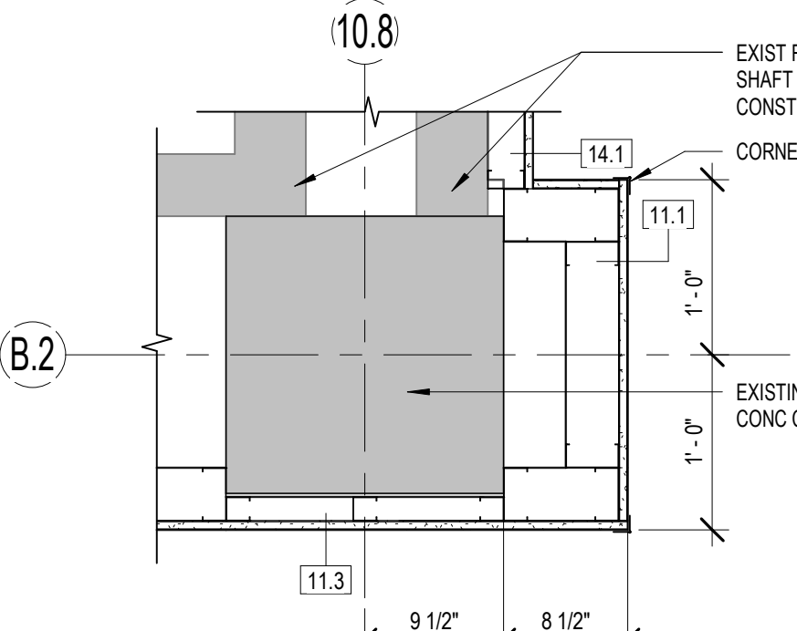
3 COLUMN PLAN DETAIL 1" = 1'-0"
