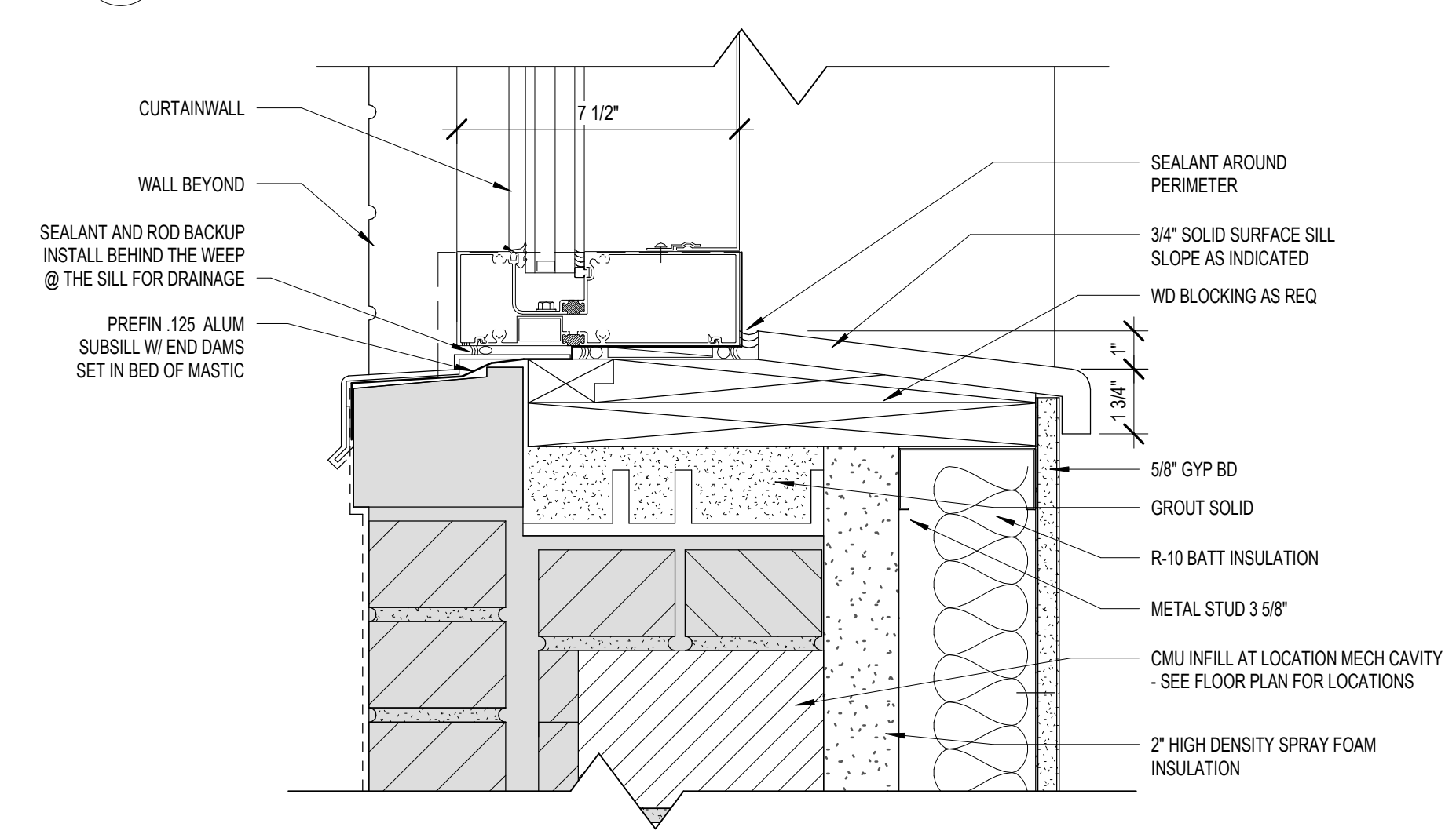
8 CURTAINWALL SILL DETAIL AE514 3" = 1'-0"
