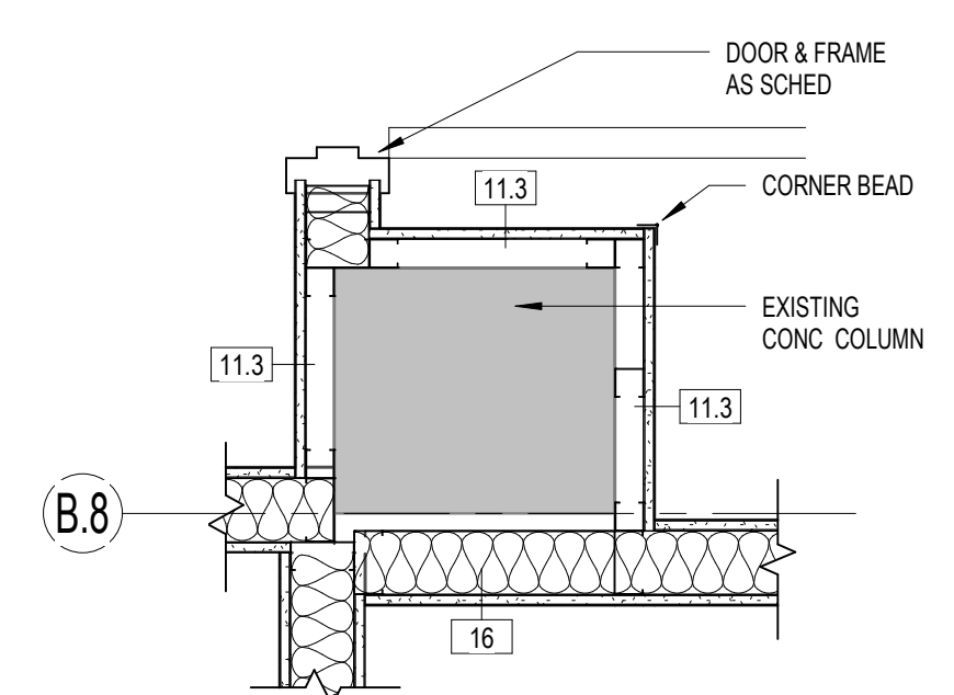
8 COLUMN PLAN DETAIL 1" = 1'-0"
