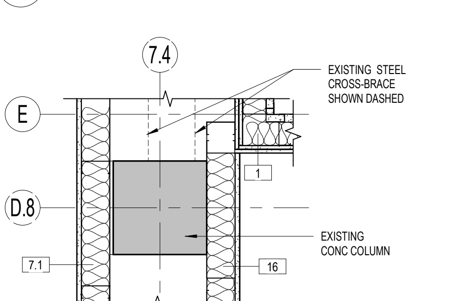
26 COLUMN PLAN DETAIL 1" = 1'-0"
