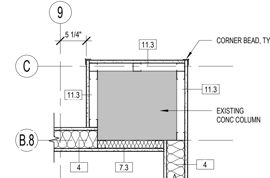
3 COLUMN PLAN DETAIL 1" = 1'-0"
