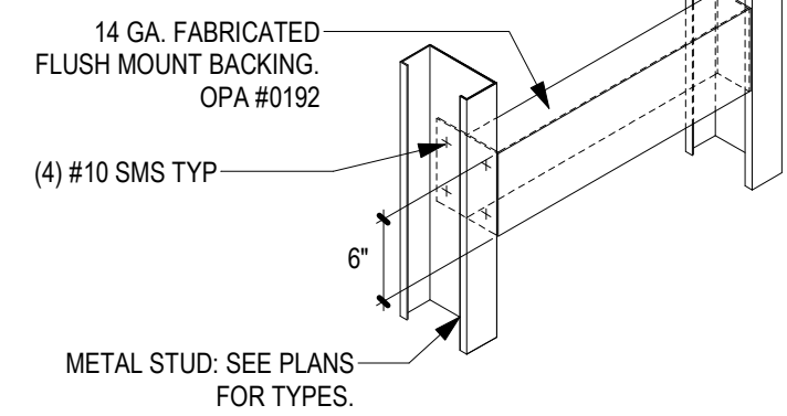
3 PARTITION BLOCKING-BACKING TYPES AE600/ 3" = 1'-0"
