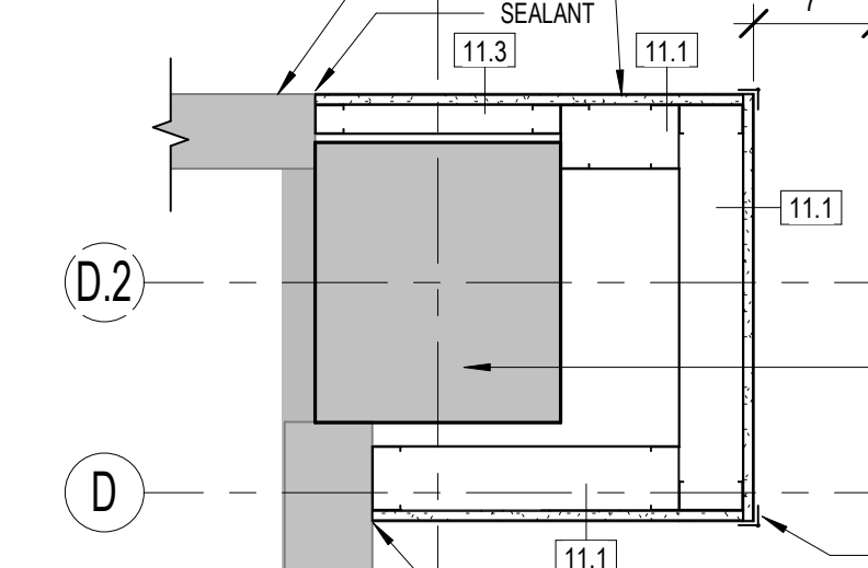
25 COLUMN PLAN DETAIL 1" = 1'-0"
