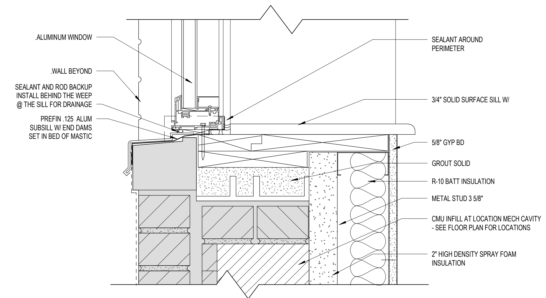
3 ALUMINUM WINDOW SILL DETAIL AE514 3" = 1'-0"
