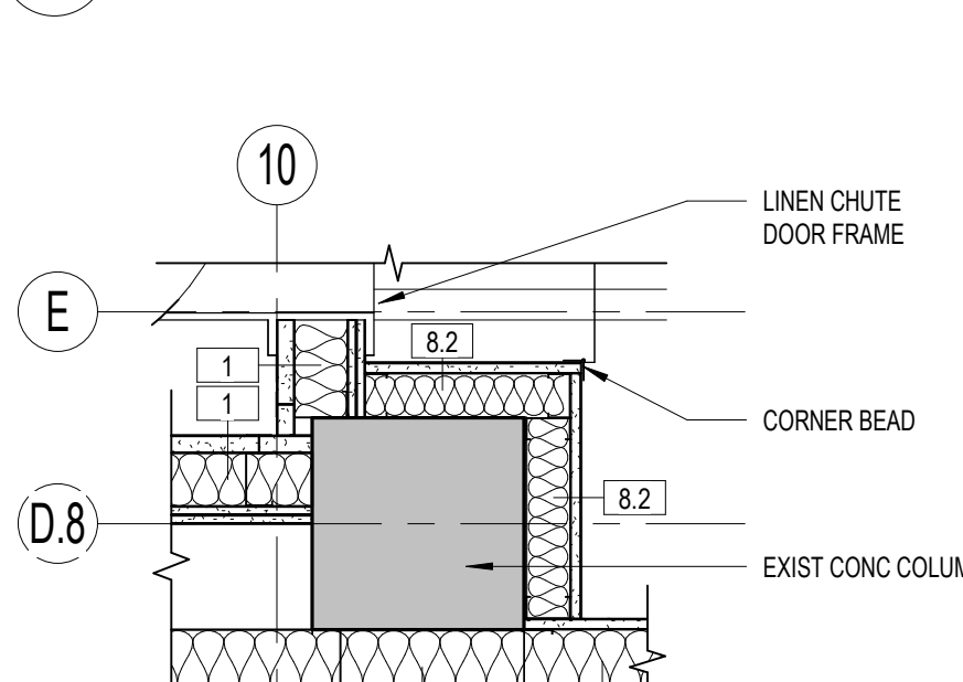
28 COLUMN PLAN DETAIL 1" = 1'-0"
