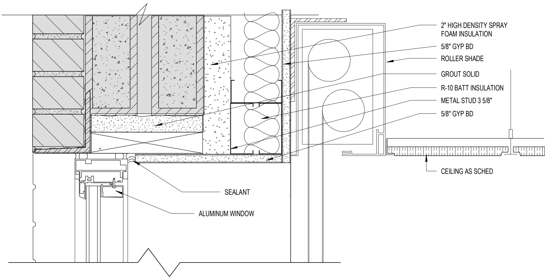
1 ALUMINUM WINDOW HEAD DETAIL AE514 3" = 1'-0"
