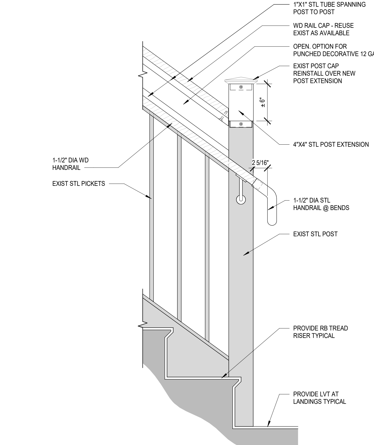
9 TYP STAIR RAIL DETAIL AE501/ 1 1/2" = 1'-0"
