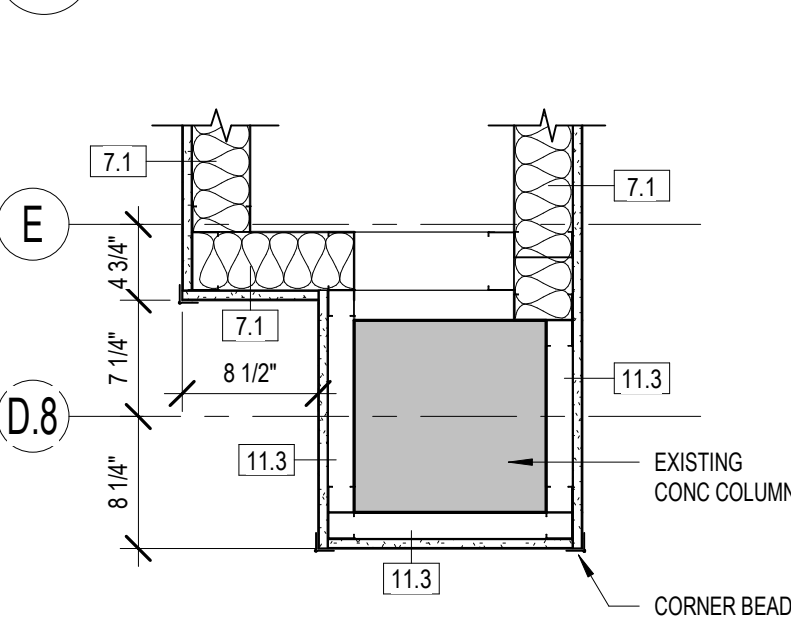
23 COLUMN PLAN DETAIL 1" = 1'-0"
