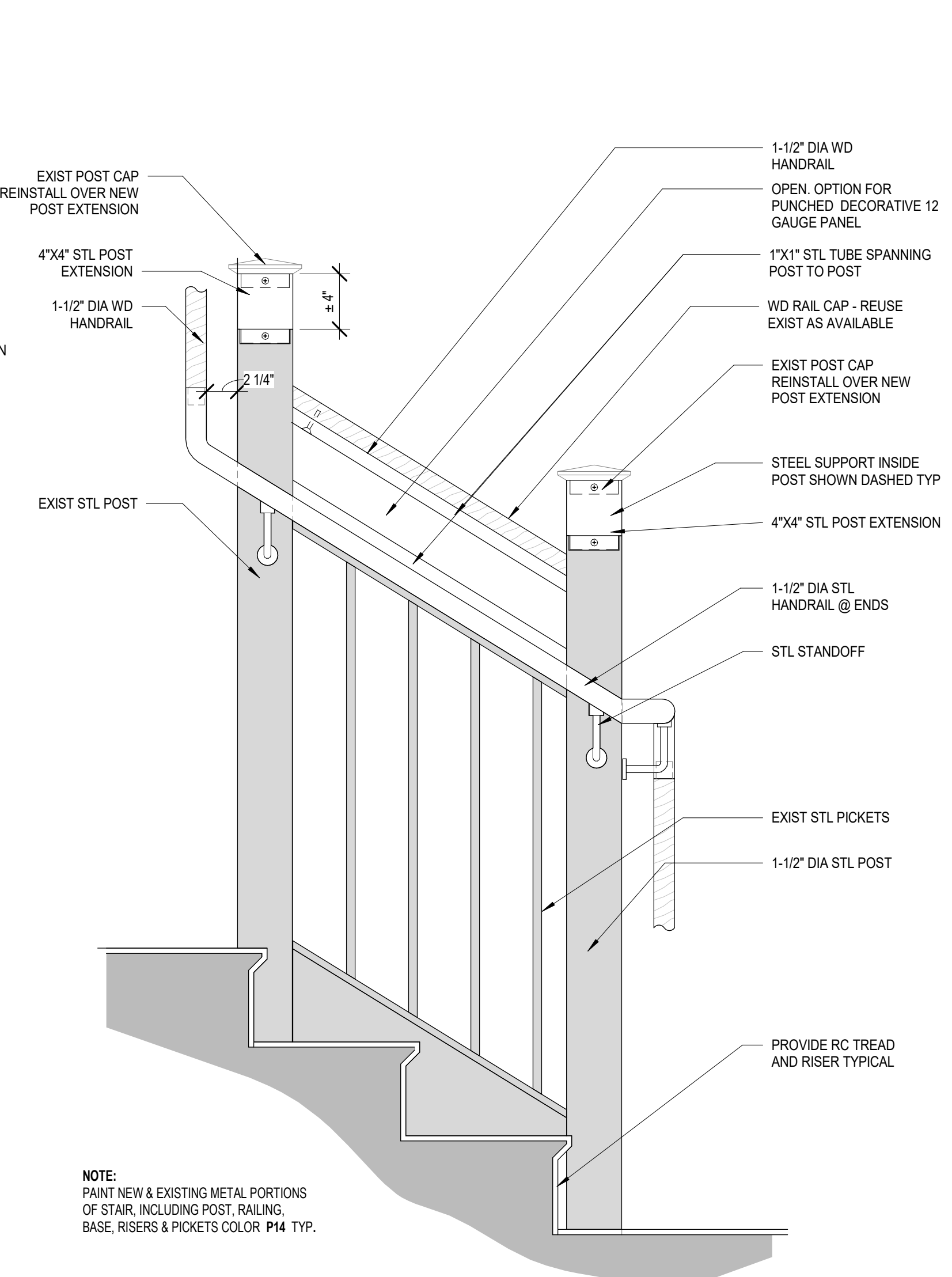
7 TYP STAIR LANDING DETAIL AE501/ 1 1/2" = 1'-0"
