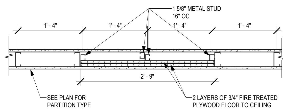
6 PARTITION DETAIL AT IN-WALL BLOCKING AT XRAY UNIT AE600/ 1" = 1'-0"
