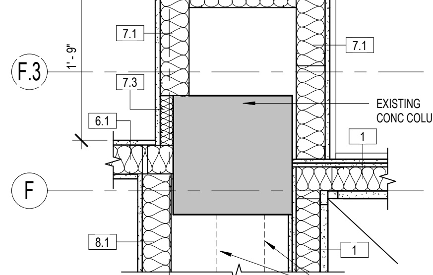
21 COLUMN PLAN DETAIL 1" = 1'-0"
