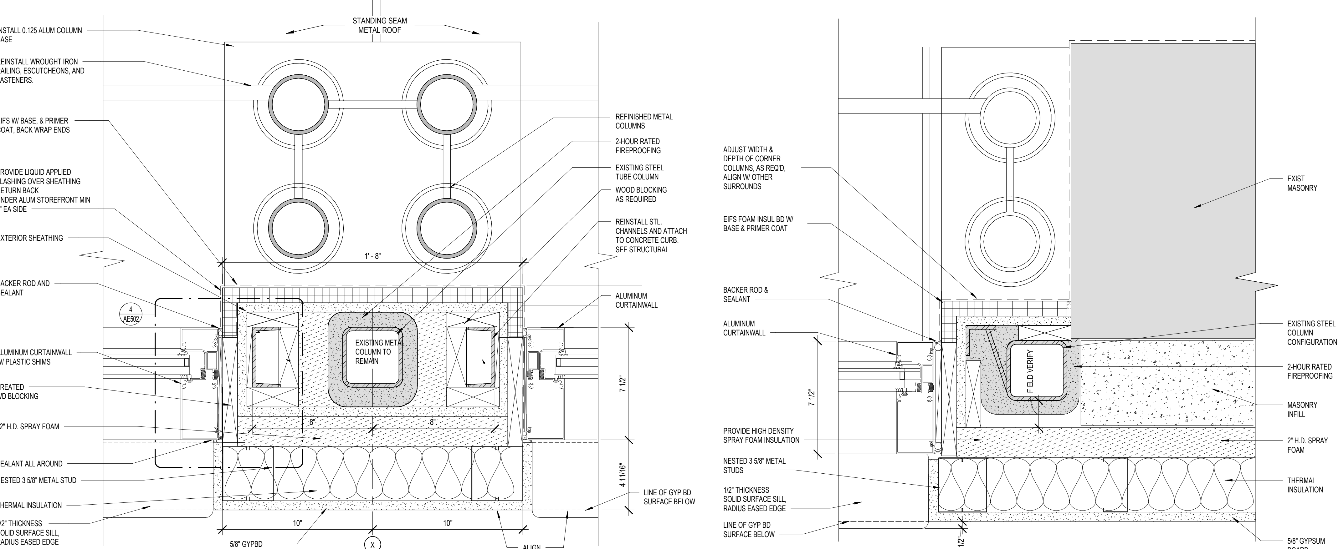
6 COLUMN DETAIL - 5TH FLOOR AE502 3" = 1'-0"
