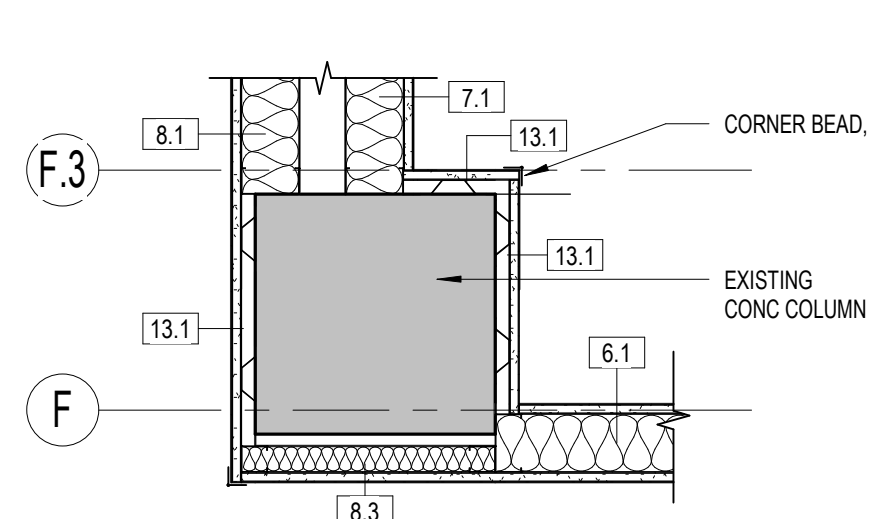
22 COLUMN PLAN DETAIL 1" = 1'-0"
