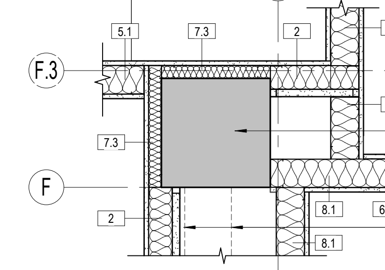
18 COLUMN PLAN DETAIL 1" = 1'-0"
