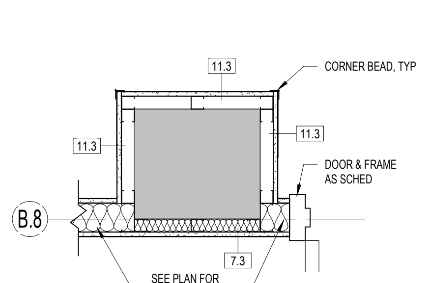
7 COLUMN PLAN DETAIL 1" = 1'-0"
