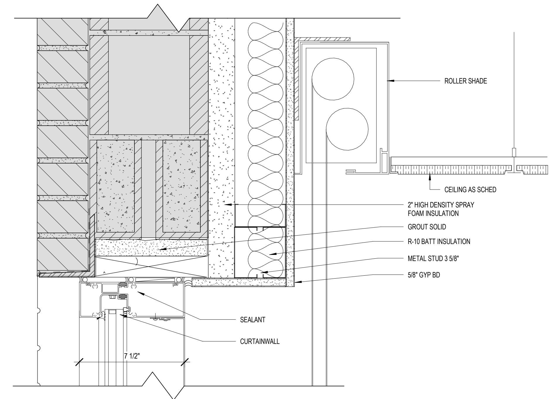
11 CURTAINWALL HEAD DETAIL AE514 3" = 1'-0"
