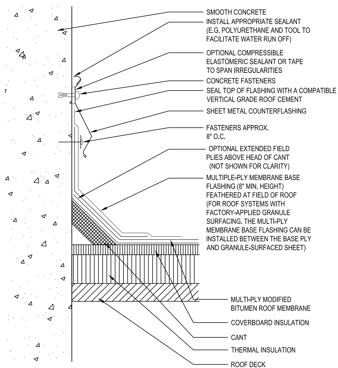
9 WALL TERMINATION DETAIL AE503 SCALE: 1-1/2"=1'-0"
