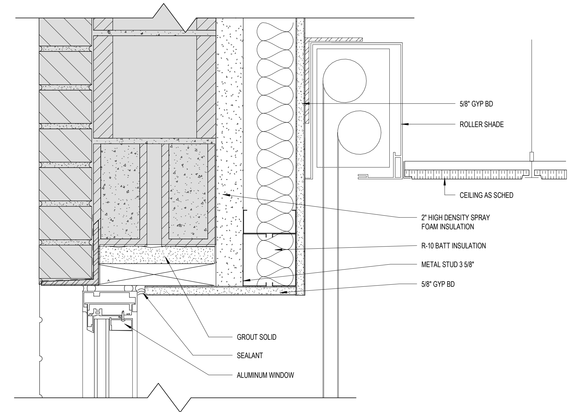
10 ALUMINUM WINDOW HEAD DETAIL AE514 3" = 1'-0"
