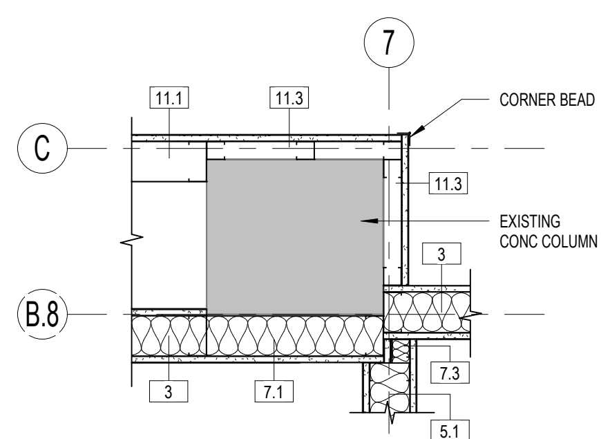
1 COLUMN PLAN DETAIL 1" = 1'-0"
