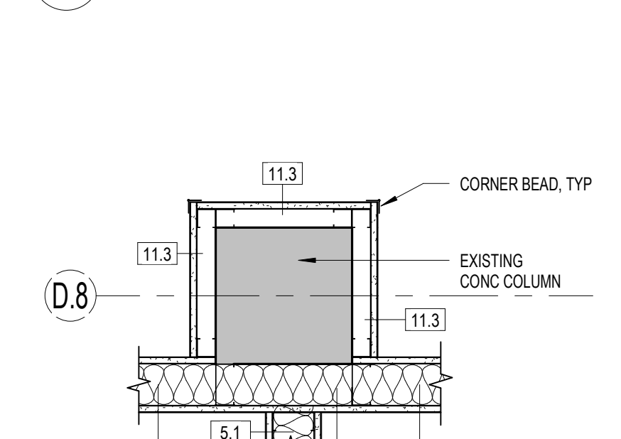
27 COLUMN PLAN DETAIL 1" = 1'-0"
