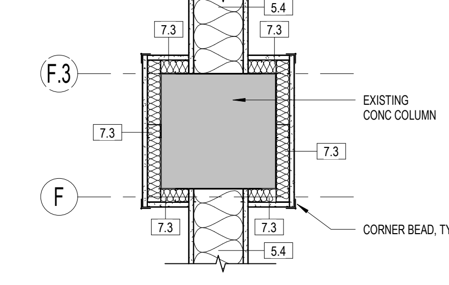
20 COLUMN PLAN DETAIL 1" = 1'-0"
