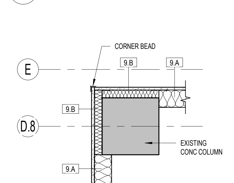
25 COLUMN PLAN DETAIL 1" = 1'-0"
