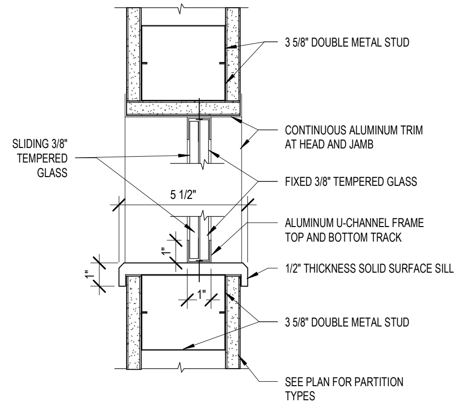
8 TRANSACTION WINDOW DETAIL AE612 3" = 1'-0"
