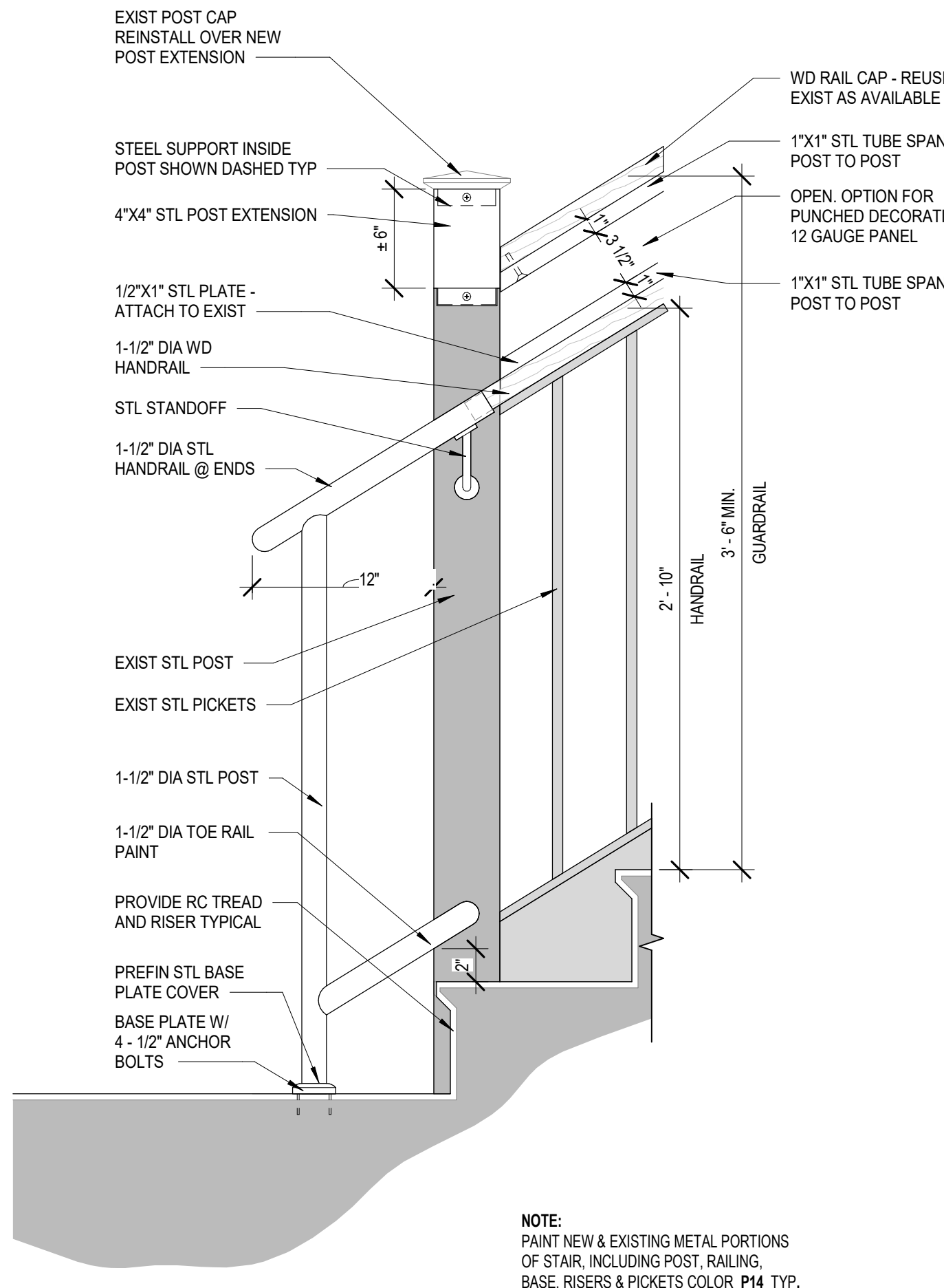
1 TYP STAIR LANDING DETAIL AE501/ 1 1/2" = 1'-0"
