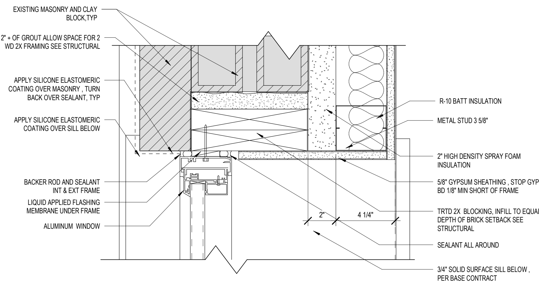
2 ALUMINUM WINDOW JAMB DETAIL AE514 3" = 1'-0"
