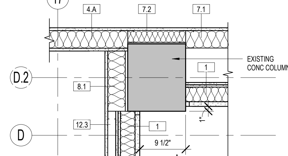
26 COLUMN PLAN DETAIL 1" = 1'-0"
