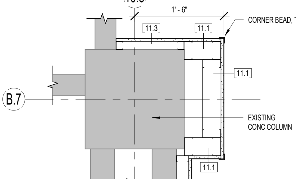
5 COLUMN PLAN DETAIL 1" = 1'-0"
