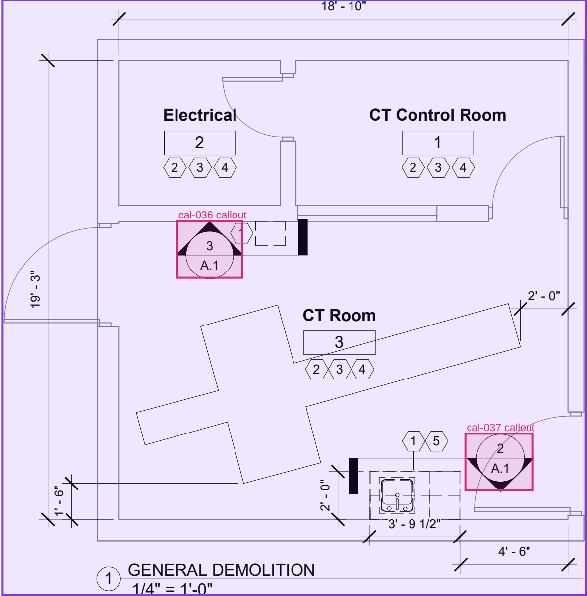
flp-003 floor plan
