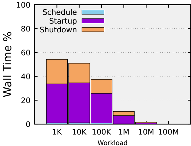
(a) Overhead Analysis
