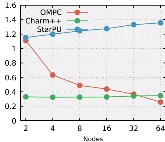
(c) Stencil-1D periodic
