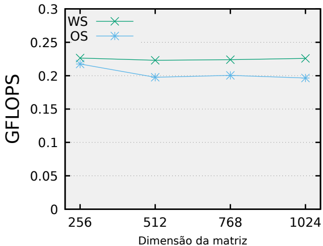
(a) SGEMV
