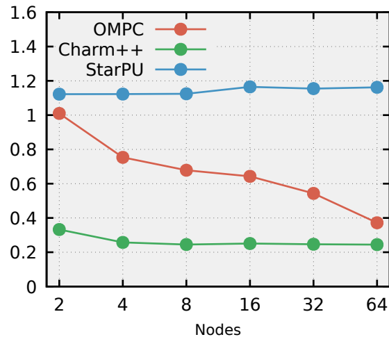
(b) Tree
