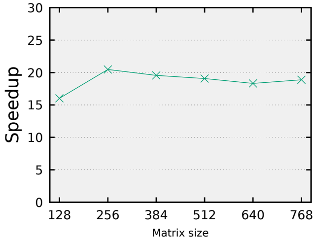
(a) SGEMM
