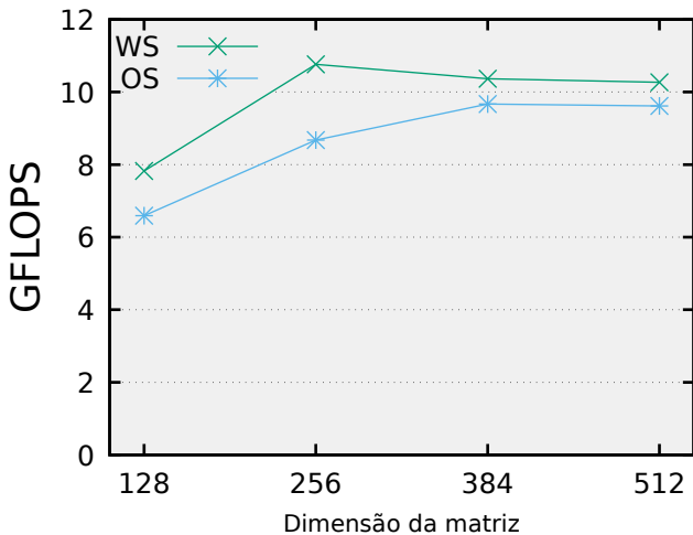
(b) SGEMM
