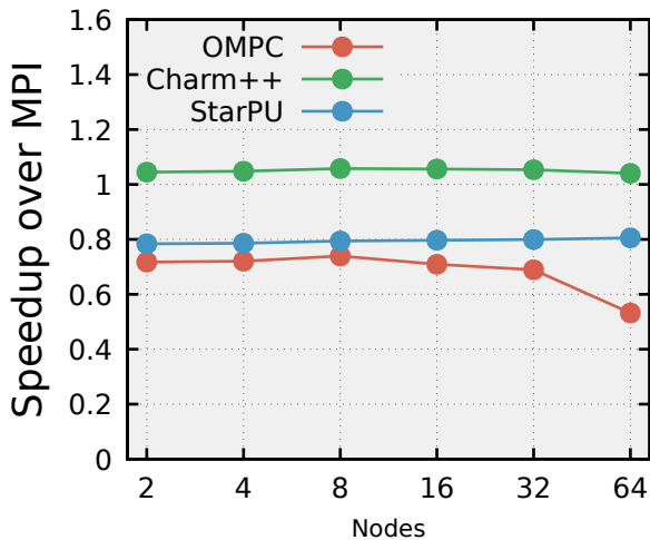
(a) Trivial
