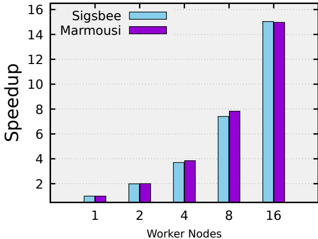
(b) Awave Scalability
