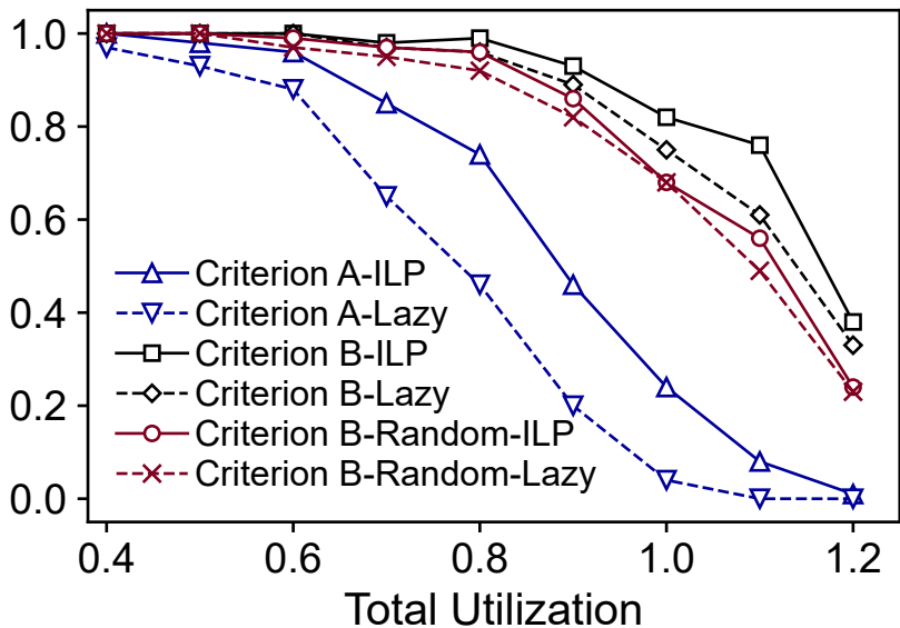
Schedulability Ratio
