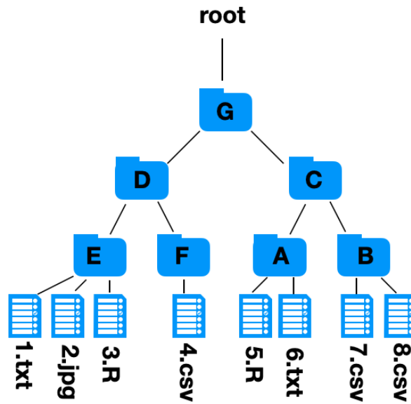
Figure 2: File system
