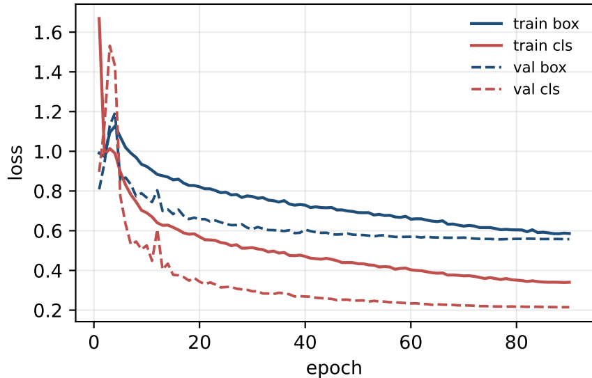
(a) Training and validation loss
