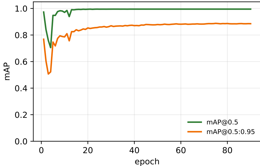
(b) Validation detection accuracy
