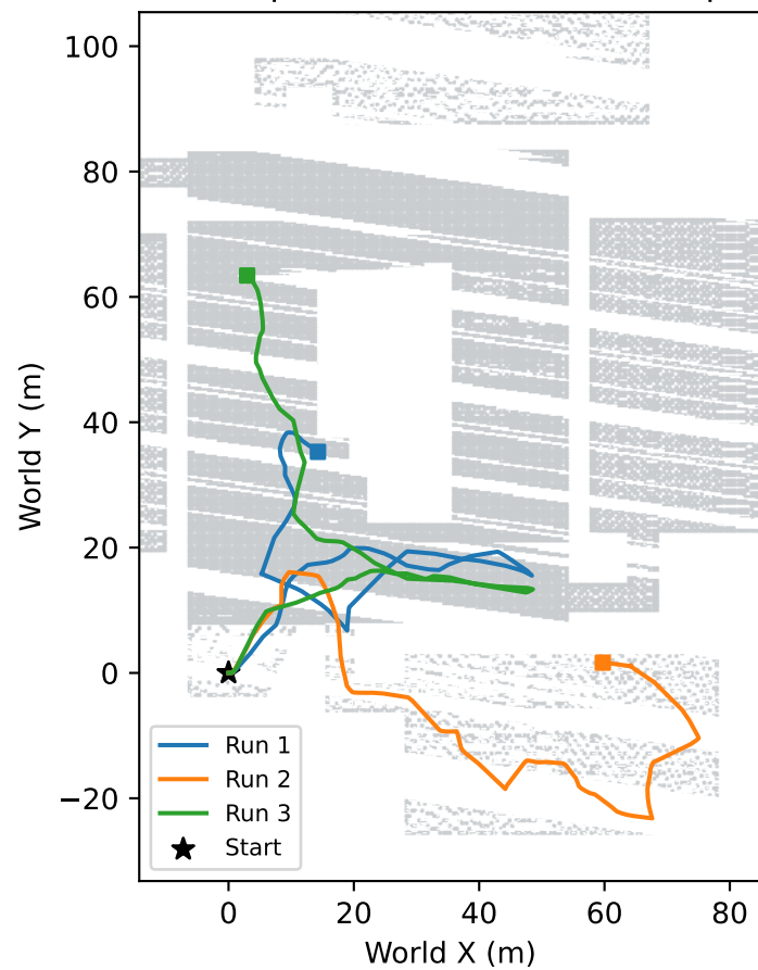
BASELINE: XY paths, reference surface projection
