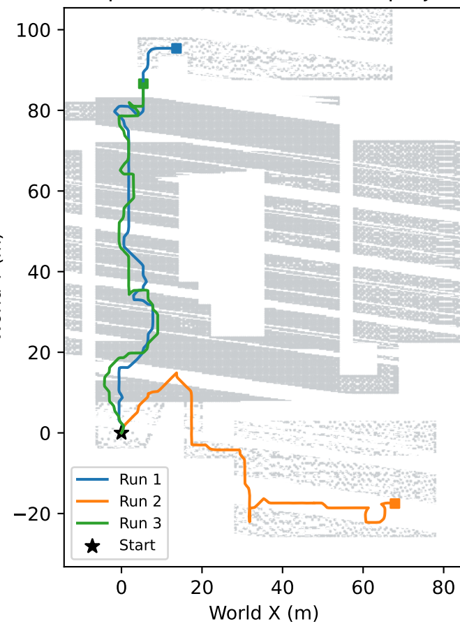
HT: XY paths, reference surface projection
