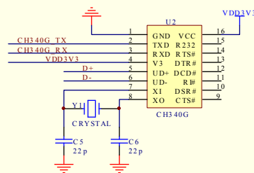
CH340G串口芯片
