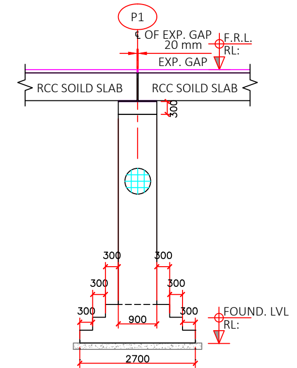
PCC PIER SECTION
