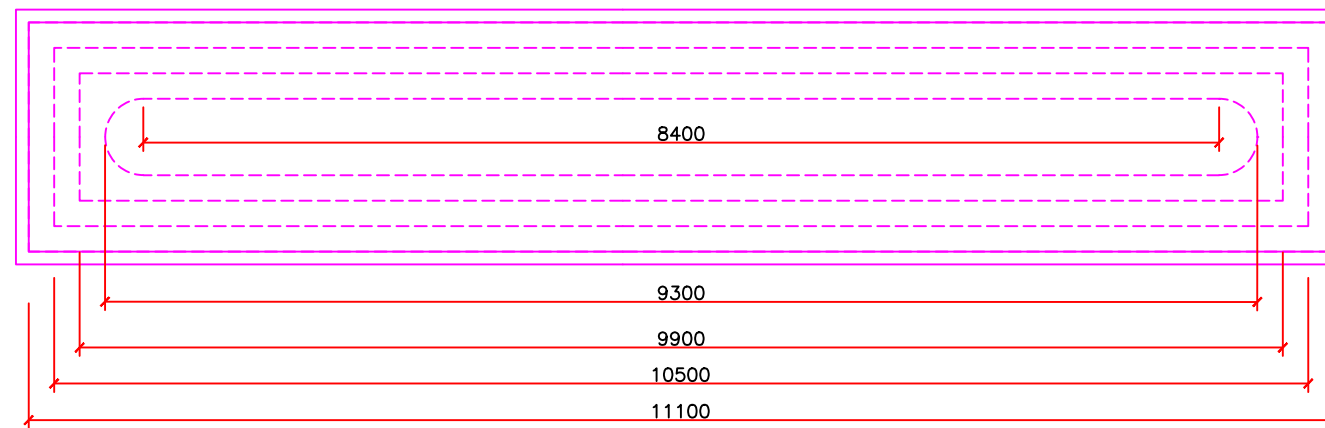
PCC PIER PLAN
