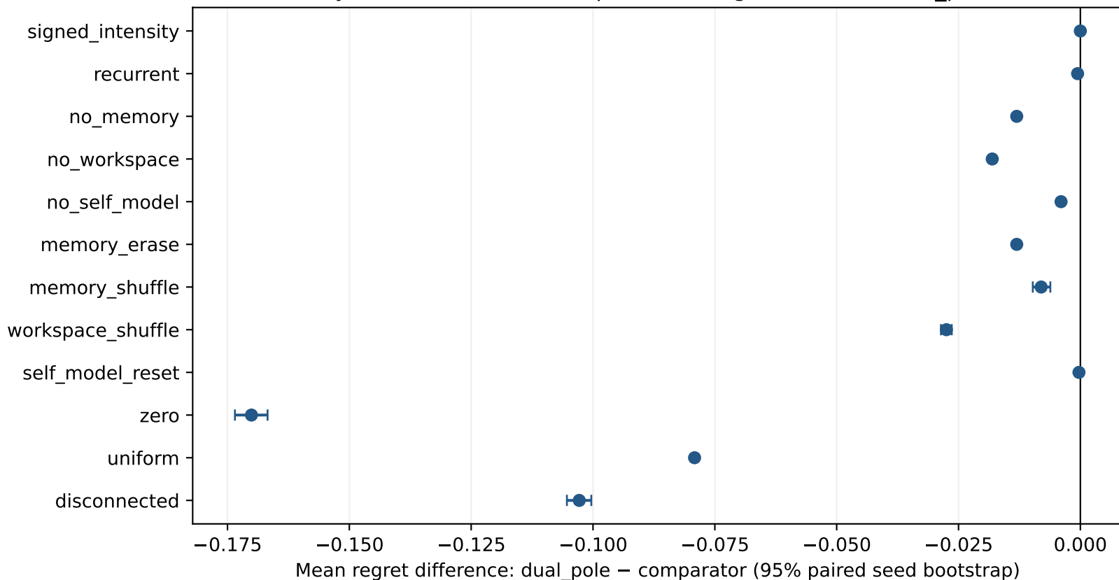
Synthetic controller comparisons; negative favors dual_pole
