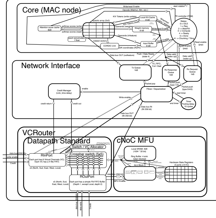
Figure 1: Detailed microarchitecture of a single NoCDAS tile.
