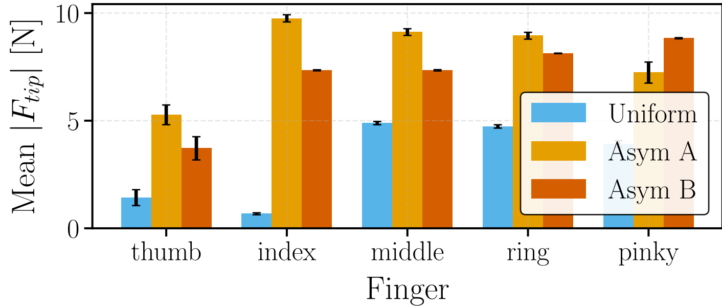
Contact force magnitude (1st-order model)
