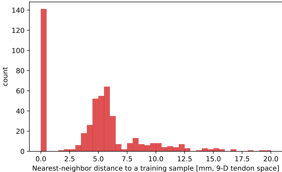
MULTI: test-to-train nearest-neighbor distance
