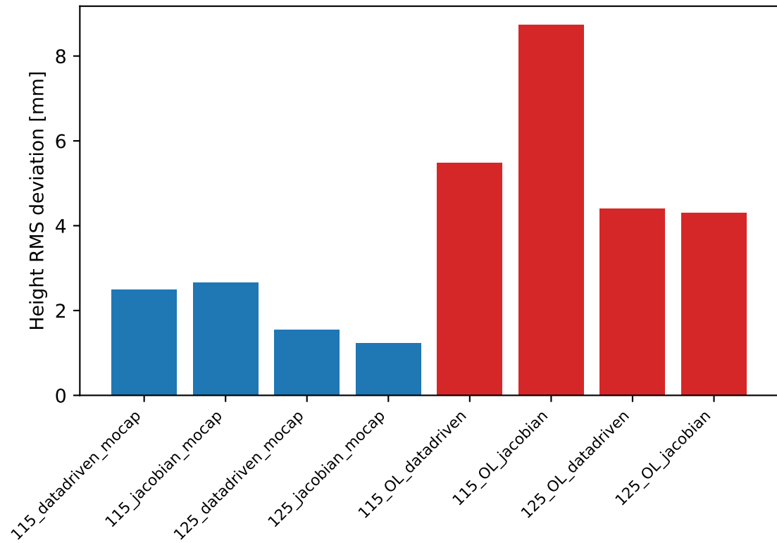
SINGLE: height path error
