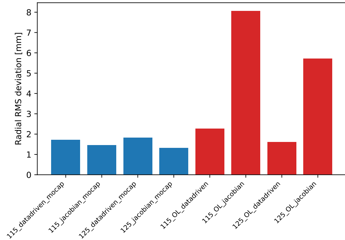
SINGLE: radial path error
