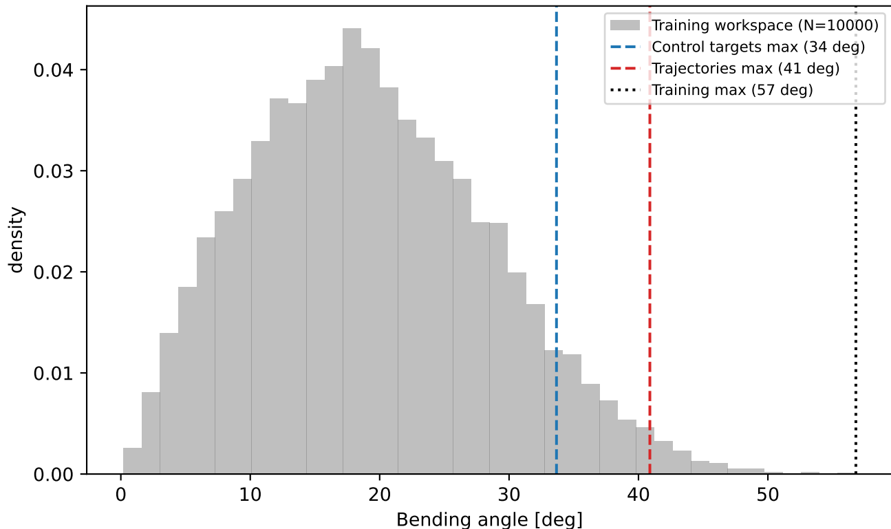
SINGLE: bending-angle coverage, control evaluation vs. training workspace
