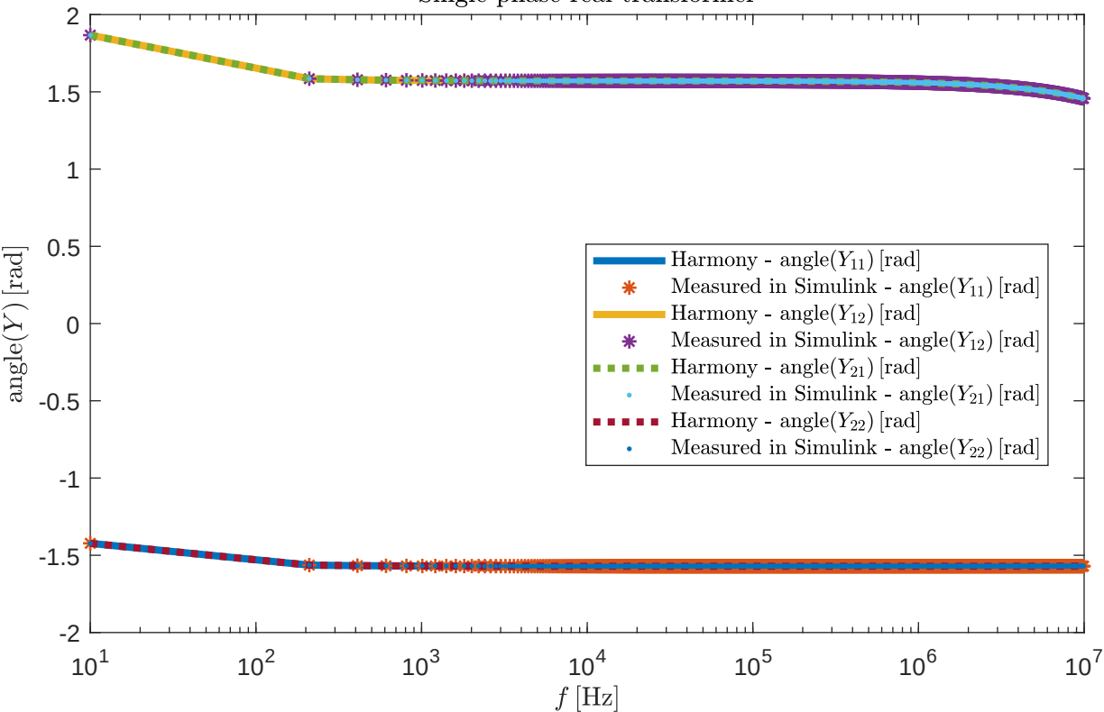
Single-phase real transformer
