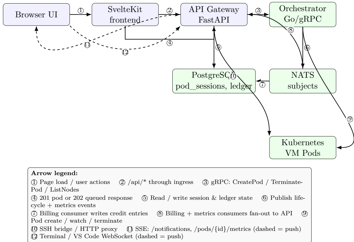
Figure 2: Main request and data flow for VM creation, monitoring, and interactive access.
