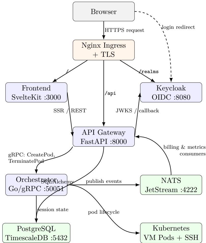
Figure 1: Verified high-level Hopper architecture derived from the frontend, gateway, orchestrator, and Kubernetes deployment files.
