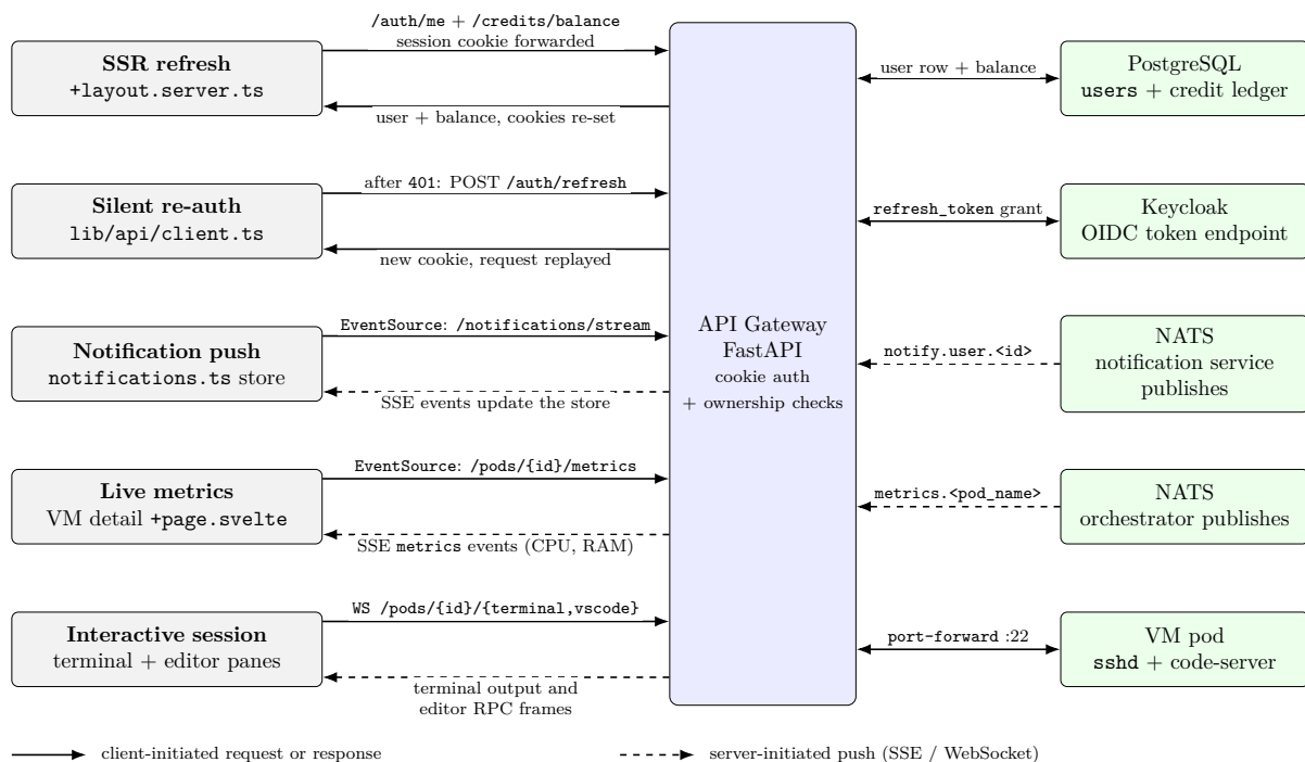
Figure 4: Verified automatic UI data-sync mechanisms: SSR refresh, SSE streams, and WebSocket proxying.
