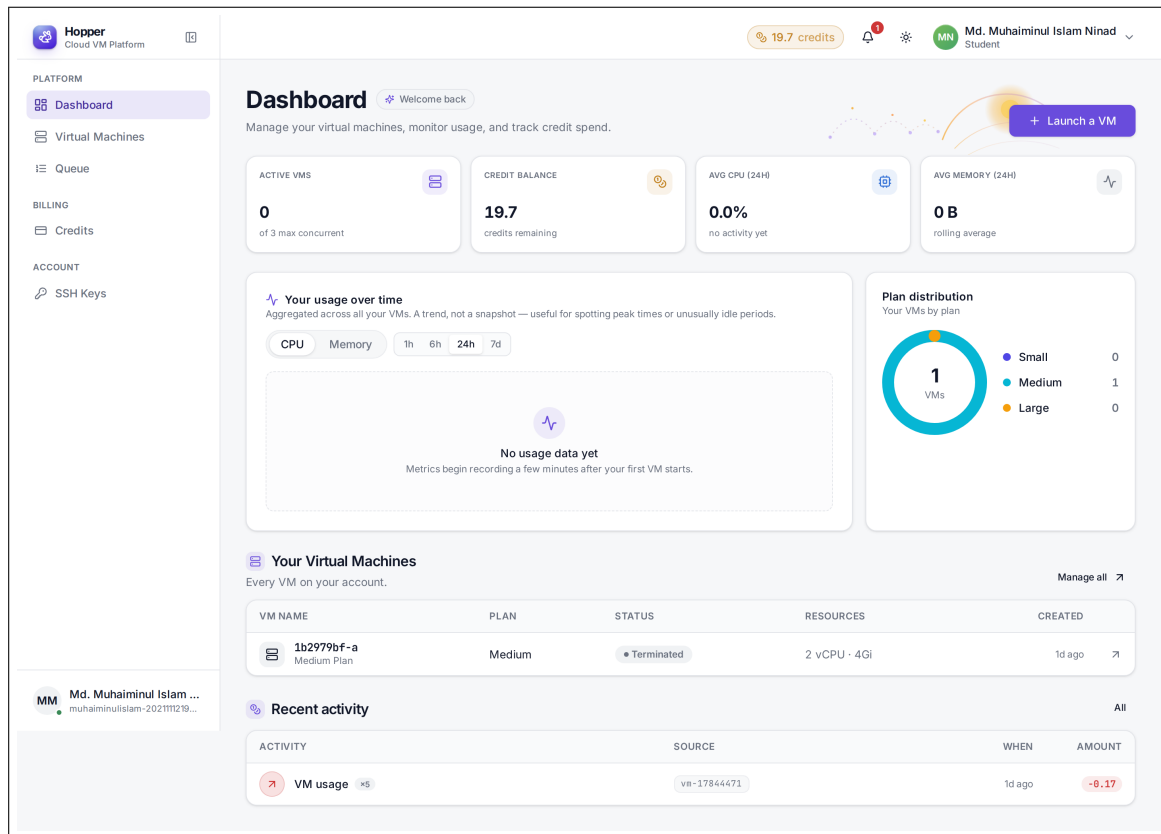
Figure 10: Screen 3: Student Dashboard (/dashboard) — Stat cards for active VMs, credit balance, and 24-hour average CPU and memory. “Your usage over time” chart with CPU/Memory and 1h/6h/24h/7d selectors, plan-distribution donut, the user’s VM table, and recent credit activity.
