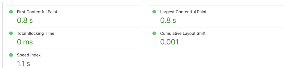
Figure 9: Core Web Vitals and supporting metric measurements from the same desktop audit.
