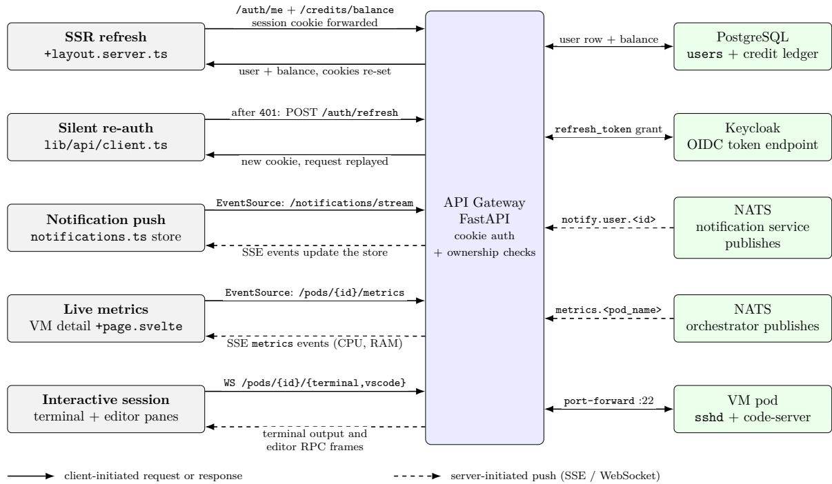
Figure 7: Verified automatic UI data-sync mechanisms: SSR refresh, SSE streams, and WebSocket proxying.
