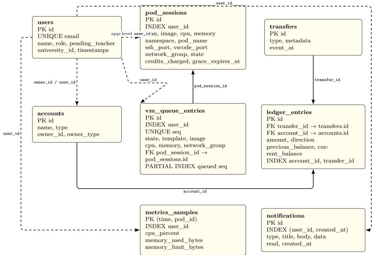
Figure 6: Core entity relationships derived from SQLAlchemy models and Alembic migrations. Solid arrows indicate database-enforced foreign keys; dashed arrows indicate application-level links stored by identifier only.
