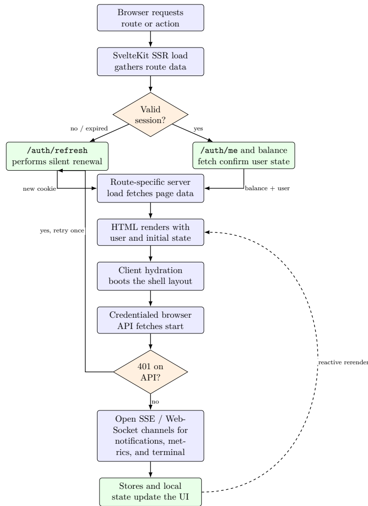
Figure 4: Frontend architecture flow: SSR authentication, server-side page loading, browser-side retry, and real-time channel setup.
