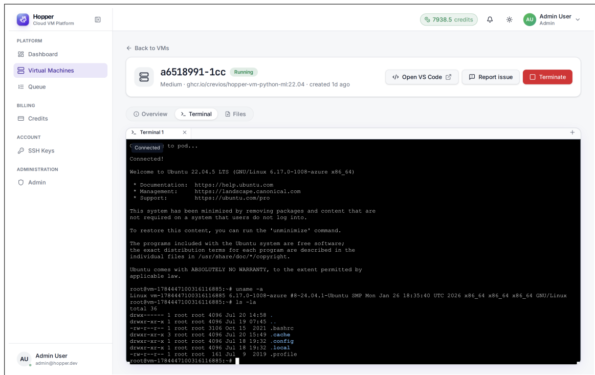
Figure 16: Screen 6: VM Detail — Terminal Tab ( /pods/[id]?tab=terminal ) — Full-height xterm.js terminal attached to the VM over a WebSocket, showing the session tab bar with its Connected status badge and a “new terminal” control. The transcript shows the Ubuntu 22.04.5 login banner followed by uname -a and ls -la executed inside the container, confirming a live interactive shell rather than a rendered mock-up.
