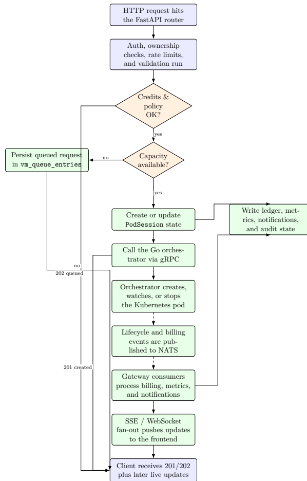
Figure 5: Backend architecture flow: synchronous admission, queued fallback, gRPC orchestration, and asynchronous event fan-out.
