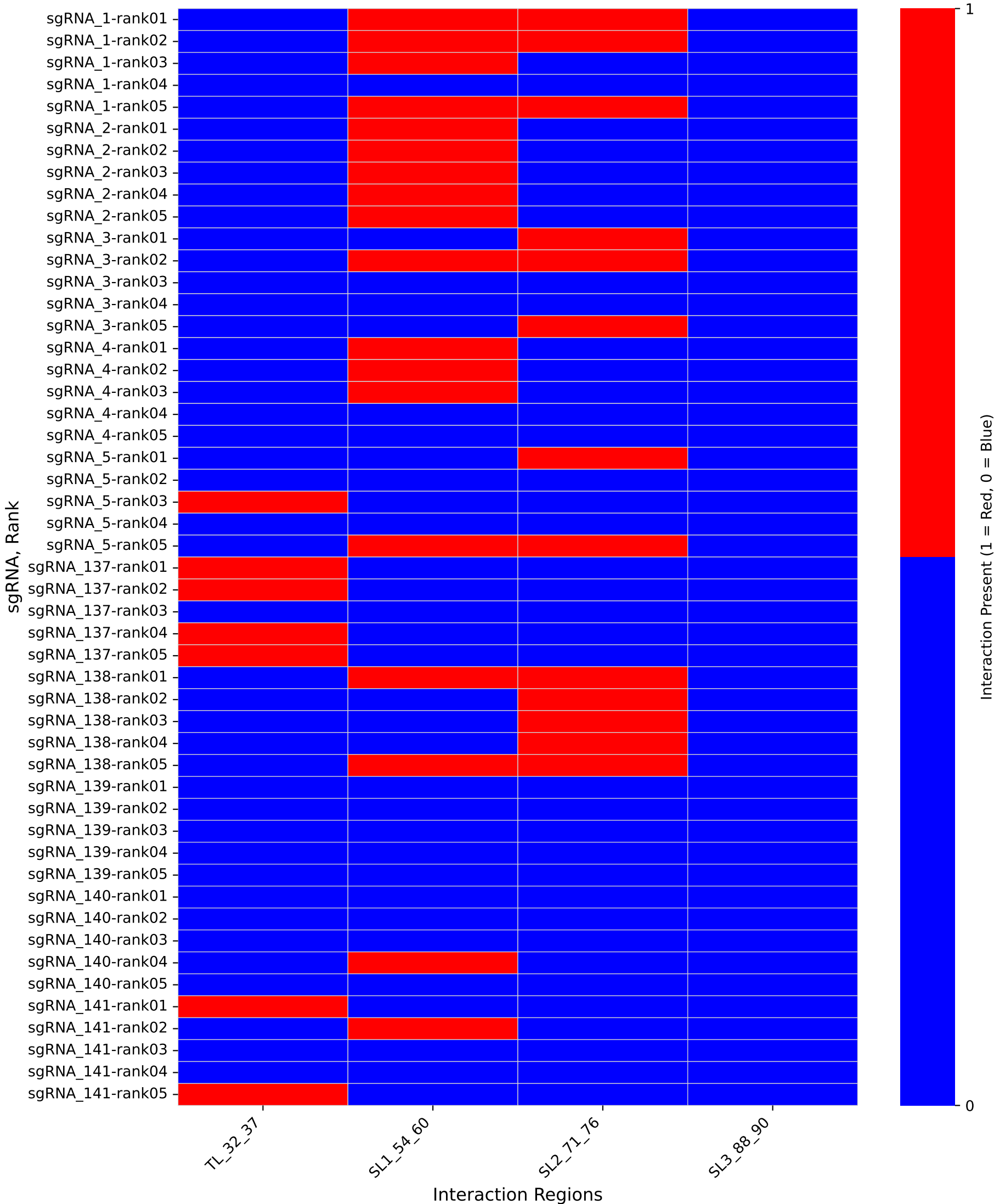
sgRNA Interaction (STACK) Heatmap across Ranks
