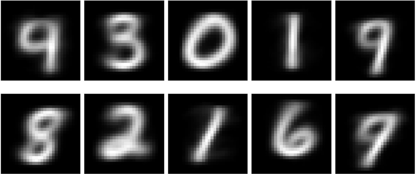
Converged centroids.
