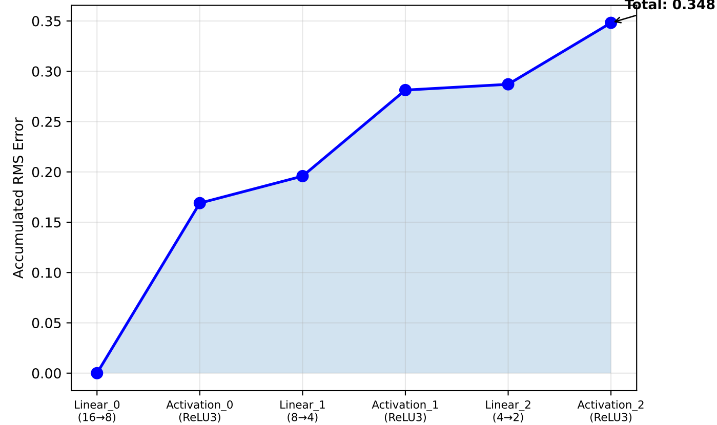
Small FC (16→8→4→2) - Error Accumulation
