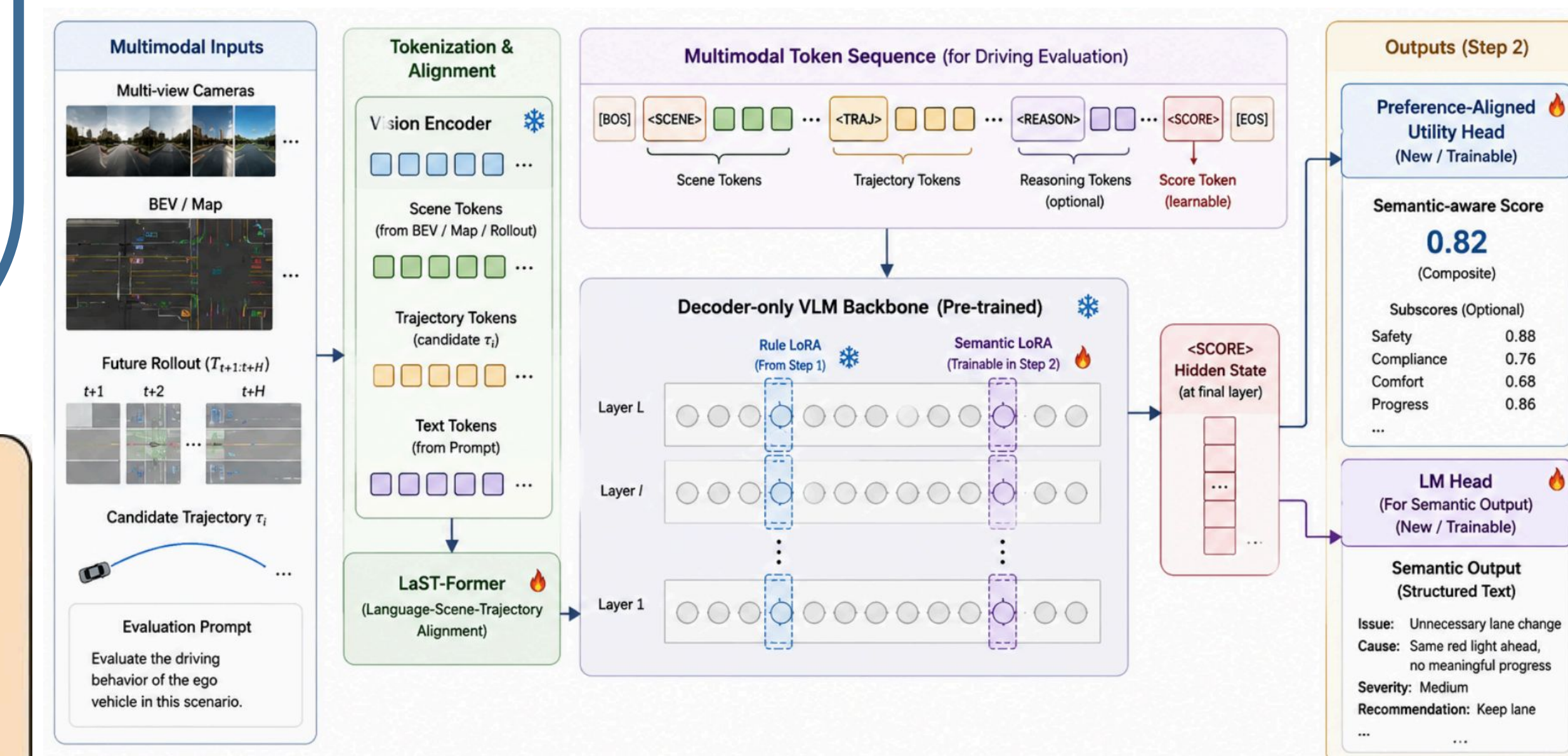
Figure 2. Multi-LoRA Details & Results
