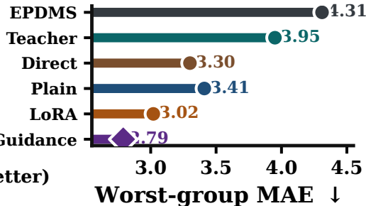
(c) Worst-group robustness
