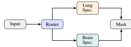
Fig. 1: Anatomy-aware routing architecture. A ConvNeXt-Tiny classifier routes each input to the appropriate specialist UNet++ network.
