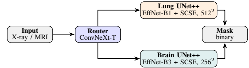
Fig. 1: Anatomy-aware routing architecture. A ConvNeXt-Tiny classifier routes each input to a dedicated UNet++ specialist with SCSE attention and encoder. The mixed baseline S^H shares the lung backbone (UNet++/EffNet-B1, 256^2 ) but uses no attention and is trained jointly on both organs.
