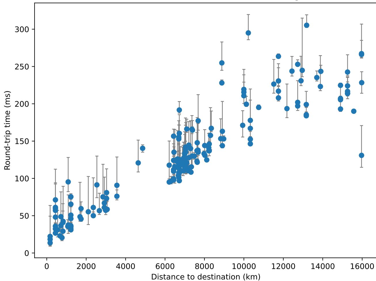
Distance vs. RTT (bars show min-max range)
