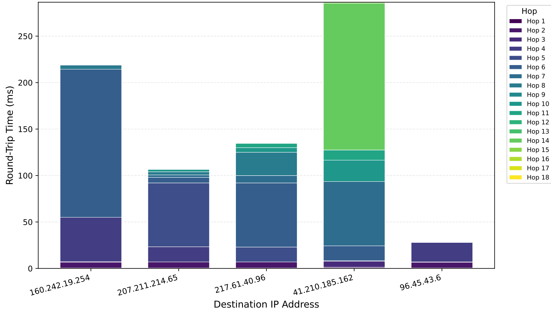
Breakdown of Latencies to Each Hop by Destination
