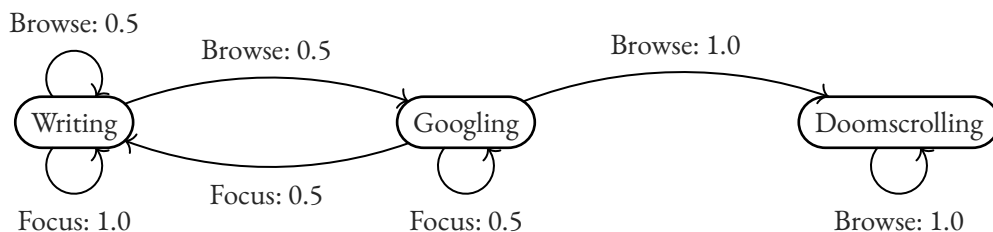
Figure 2: State Transition Diagram with Transition Probabilities
