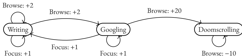
Figure 3: State Transition Diagram with Rewards
