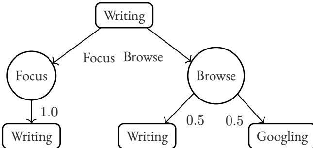
Figure 5: Expectimax trees for Writing. Square nodes are agent (max) nodes, circle nodes are Q-states where the environment resolves the outcome.
