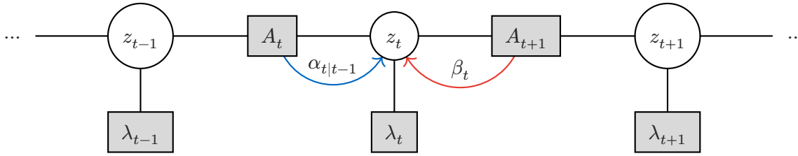
Figure 15: The HMM as a factor graph. Square nodes are the transition factors A_t(z_{t-1}, z_t) = A_{z_{t-1}z_t} and the local evidence factors \lambda_t . Sum-product messages into z_t from the left and right transition factors are exactly the forwards prediction \alpha_{t|t-1} and the backwards message \beta_t .
