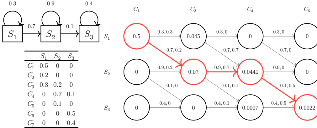
Figure 8: Viterbi decoding in a three-state HMM for a single phone. Left: the state transition diagram and the emission probabilities of each symbol C_1, \dots, C_7 . Right: the trellis for observations (C_1, C_3, C_4, C_6) . Each node shows \delta_t(j) and each edge is labeled (transition probability, emission probability). The red path is recovered by traceback. After textbook Figure 9.6, adapted from Russell and Norvig.
