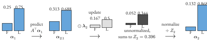
Figure 5: One step of the forwards algorithm on the casino, after two sixes in a row from a uniform start. Predict pushes yesterday's belief through A ; update multiplies by the local evidence of a six, \lambda = [1/6, 1/2] (gray inset); normalizing divides by Z_2 = p(y_2 | y_1) .
