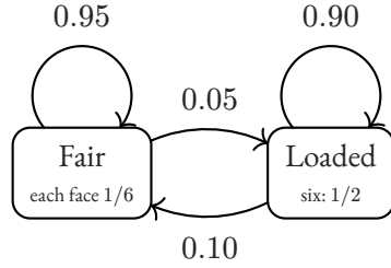
Figure 3: Casino HMM state transition diagram. After textbook Figure 9.2, adapted from Durbin et al. 1998, p. 54.
