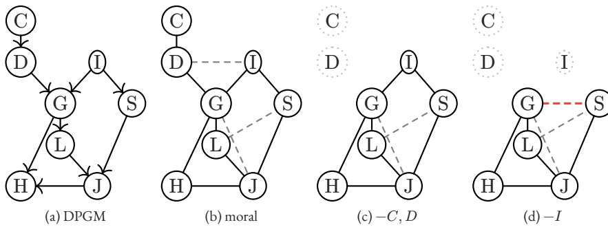
Figure 11: Symbolic variable elimination on the student network (Coherence, Difficulty, Intelligence, Grade, SAT, Letter, Job, Happy). (a) The DPGM. (b) Its moralization; gray dashed edges join co-parents. (c) Eliminating C then D adds no edges. (d) Eliminating I joins its remaining neighbors G and S with a fill-in edge (red). After textbook Figure 9.18, adapted from Koller and Friedman Figure 9.10.
