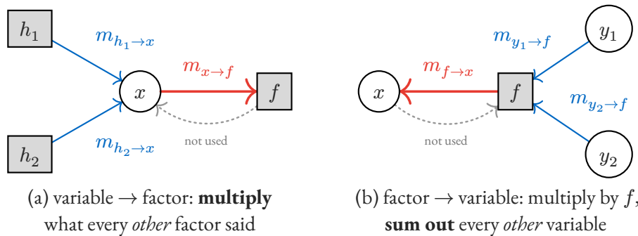
Figure 12: The two sum-product rules. Both rules exclude the recipient's own message (dashed): a node never echoes information back to where it came from.
