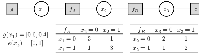
Figure 9: The running example for the rest of the section: a binary chain x_1 - x_2 - x_3 as a factor graph, with a prior factor g on x_1 , pairwise factors f_A, f_B that prefer agreement, and an indicator factor e entering the evidence x_3 = 1 .
