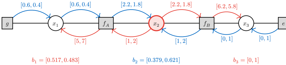
Figure 13: Sum-product on the running example, rooted at x_2 . Blue messages collect toward x_2 ; red messages distribute back out. Each reply excludes the message received on that edge.
