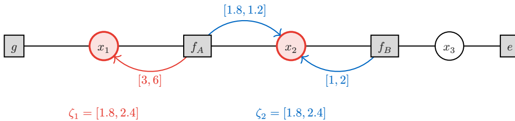
Figure 16: Max-product on the running example. Each max-marginal peaks at 2.4 and points to the MAP assignment (x_1, x_2) = (1, 1) .
