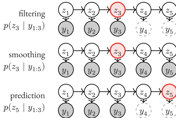
Figure 4: Which evidence each query uses, for T = 5 . The queried state is outlined in red; shaded observations are conditioned on, dashed ones are not.
