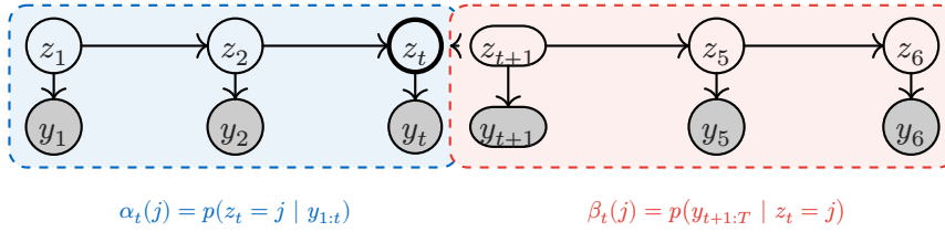
Figure 7: Smoothing splits the evidence at z_t . The forwards message \alpha_t summarizes everything to the left, including y_t ; the backwards message \beta_t summarizes everything to the right. Because z_t d-separates the two regions, the smoothed marginal is their normalized product.
