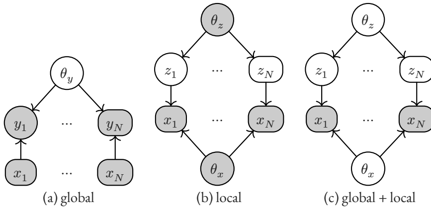
Figure 1: Three common inference patterns. (a) Global hidden variables, the Bayesian discriminative model p(y_{1:N}, \theta_y | x_{1:N}) = p(\theta_y) \prod_n p(y_n | x_n; \theta_y) . (b) Local hidden variables with known parameters, p(x_{1:N}, z_{1:N} | \theta) = \prod_n p(z_n | \theta_z) p(x_n | z_n, \theta_x) . (c) Local and global hidden variables, p(x_{1:N}, z_{1:N}, \theta) = p(\theta_z) p(\theta_x) \prod_n p(z_n | \theta_z) p(x_n | z_n, \theta_x) . Shaded nodes are observed. After textbook Figure 7.1.
