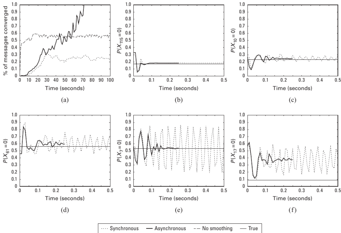
Figure 18: Loopy BP on an 11 \times 11 Ising grid with random couplings w_{ij} \sim \text{Unif}(-C, C) , C = 11 . (a) Fraction of messages converged over time for damped synchronous (dotted), undamped asynchronous (dashed), and damped asynchronous (solid) schedules. (b–f) Marginal beliefs of individual nodes over time against the true marginal (straight line). Reproduced from Murphy, Textbook Figure 9.13, p. 422, originally Koller and Friedman Figure 11.C.1 (CC BY-NC-ND).
