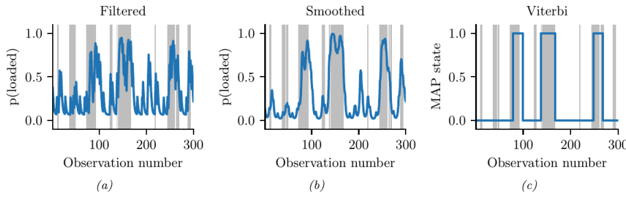
Figure 6: Inference in the dishonest casino over T = 300 rolls. Gray bars mark the times the loaded die was actually in use; blue lines show the posterior probability of the loaded state. (a) Filtered, p(z_t \mid y_{1:t}) . (b) Smoothed, p(z_t \mid y_{1:T}) . (c) The Viterbi (MAP) trajectory. Reproduced from Murphy, Textbook Figure 9.3, p. 404 (CC BY-NC-ND).
