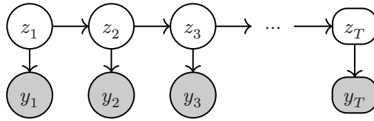
Figure 2: A hidden Markov model as a DPGM. z_t are the hidden states and y_t the observations. After textbook Figure 9.1.
