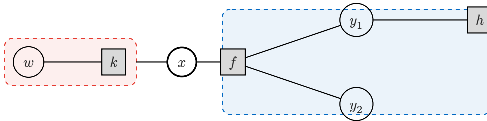
Figure 14: On a tree, the message a factor sends toward x is the sum over the whole subtree behind it (blue region), and different neighbors' subtrees (blue, red) share no variables. Multiplying all messages into x therefore sums the full joint over everything except x .
