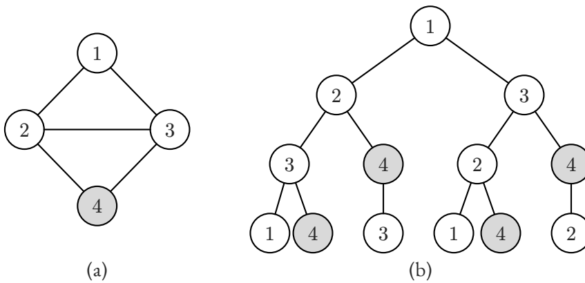
Figure 17: (a) A simple loopy graph. (b) Its computation tree rooted at node 1 after three rounds of message passing. Evidence at node 4 (shaded) reaches node 1 along two different branches, and the original variables recur in several places. After textbook Figure 9.12, from Wainwright and Jordan 2008.
