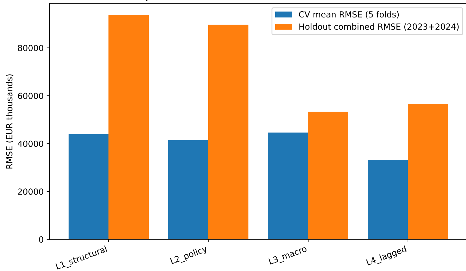
4-layer ablation lift: CV mean vs 2023+2024 holdout
