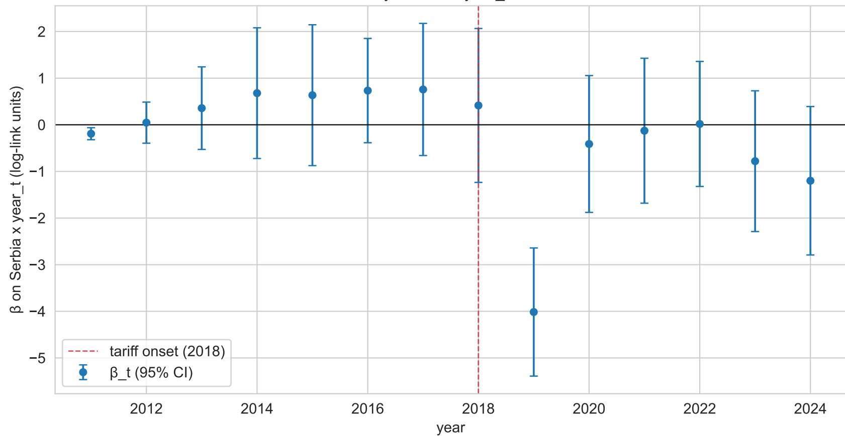
Event study: Serbia x year_t coefficients
