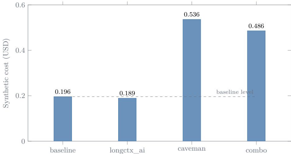
Total synthetic cost by configuration (66 problems each)
