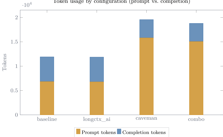
Token usage by configuration (prompt vs. completion)
