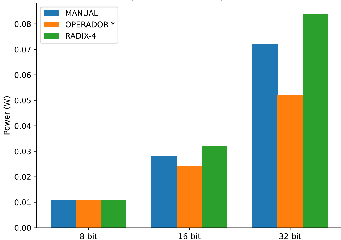
Dynamic Power Comparison
