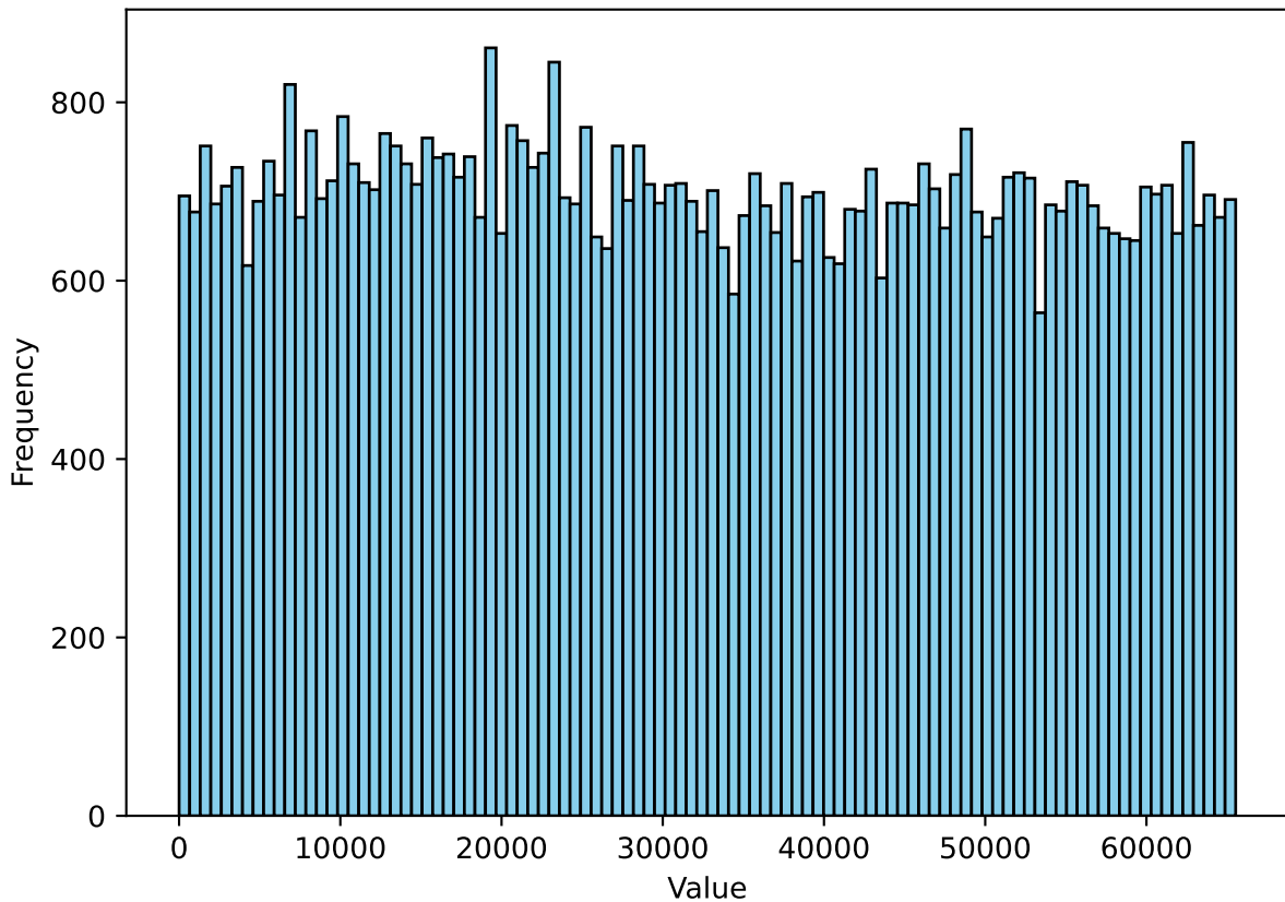
Uniform Distribution (16-bit)
