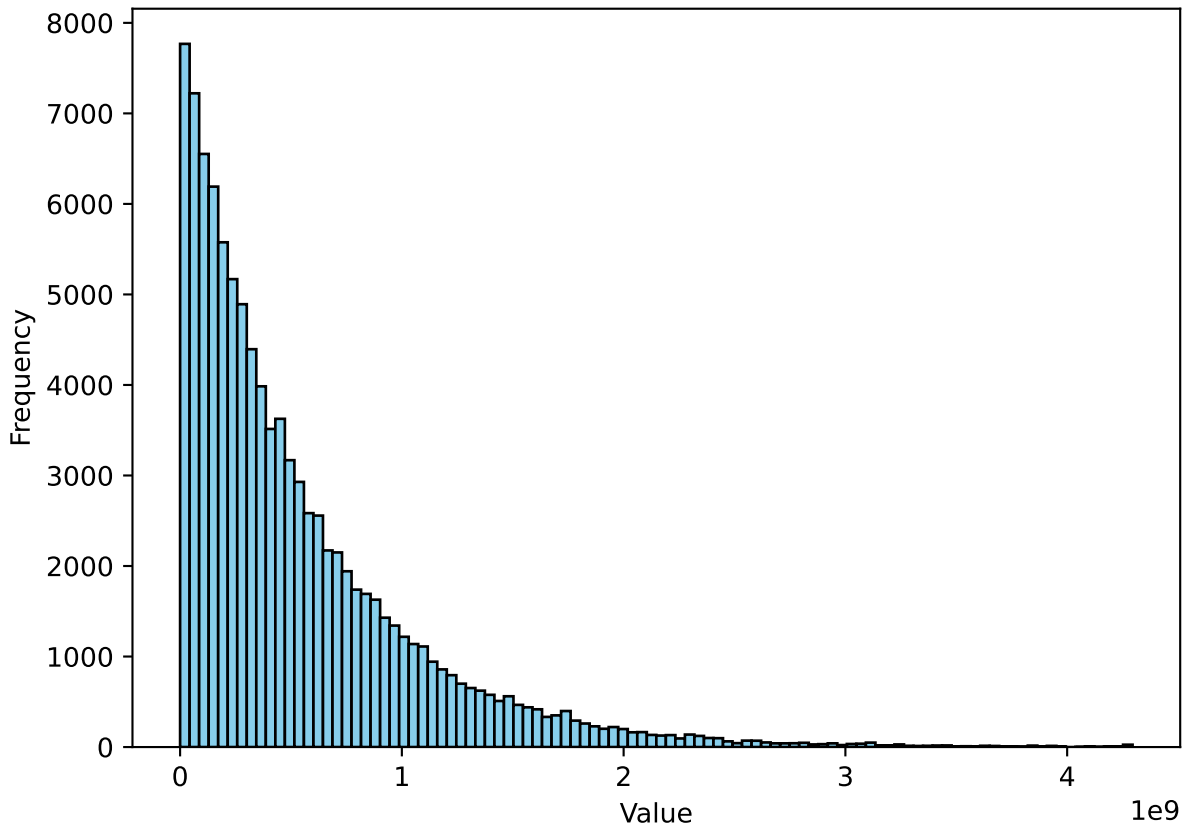
Exponential Distribution (32-bit)
