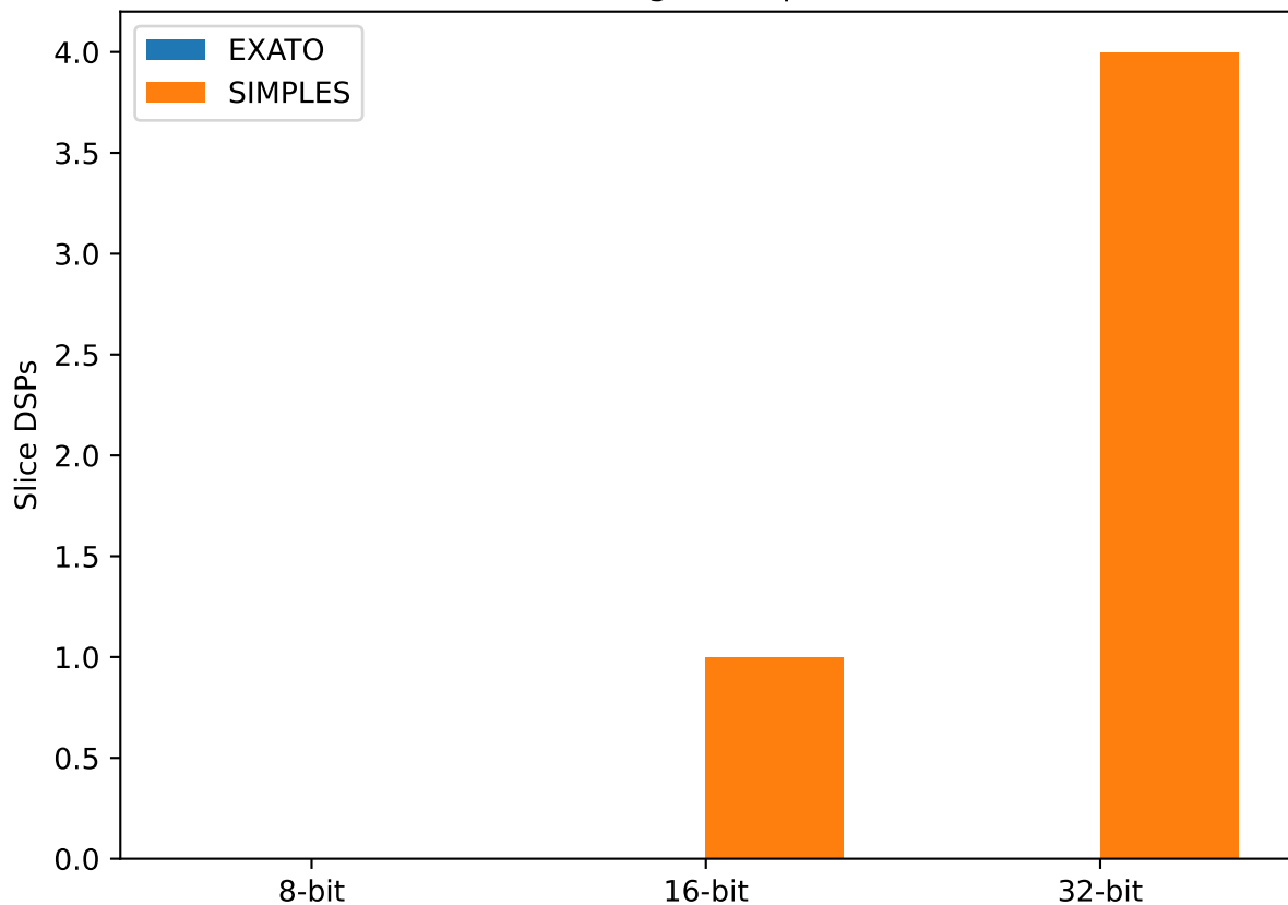
DSP Usage Comparison
