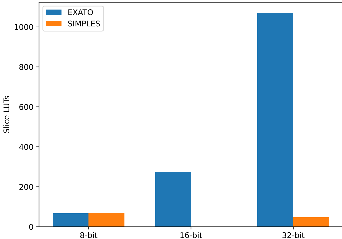
LUT Usage Comparison
