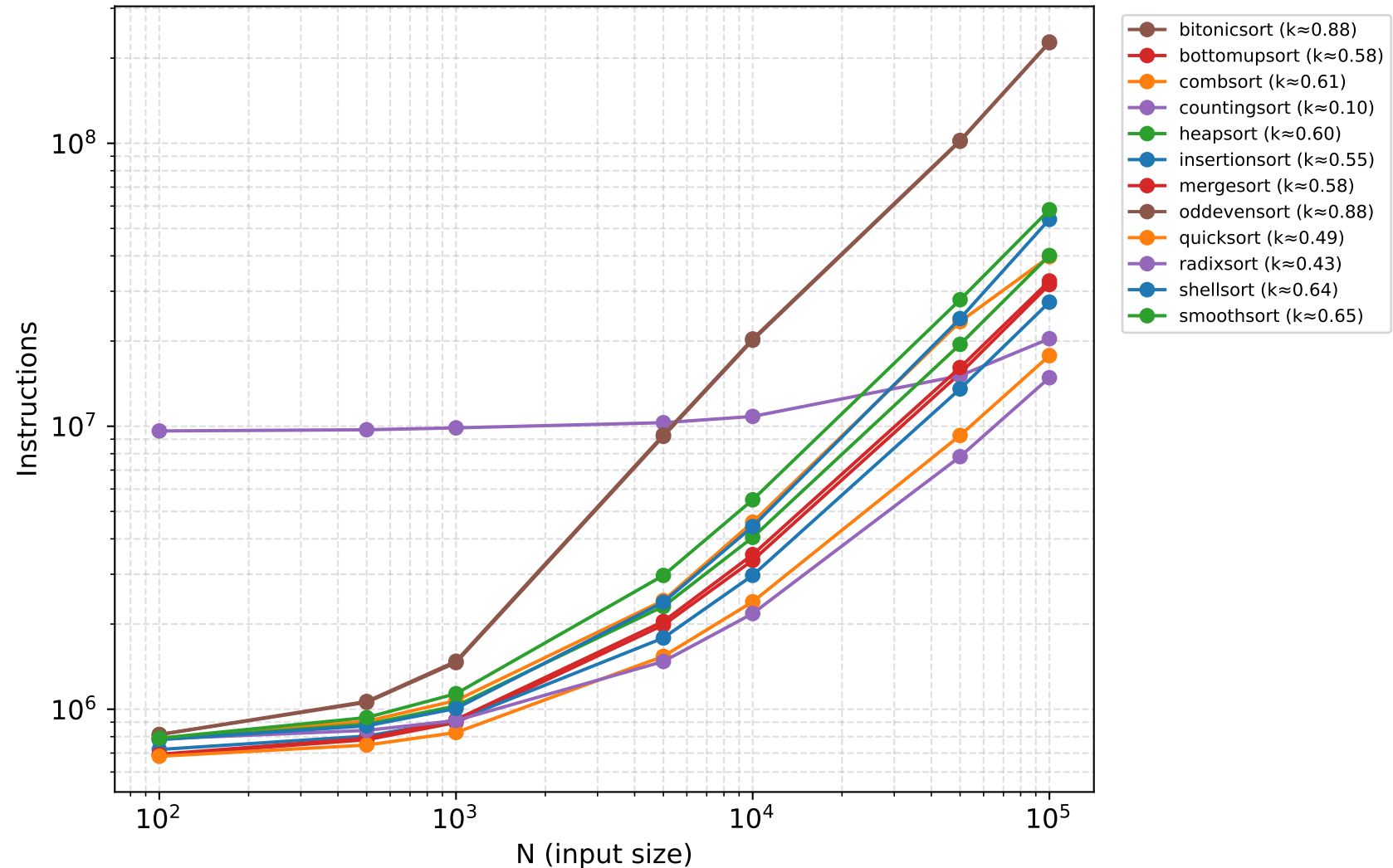
Empirical complexity — Instructions vs N (log-log, serial t1)
