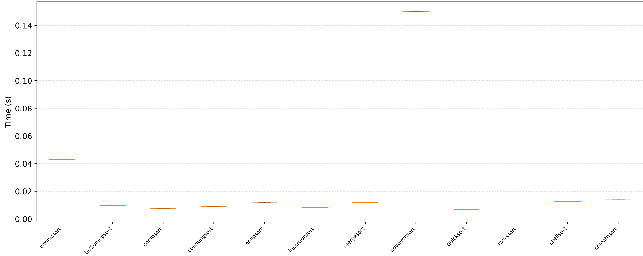
Distribution over repetitions (N=100000, serial)
