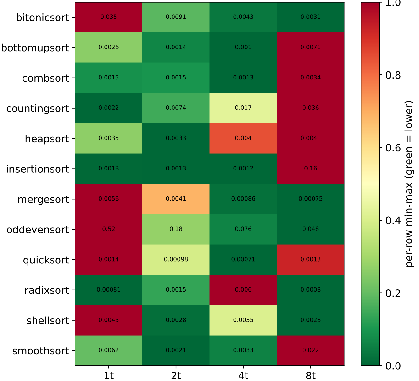
EDP (J·s) by algorithm × threads (N=100000) — green = best per row
