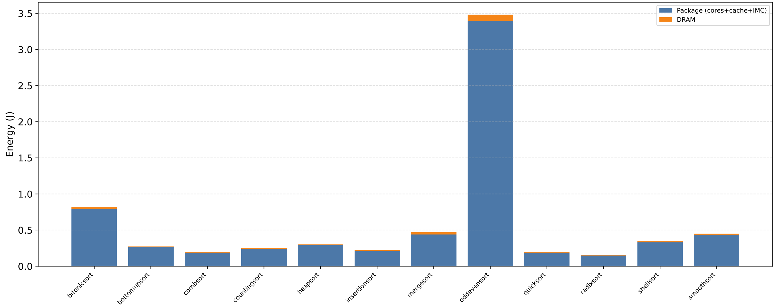
Energy breakdown: package vs DRAM (N=100000, serial)
