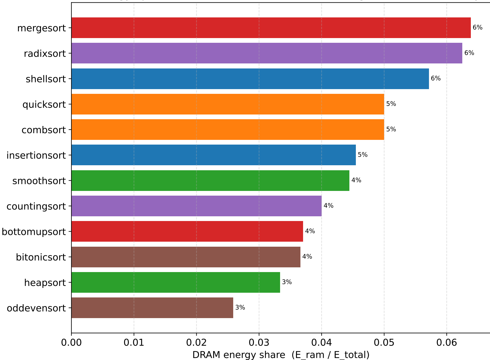
Share of energy spent in DRAM (N=100000, serial) — higher = more memory-bound
