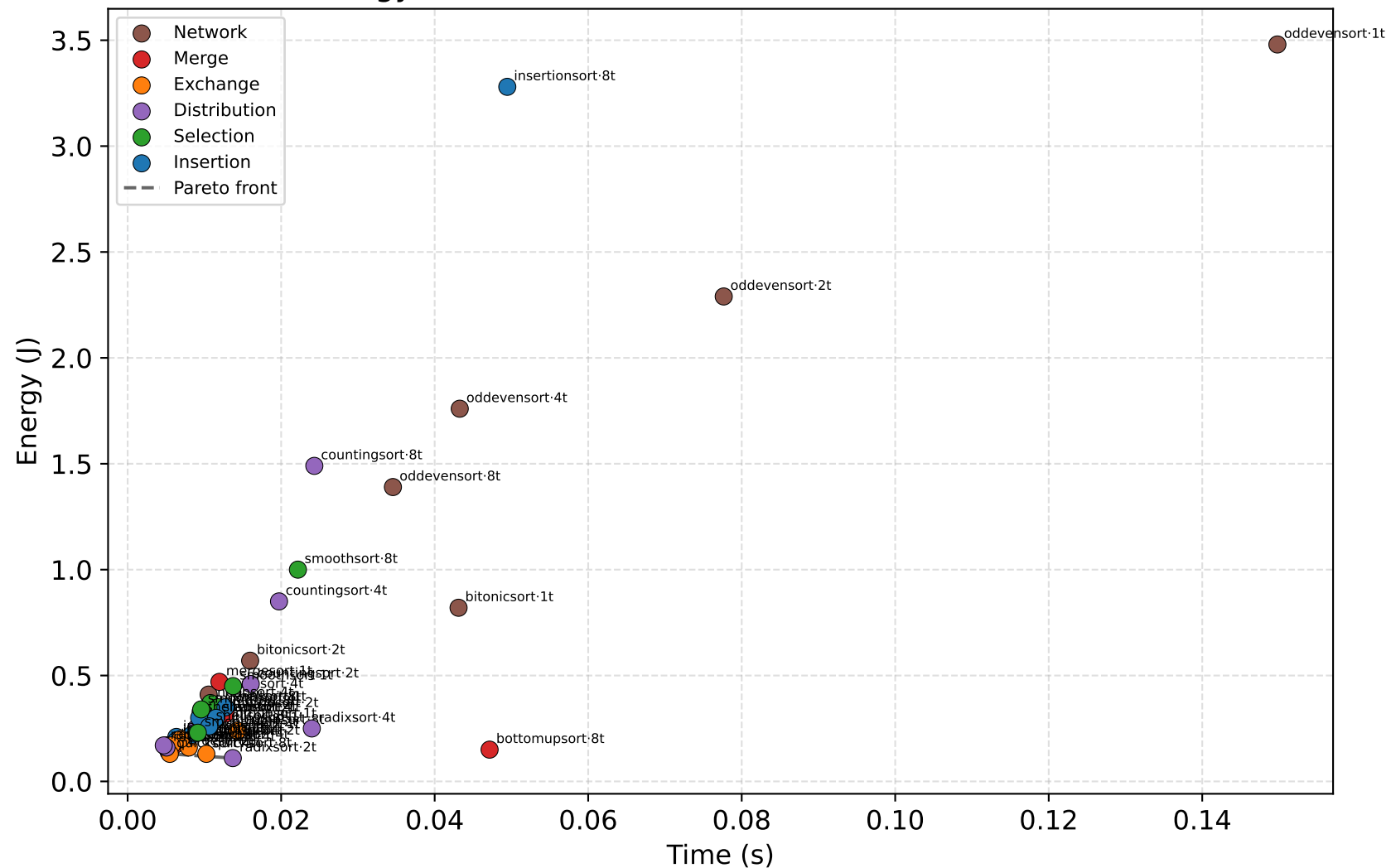
Energy-time trade-off (N=100000, all thread counts)
