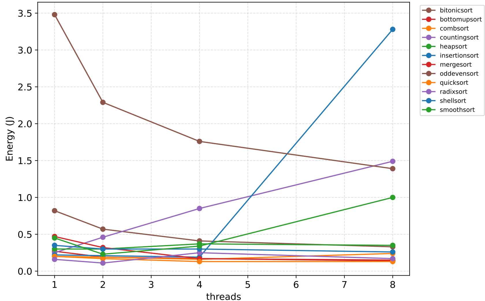
Total energy vs threads (N=100000) — does not drop like time
