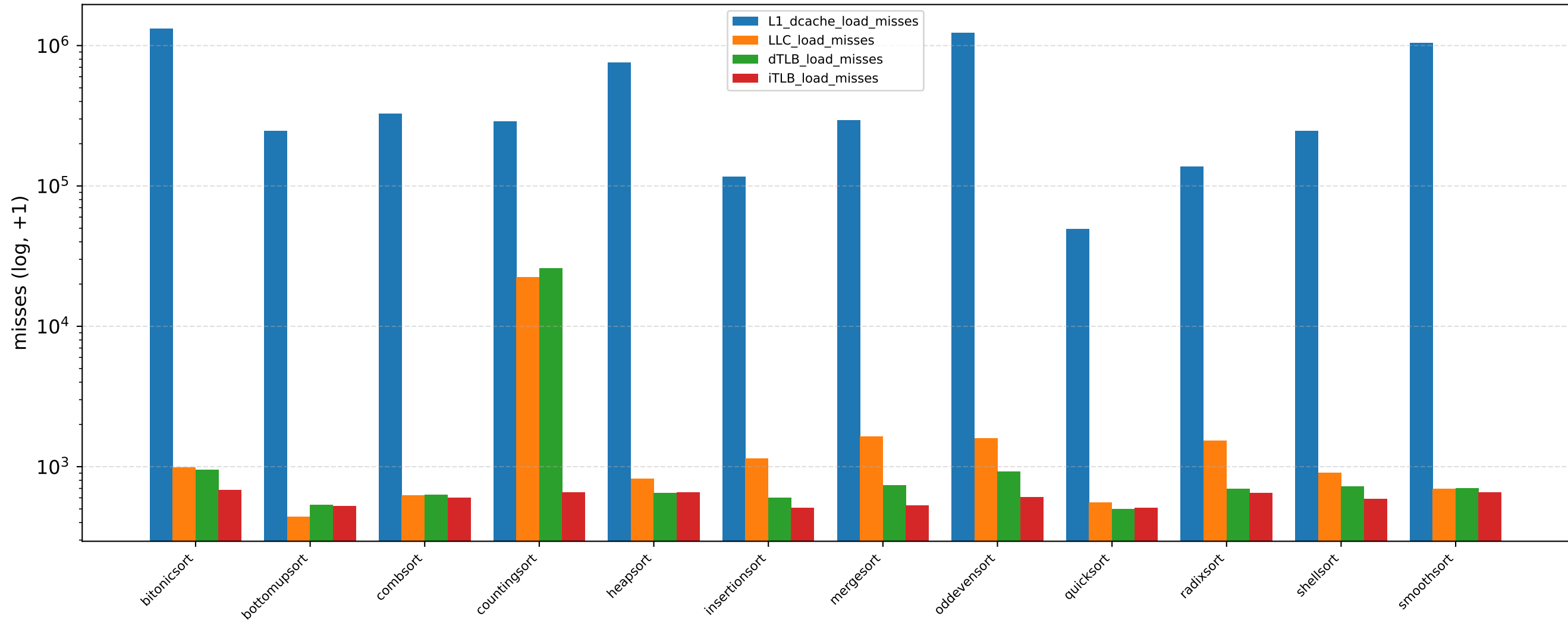
Memory hierarchy pressure (N=100000, serial)
