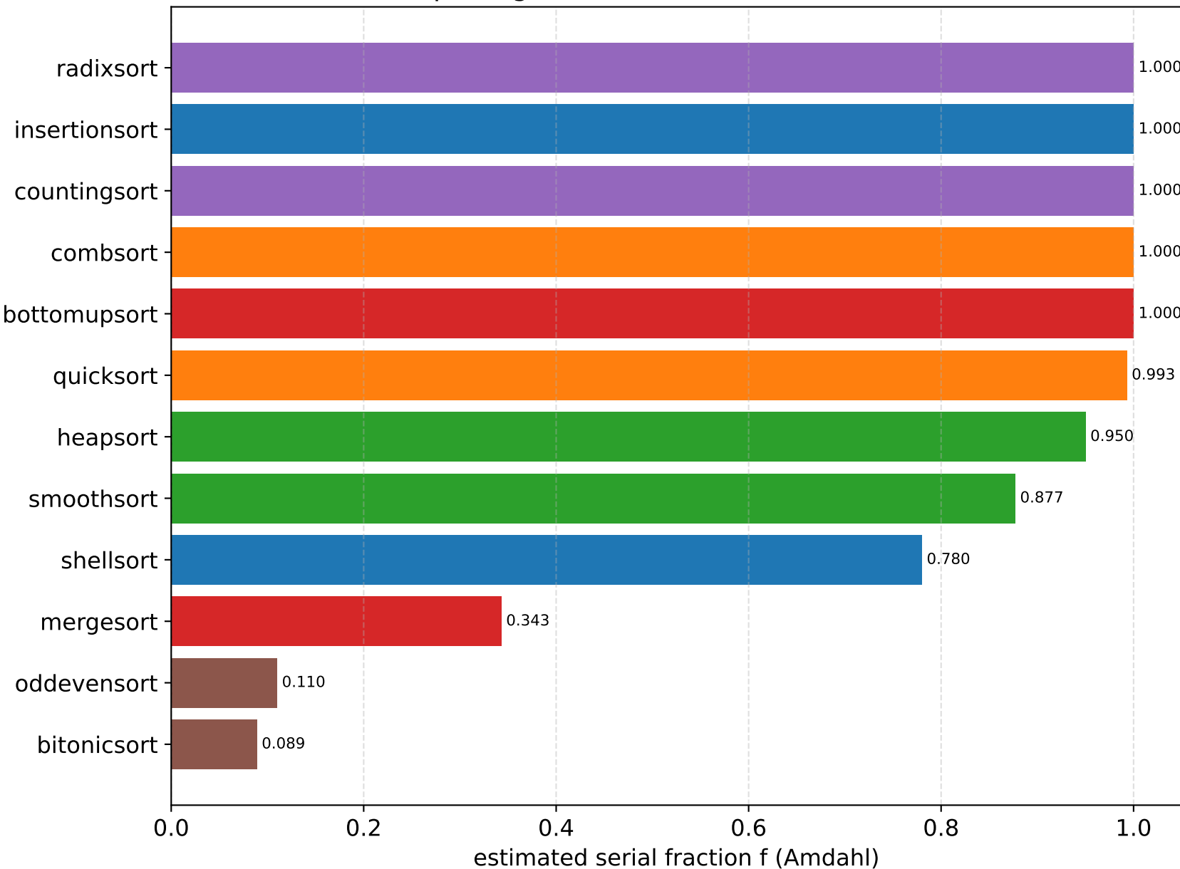
Serial fraction per algorithm (N=100000) — lower f scales better
